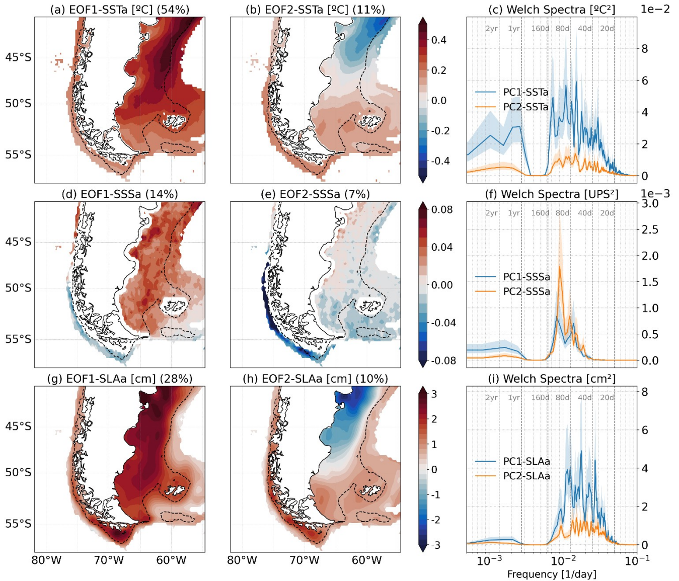
Figure 4: EOF analysis results for SSTa, SSSa, and SLAa. Panels a and b show the first and second EOF modes of SSTa, panels d and e show EOF1 and EOF2 of SSSa, and panels g and h show EOF1 and EOF2 of SLAa. Panels c, f, and i display the power spectra of the corresponding PC time series for SSTa, SSSa, and SLAa, respectively, estimated using Welch's method. In the spectral plots, blue and orange curves correspond to the spectra of the first and second PCs. Spectra are shown in a variance-preserving form to emphasize the relative contribution of different frequency bands. Contour intervals are 0.05^{\circ}\text{C} for SSTa, 0.01 salinity units for SSSa, and 0.2 cm for SLAa. BlackGray dashed lines in the EOF maps indicate the 200 m isobath.
