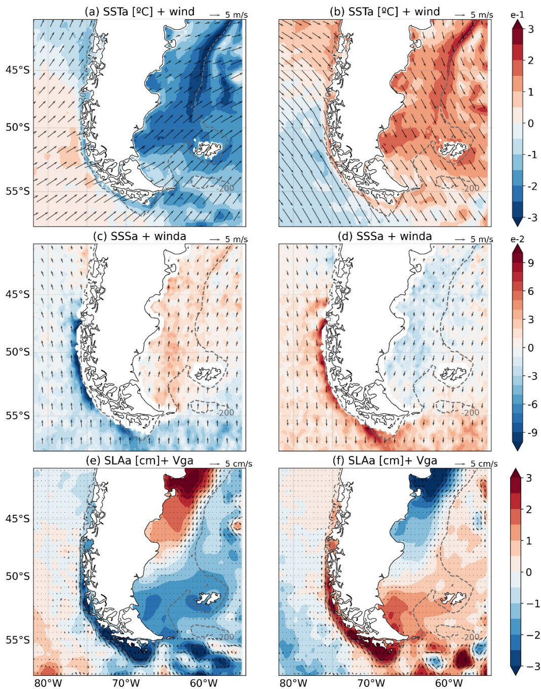
520 | Figure 6: Composites for the positive (southerly winds) and negative (northerly winds) phases of the leading mode of the meridional wind. Panels a, c, and e show SST, SSS, and SLA anomalies for the positive phase, while panels b, d, and f show these anomalies for the negative phase. Black arrows represent wind composites in panels a and b, wind anomalies in panels c and d, and geostrophic velocity anomalies in panels e and f. Gray dashed lines indicate the 200 m isobath.
