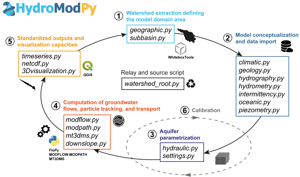
Figure 1. Workflow of HydroModPy, illustrating the organization and interconnection of Python scripts within the toolbox across six five BB main stages: (1) watershed extraction defining the model domain area from digital elevation models and outlet coordinates, (2) model conceptualization and data import, including climatic forcing, hydrographic networks, and observational datasets for calibration, (3) aquifer parametrization, specifying hydraulic properties, geometry, and boundary conditions, (4) computation of groundwater flows using MODFLOW-NWT via FloPy, with optional particle tracking (MODPATH) and transport simulations (MT3DMS), and AG (5) standardized outputs and visualization, exporting results in geospatial formats (GeoTIFF, shapefile, n NetCDF , VTK) and providing 2D/3D visualization tools for interactive exploration and analysis, and (6) comparison of outputs and data for calibration. AG
