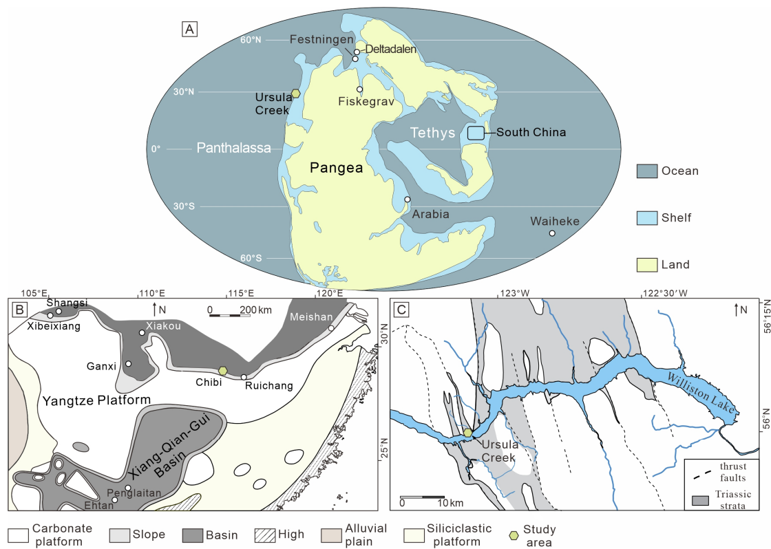
Figure 1. (A) Palaeogeographic reconstruction of Pangaea in the Late Permian (modified from Scotese, 2014). (B) Palaeogeographic reconstruction of the South China Block Craton during the Changhsingian (modified from Feng et al., 1996). (C) Locations of the Ursula Creek section- (modified from Wignall
