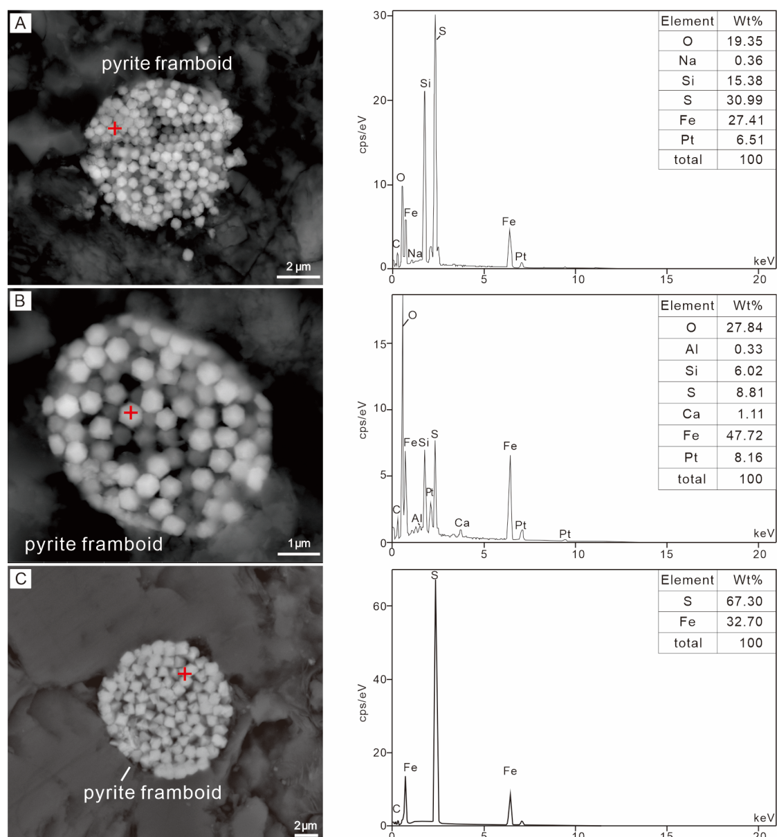
Figure 4. Mineral composition of pyrite framboids in samples from the Ursula Creek and Chibi sections. (A) SEM image and EDS spectrum at the red cross of a pyrite framboid from the lower Fantasque Formation, Ursula Creek; (B) SEM image and EDS spectrum at the red cross of a pyrite framboid from the lower Grayling Formation, Ursula Creek; and (C) SEM image and EDS spectrum at the red cross of a pyrite framboid from the lower Talung Formation, Chibi.
