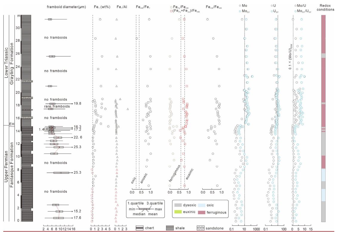
Figure 2. Stratigraphic log of the Ursula Creek section with total iron (Fe T ), Fe T /Al, iron proxies
