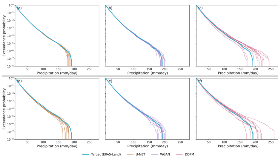
Figure 7. Exceedance probability (1-CDF) curves of daily precipitation for observations and model predictions at 8× (top row) and 16× (bottom row) spatial downscaling. Panels show results for (a, d) U-NET, (b, e) WGAN, and (c, f) DDPM. The observed precipitation is shown by the thick blue curve, while thin colored curves represent 10 ensemble members for each generative model. All curves are computed using the same test samples and plotted on a logarithmic exceedance scale, highlighting differences in the representation of extreme precipitation tails across downscaling approaches and spatial scales.
