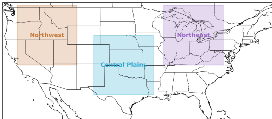
Figure 1. Geographic domains used in this study, showing the three 128 \times 128 grid regions over the contiguous United States representing distinct hydroclimatic regimes: the Pacific Northwest, Central Plains, and Northeast
