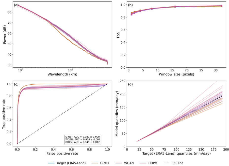
Figure 8. Comparison of U-Net, WGAN, and DDPM performance over the independent Northeast test region at 16× super-resolution. (a) Radial power spectra showing the distribution of spatial variance across wavelengths relative to the target (ERA5-Land) fields. (b) Fractions Skill Score (FSS) as a function of spatial window size. (c) Receiver Operating Characteristic (ROC) curves for wet-pixel classification, with inset values showing the mean \pm standard deviation of the Area Under the Curve (AUC) across ten independent model initializations. (d) Quantile–Quantile (Q–Q) comparison between model and target precipitation quantiles for precipitation amounts exceeding 20 mm/day. Colored lines represent individual model initializations, and the dashed line in (d) denotes perfect agreement (1:1 relationship).
