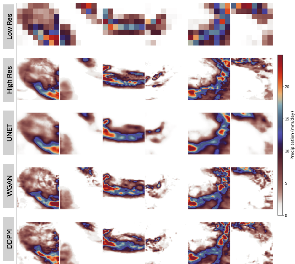
Figure 3. Reconstruction of high-resolution precipitation fields for the 16 \times downscaling task (8 \times 8 \rightarrow 128 \times 128). Columns show six randomly selected test samples, while rows show the low-resolution input, high-resolution target (ERA5-land), and predictions from U-NET, WGAN, and DDPM respectively.
