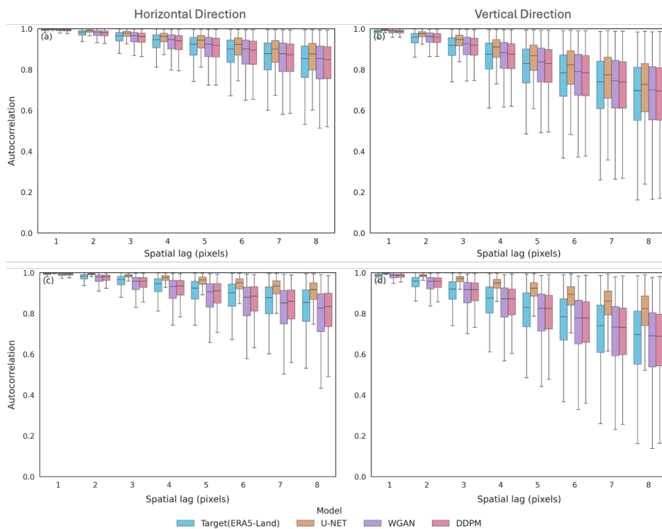
Figure 6. Distributions of horizontal and vertical spatial autocorrelation for lags 1–8 pixels for the ERA5-Land target fields and precipitation fields generated by U-Net, WGAN, and DDPM. Results are aggregated across all test samples and across the 10 independently trained model seeds for each method. Panels (a, b) correspond to the 8× downscaling experiment, while panels (c, d) correspond to the 16× downscaling experiment.
