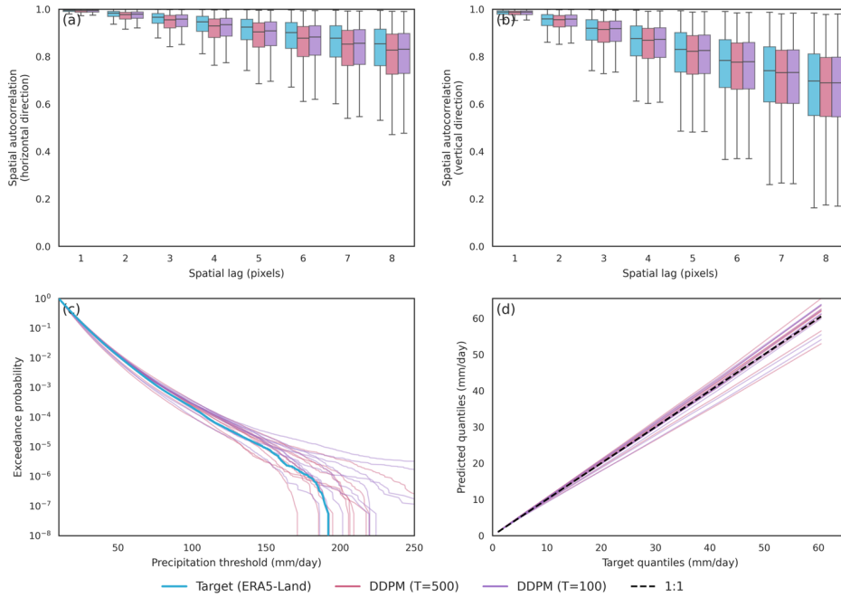
Figure 11. Comparison of DDPM predictions generated using 500 and 100 denoising steps for 16x precipitation downscaling across ten independently trained seeds. Panels show (a) horizontal spatial autocorrelation, (b) vertical spatial autocorrelation, (c) exceedance probability for precipitation intensities exceeding 10 mm/day, and (d) quantile-quantile (Q-Q) relationships relative to Target (ERA5-Land). Boxplots in (a-b) summarize the distribution of spatial correlations across all test samples, while panels (c-d) display individual seed realizations as separate lines. The Target (ERA5-Land) distribution is shown in cyan, DDPM T=500 in pink, and DDPM T=100 in purple. The comparison assesses the sensitivity of spatial dependence and precipitation statistics to the number of diffusion inference steps.
