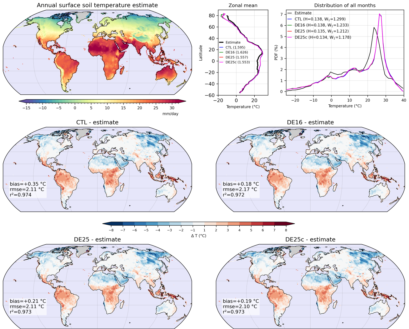
Figure 12. As in Figure 89, but for the comparison between simulated and estimated near-surface soil temperature (°C) at 0–5 cm depth over the 1979–2010 period. The estimate corresponds to the climatological product of Lembrechts et al. (2022) .
