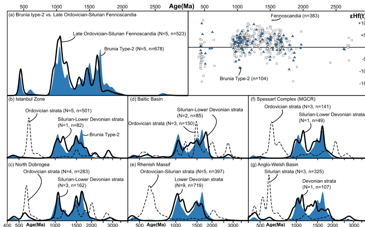
540 Figure 12: Comparison of Brunia Type-2 detrital zircon data with compiled published data from Late Ordovician–Silurian strata 545 of Fennoscandia (a) as well as Late Silurian – Lower Devonian strata from the (b) Istanbul Zone (Akdoğan et al., 2021), (c) North Dobrogea region (Beştepe and Cerna formations in Balintoni and Balica, 2016), (d) Baltic Basin in Estonia (Pöldvere et al., 2014), (e) Rhenish Massif (Eckelmann et al., 2014; Linnemann et al., 2024; Dörr et al., 2025), (f) Spessart Complex in the Mid-German Crystalline Rise (Kirchner and Albert, 2021), and (g) Anglo-Welsh Basin (Waldron et al., 2025). Data used in the construction of this figure is compiled in Collett (2025).
