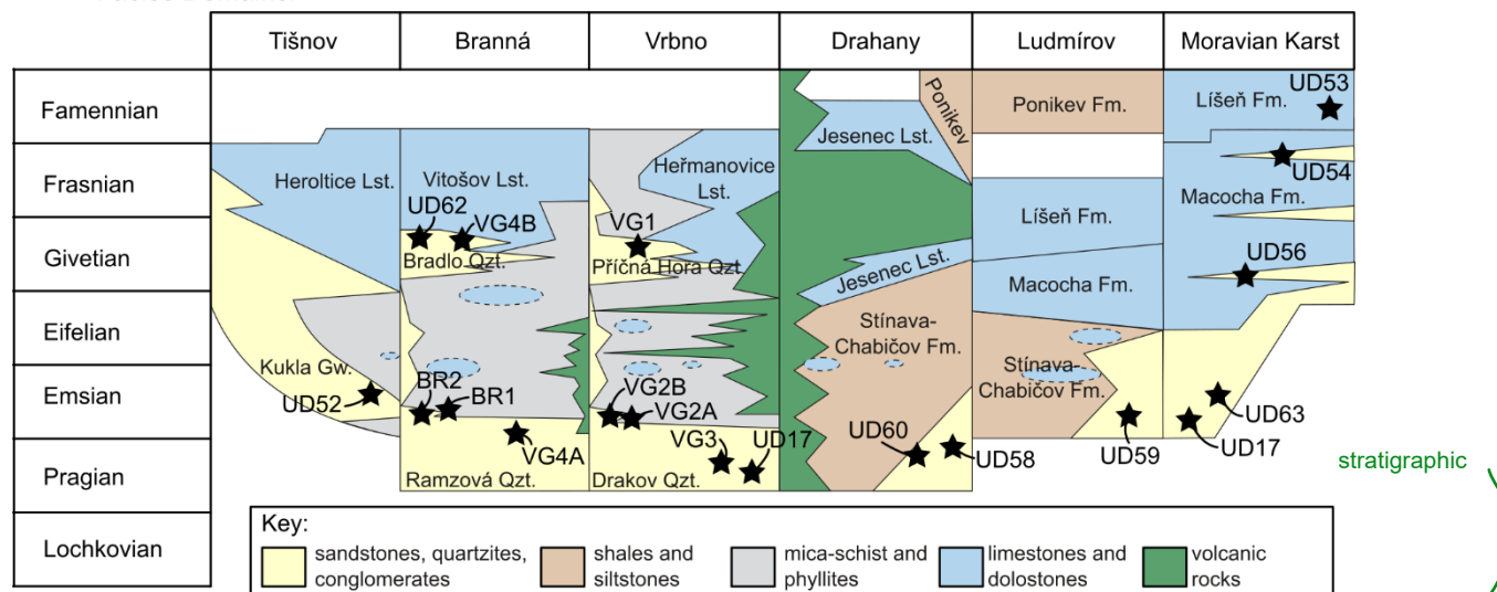
Figure 2: Lithostratigraphic chart of the Devonian facies domains of Brunia with approximate position of the studied samples marked by black stars. Modified from Kalvoda et al. (2025).
