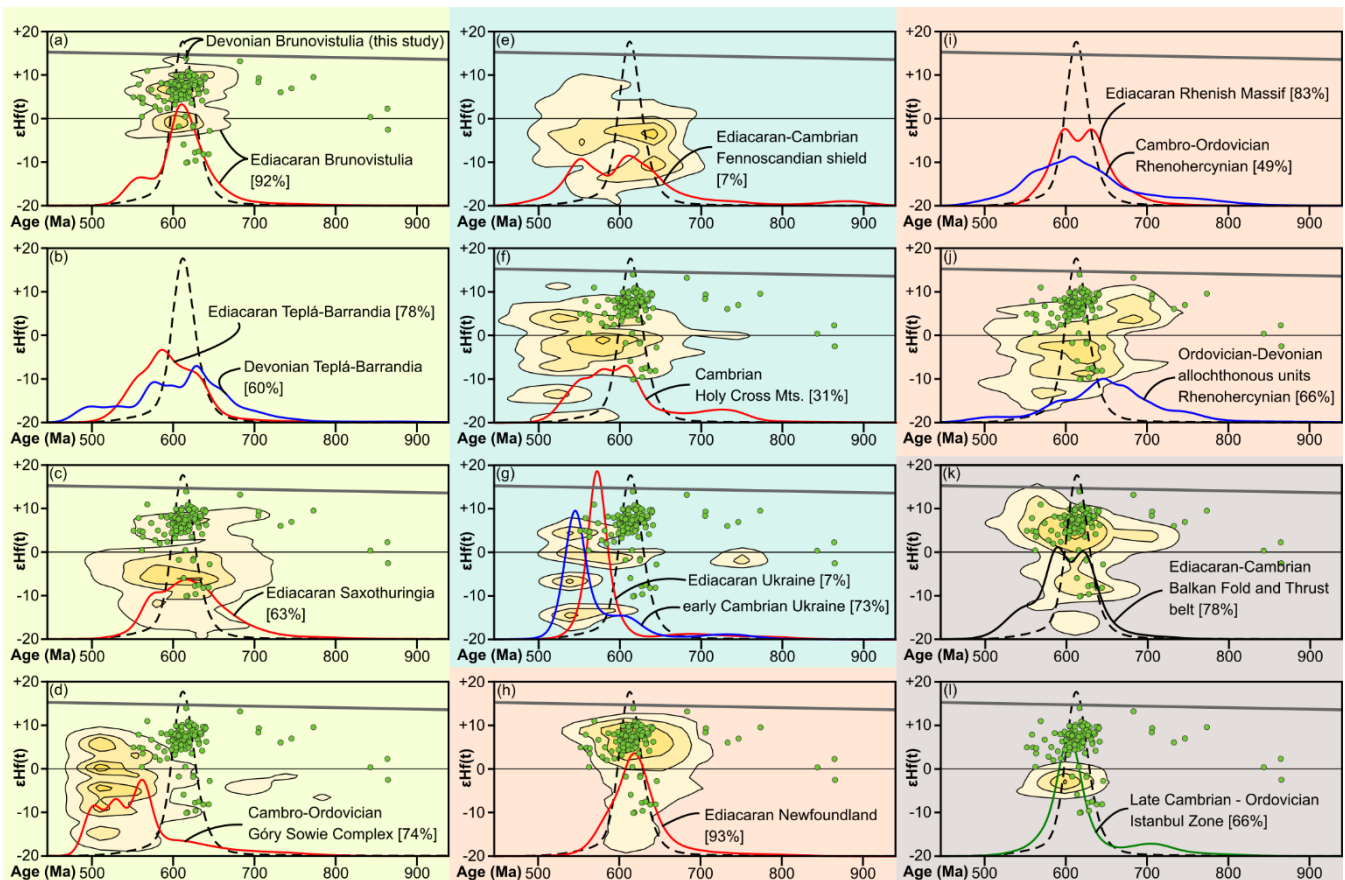
390 Figure 9: Compiled U–Pb and Lu–Hf isotopic data from Neoproterozoic–early Paleozoic zircons in the Bohemian Massif (a–d), SW marginal Baltica (e–g) and Avalonian (h–j) and Far-East Avalonia (k,l) Ediacaran – Devonian strata. Number in parentheses equals the percentage of all concordant zircon analyses in the range 900–485 Ma. Compiled data used to construct this figure are from the detrital zircon database in Collett (2025), a full list of data sources is provided in Section S3.
