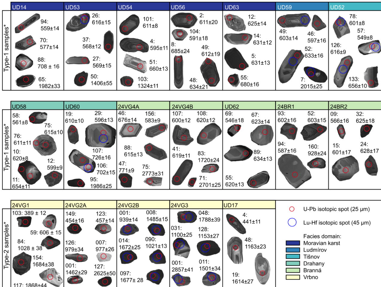
Figure 4: Cathodoluminescence images of representative zircons from each sample. All zircons in the figure gave concordant (concordia distance <5) ages and the given age is the iterative single-grain concordia age with 2s uncertainty. *classification into Type-1 and Type-2 samples according to results section.
