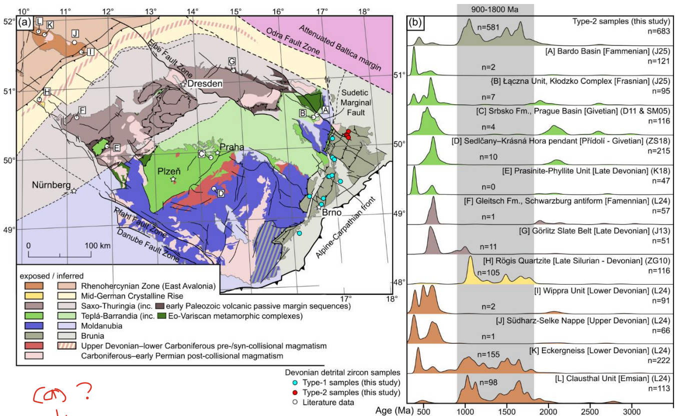
Figure 11: Comparison of published zircon U–Pb data from Devonian strata in the Bohemian Massif. J25: Jastrzębski et al. (2025); D11: Drost et al. (2011); SM05: Strnad and Mihaljevič (2005); ZS: Žák and Sláma (2018); Koglin et al. (2018); L24: Linnemann et al. (2024); J13: Jähne et al. (2013); ZG10: Zeh and Gerdes (2010). Shaded area selected because?
