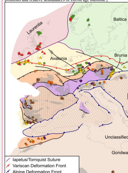
Figure 14: Distribution of Late Ordovician–Devonian strata with published U–Pb zircon isotopic data in the database of Collett (2025). Samples with high proportion of Mesoproterozoic...
