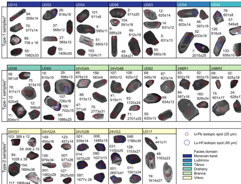
330 Figure 4: Cathodoluminescence images of representative zircons from each sample, with positions of laser spots for U–Pb and Lu– Hf isotope analyses. All zircons in the figure gave concordant (concordia distance <5) ages and the given age is the iterative single- grain concordia age quoted with 2σ uncertainty. *classification into Type-1 and Type-2 samples according to results section.
