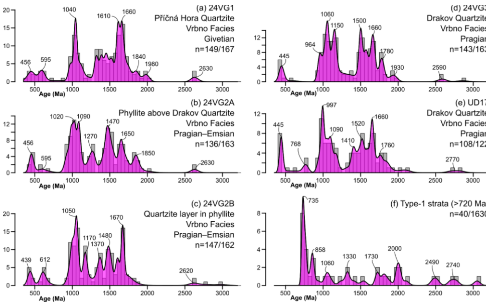
380 Figure 6: Kernel Density Estimates and histograms for the Type-2 samples (a–e) and compiled >720 Ma zircons in the Type-1 strata (f) for comparison.
