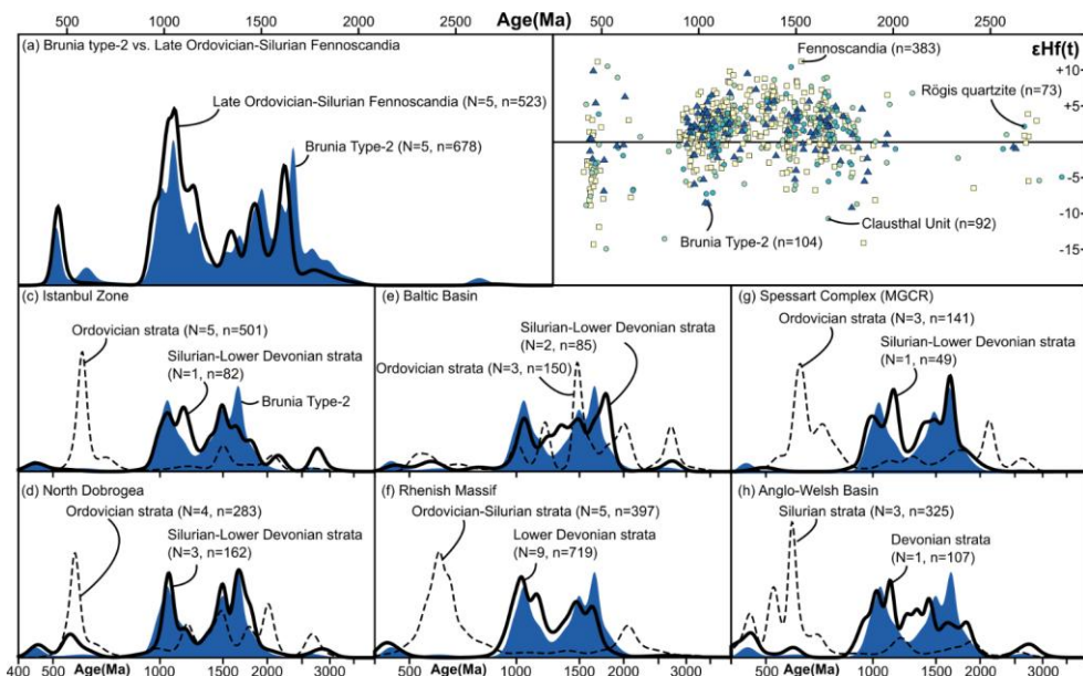
735 Figure 12: (a) Comparison of Brunia Type-2 detrital zircon data with compiled published data from Late Ordovician–Silurian strata of Fennoscandia (Kristoffersen et al., 2014; Sláma, 2016). (b) Comparison of HF-in-zircon isotopic data from the Fennoscandian strata and data from Brunia Type-2 strata, also included are data from the Clausthal Unit (data in Beck et al. 2026) and Rögis quartzite (Zeh and Gerdes, 2010). (c–h) Further comparison of the Brunia Type-2 strata with Late Silurian–Lower Devonian strata from the (c) Istanbul Zone (Akdoğan et al., 2021), (d) North Dobrogea region (Beştepe and Cerna formations in Balintoni and Balica, 2016), (e) Baltic Basin in Estonia (Pöldvere et al., 2014), (f) Rhenish Massif (Eckelmann et al., 2014; Linnemann et al., 2024; Dörr et al., 2025), (g) Spessart Complex in the Mid-German Crystalline Rise (Kirchner and Albert, 2021), and (h) Anglo-Welsh Basin (Waldron et al., 2025). Data used in the construction of this figure is compiled in Collett (2025).
