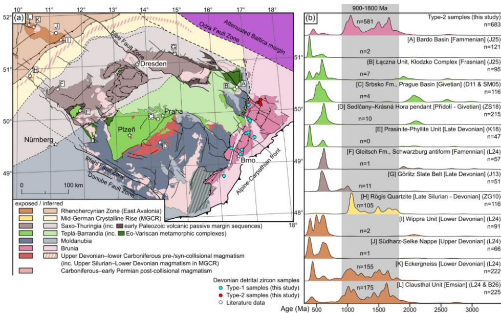
Figure 11: Comparison of published zircon U-Pb data from Devonian strata in the Bohemian Massif and adjacent smaller massifs. (a) Geological map as in Fig. 1a including sample locations. (b) KDE plots of compiled data. J25: Jastrzębski et al. (2025); D11: Drost et al. (2011); SM05: Strnad and Mihaljević (2005); ZS: Žák and Sláma (2018); K18: Koglin et al. (2018); L24: Linnemann et al. (2024); J13: Jähne et al. (2013); ZG10: Zeh and Gerdes (2010); B26: Beck et al. (2026). Shaded area in (b) represents principal range of ages observed in type-2 Brunia samples.
