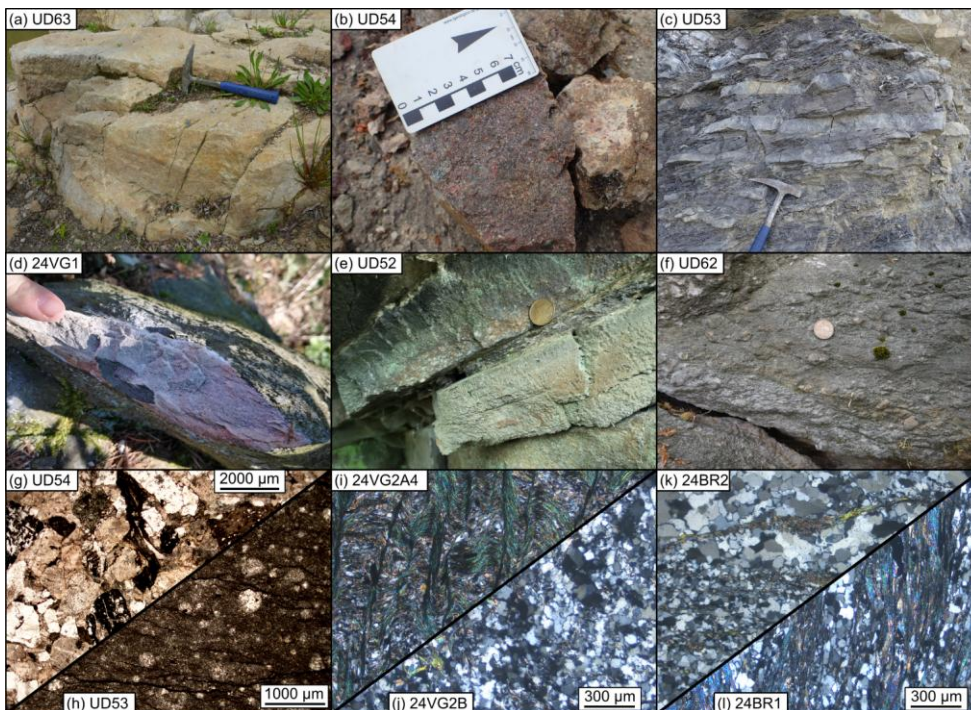
215 Figure 3: Selected field photographs and thin section photographs from representative samples. Refer to Table 1 for location and description of each sample.
