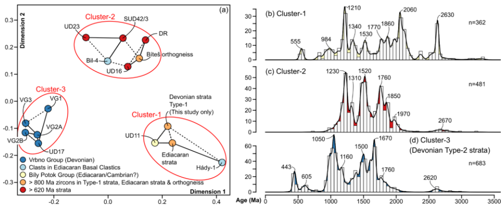
655 Figure 10: (a) Multi-dimensional scaling plot for selected samples from Brunia as well as compiled data from >800 Ma zircons from Type-1 strata, Ediacaran paragneiss and the Bíteš orthogneiss. Note that only >800 Ma zircons are used so as not to overwhelm the statistical comparison with late Neoproterozoic zircons that are minor component in other samples. (b-d) Representative histograms and KDE plots of the data included in each cluster. Data used in construction of this figure was compiled in Collett (2025).
