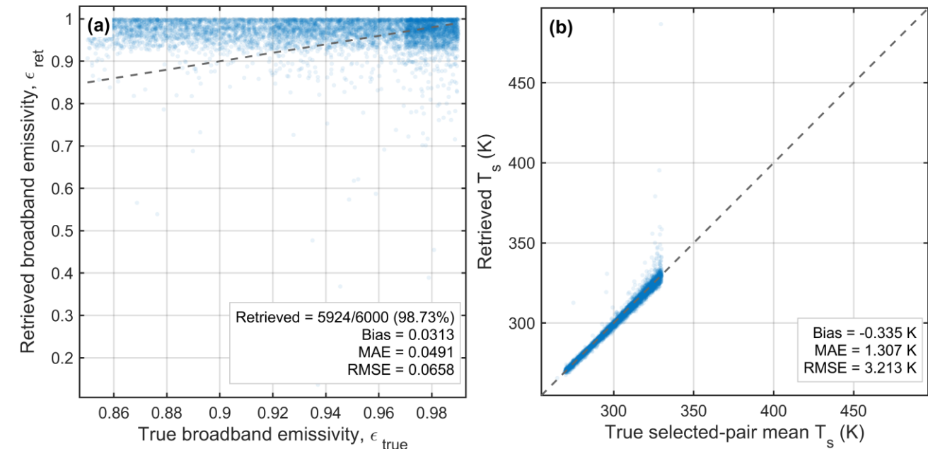
Figure 9. Physics-based known-truth validation for the G1 noiseless experiment. (a) Retrieved versus prescribed broadband emissivity for successful retrievals. (b) Retrieved T_s versus the true surface temperature corresponding to the selected production pair. The success denominator is all 6000 generated scenes; plotted error statistics use successful retrievals only.
