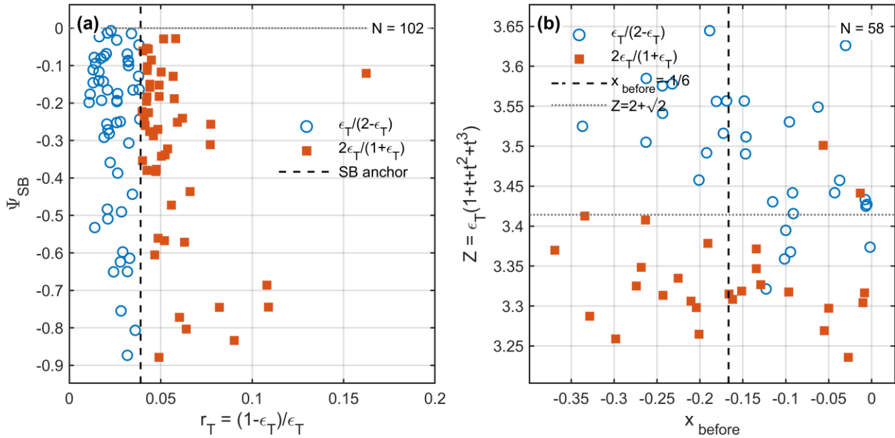
Figure 4. Physical-state applicability of the reciprocal emissivity formulations. (a) Stefan-Boltzmann-controlled configuration expressed in the - state space. (b) Reciprocal-conductance configuration expressed in the - state space. The plotted boundaries are the pre-specified physical applicability conditions used by the production selector.
