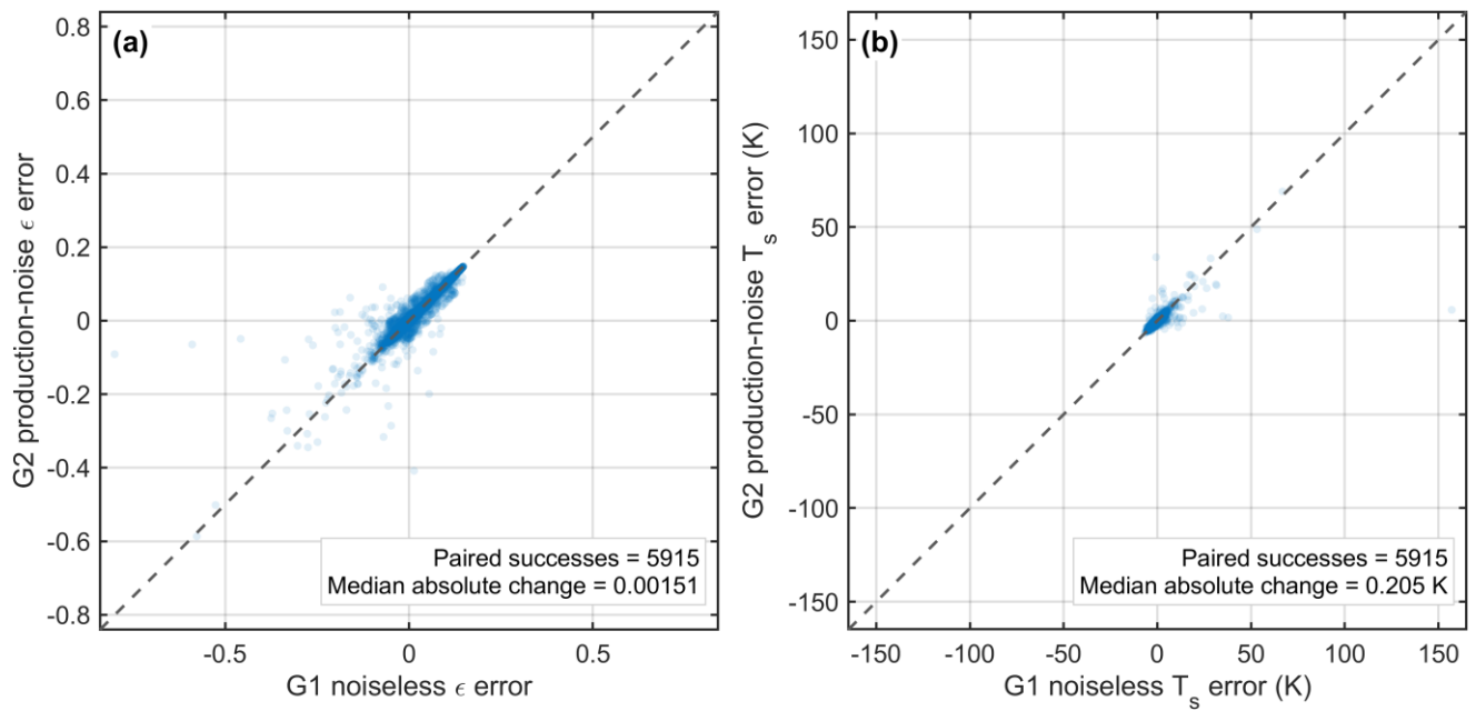
Figure B2. Paired G1-versus-G2 production-noise robustness for the same prescribed truth scenes. The panels compare the change in emissivity error and the change in error when the pre-specified production-noise model is added before preprocessing.
