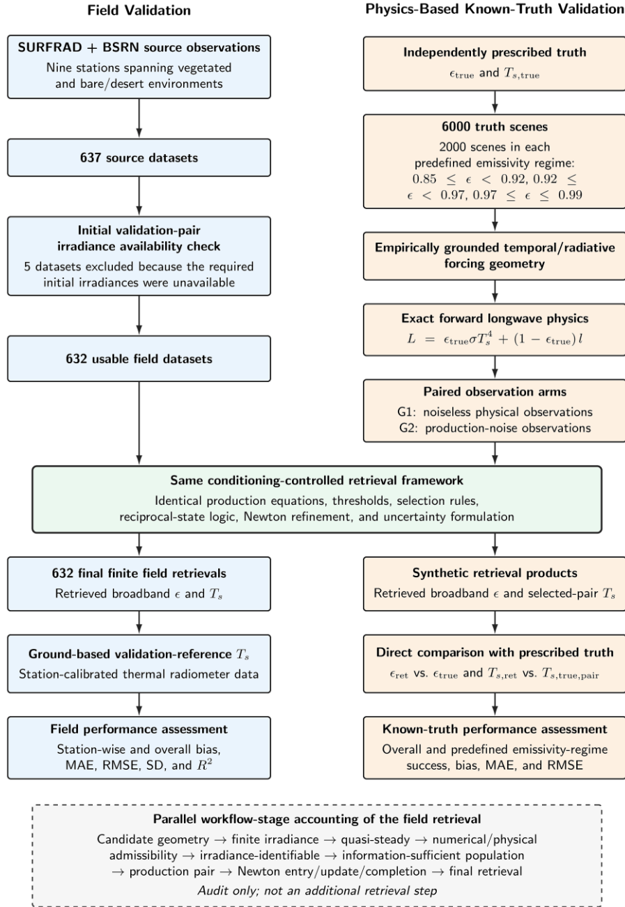
275 Figure 2. Field and physics-based known-truth validation architecture. The field arm retains 632 usable datasets from 637 source datasets; the synthetic arm contains 6000 prescribed truth scenes evaluated as noiseless (G1) and production-noise (G2) observations. Both arms use the same conditioning-controlled retrieval framework.
