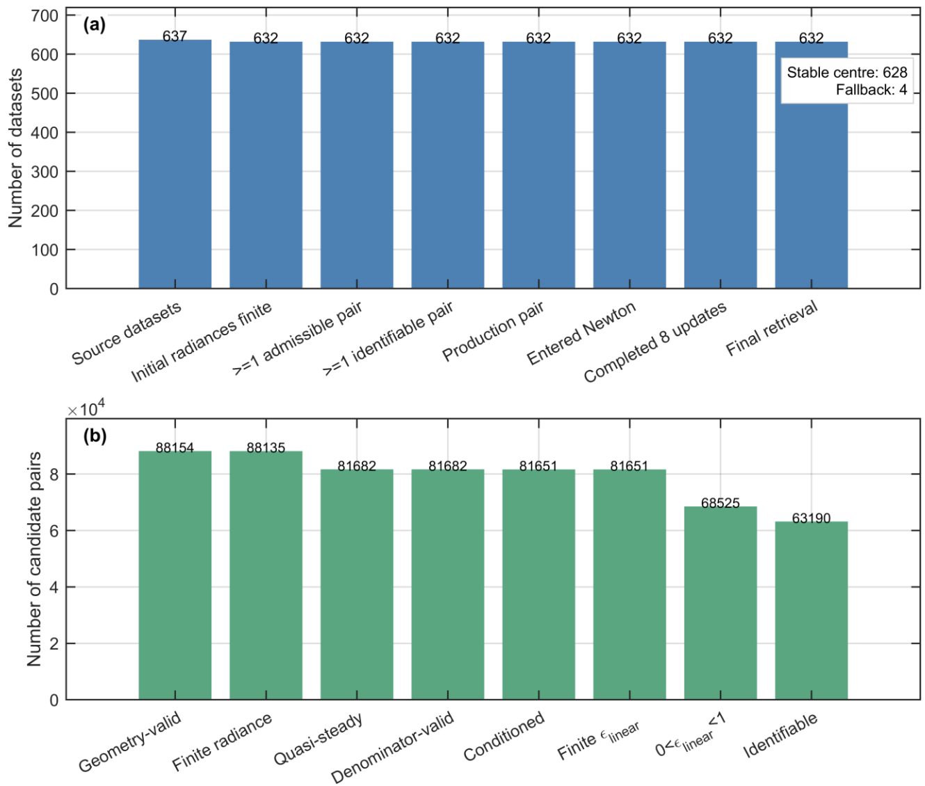
490 Figure A1. Workflow-stage accounting for the field dataset. (a) Scene-level progression from source datasets to final retrievals. (b) Candidate-pair retention through the physical, numerical, and irradiance-identifiability screening stages.
