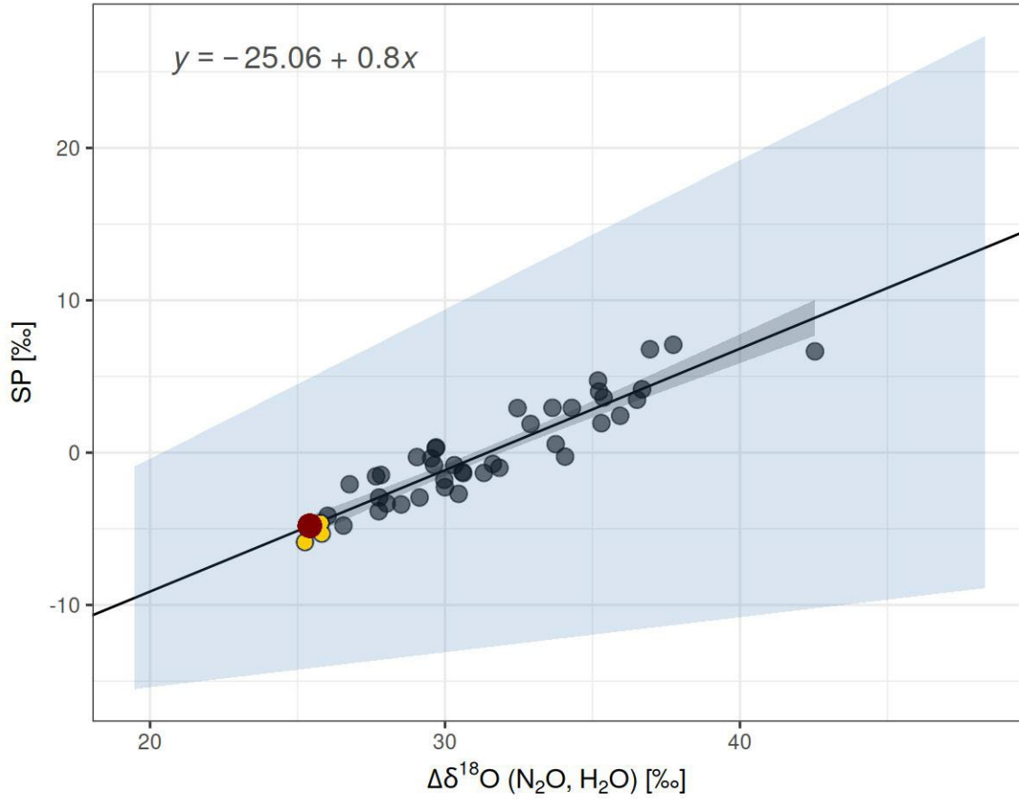
Figure 5: SP plotted against \Delta\delta^{18}\text{O} (\text{N}_2\text{O}, \text{H}_2\text{O}) with the linear regression line representing the study-specific reduction line. Grey area covers the 99 % confidence interval; the blue area indicates the range of reduction slopes reported in the literature (Yu et al., 2020); the red dot represents \delta_0 and the yellow dots the five lowest-ranked points as estimated by the method described in section 2.3.1. Data from February 5 th to February 21 st 2025; n = 45.
