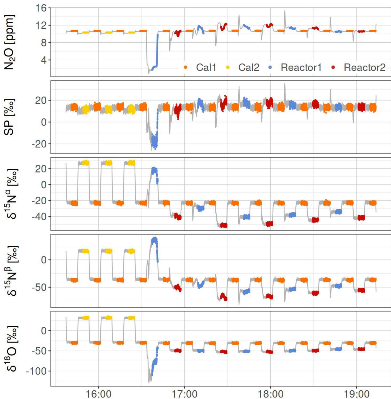
Figure 6: N 2 O mole fraction data and SP, \delta^{15}\text{N}^{\alpha} , \delta^{15}\text{N}^{\beta} , \delta^{18}\text{O} values as provided by the laser spectrometer, i.e. prior to corrections and calibration. Data from June 12 th 2025 under standard WWTP operation conditions. A measurement interval of 8 minutes was chosen and only the last five minutes of each interval were used for further analysis to assure complete exchange of the analyte gas in the gas pretreatment and analyser. Cal1 measurements are shown in orange, Cal2 measurements in yellow and sample measurements in blue (reactor 1) and red (reactor 2).
