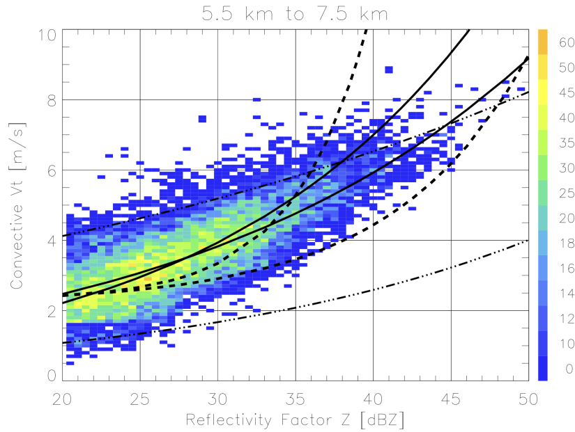
Figure 4: Cumulative histograms for profiler fall speed V_t (adjusted to sea level) versus radar reflectivity factor Z for “convective” media for heights between 5.5 km and 7.5 km agl. Solid lines are the matched profiler behaviors for fits having “a” coefficients = [1.0, 0.71] and “b” coefficients = [0.19, 0.25]. Dashed lines are “graupel” fall speed curves from Giangrande et al. (2013; 2016a). Dashed-dotted lines follow previous fall speed relationships for rain and snow.
