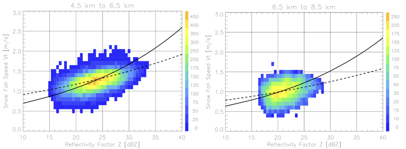
Figure 3: Cumulative histograms for Darwin profiler fall speed Vt (adjusted to sea level) versus radar reflectivity factor Z for snow above bright band signatures, for heights between 4.5 km and 6.5 km agl (left panel), and 6.5 km and 8.5 km agl (right panel). The solid line represents the fall speed relationship coefficient “a” = 0.45 (left panel) and 0.41 (right panel) for a fixed “b” coefficient of 0.19. The dashed lines represent our dataset best-fit “a” = 0.72 (left panel) and 0.62 (right panel) for a fixed “b” = 0.1.
