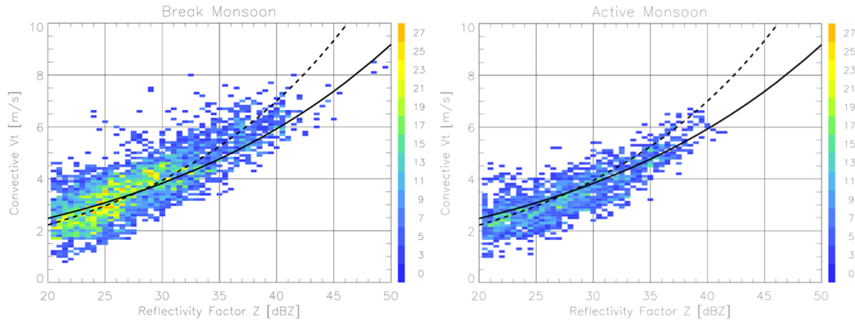
Figure 5: As in Fig. 4, but for (left) Break monsoon and (right) Active monsoon regime date breakdowns. Solid line is matched to profiler behaviors for the fit having coefficients [“a”, “b”] = [1.0, 0.19]. Dashed line is for coefficients = [0.72, 0.25].
