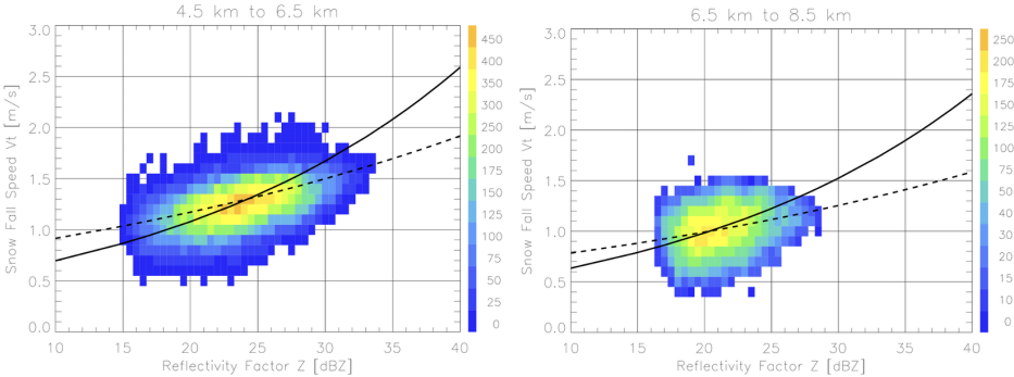
Figure 3: Cumulative histograms for Darwin profiler fall speed V_t (adjusted to sea level) versus radar reflectivity factor Z for snow above bright band signatures, for heights between 4.5 km and 6.5 km agl (left panel), and 6.5 km and 8.5 km agl (right panel). The solid line represents the fall speed relationship coefficient “ a ” = 0.45 (left panel) and 0.41 (right panel) for a fixed “ b ” coefficient of 0.19. The dashed lines represent our dataset best-fit “ a ” = 0.72 (left panel) and 0.62 (right panel) for a fixed “ b ” = 0.1.
