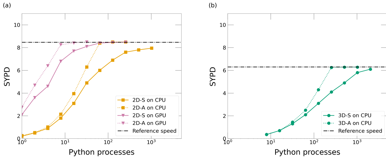
Figure 7. (a): NEMO simulation speed in Simulated Year Per Day for eORCA025.L75 as function of the number of processes allocated to the 2D case Python script executed on CPUs and on GPUs, and for different coupling implementation, asynchronous (-A) and synchronous (-S). Number of processes allocated to NEMO is fixed and equal to 999. (b): Same with the 3D case Python script executed on CPUs.
