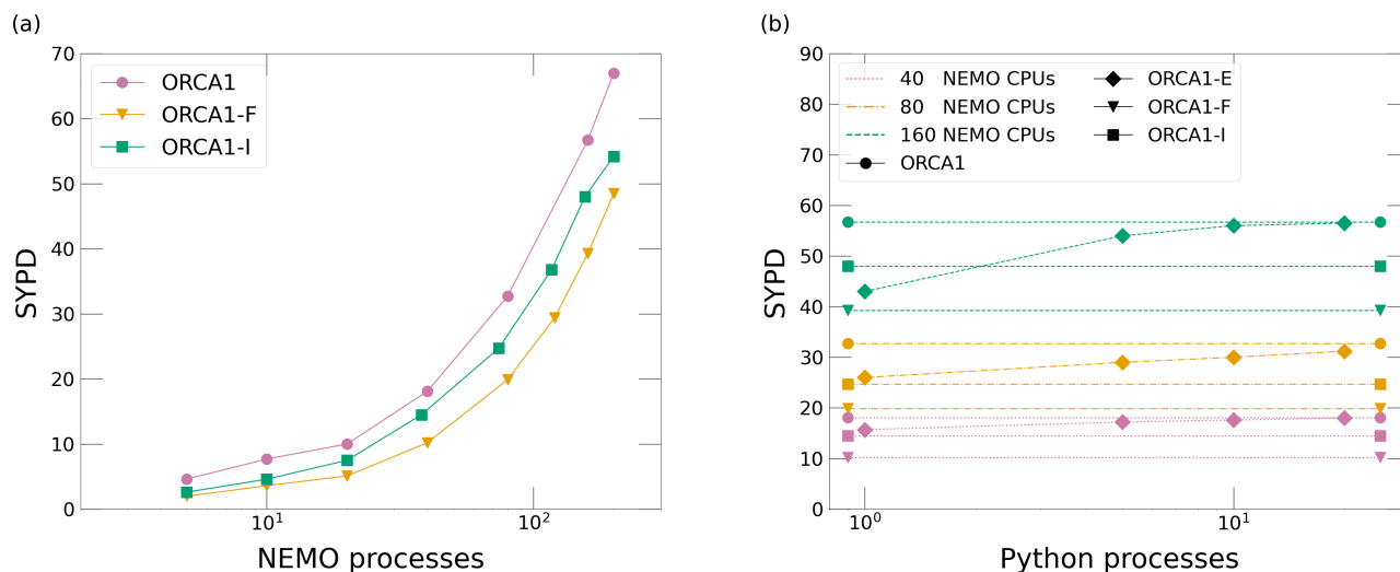
Figure 9. (a) Simulation speed in Simulated Year Per Day as function of the number of processes allocated to NEMO for different implementation of the Storto et al. (2024) ML model: NEMO without ML model (ORCA1), with Fortran (ORCA1-F), and Infero (ORCA1-I). (b) Simulation speed in Simulated Year Per Day for ORCA1-E as a function of the number of processes allocated to the Python script for different number of processes allocated to NEMO. Results are compared for different implementation of the Storto et al. (2024) ML model: NEMO without ML model (ORCA1), with Fortran (ORCA1-F) and Infero (ORCA1-I). Lines for those cases are here for readability as their values are fixed and independent of the number of Python processes.
