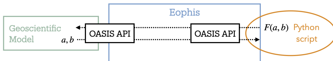
Figure 1. Coupling through OASIS3-MCT with Eophis principle diagram. The geoscientific model and Eophis are executed independently. Both can exchange data through the coupling library. Eophis flexibly automates the configuration of the OASIS3-MCT Python API, and runs a generic Python environment compatible with the OASIS3-MCT usage in which any functions can be imported.
