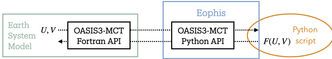
Figure 1. Coupling through OASIS3-MCT with Eophys principle diagram. The Earth System Model and Eophys are executed independently. Both can exchange data through the coupling library. Eophys flexibly automates the configuration of the OASIS3-MCT Python API, and runs a generic Python environment compatible with the OASIS3-MCT usage in which any functions can be imported. In this example, the Earth System Model sends two fields named U and V to Eophys through OASIS3-MCT. These are passed as arguments to the Python function F , imported from a separate Python script, and Eophys leverages OASIS3-MCT Python API to send the result back to the Earth System Model.
