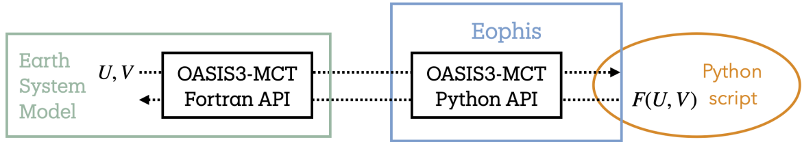
Figure 1. Coupling through OASIS3-MCT with Eophis principle diagram. The Earth System Model and Eophis are executed independently. Both can exchange data through the coupling library. Eophis flexibly automates the configuration of the OASIS3-MCT Python API, and runs a generic Python environment compatible with the OASIS3-MCT usage in which any functions can be imported. In this example, the Earth System Model sends two fields named U and V to Eophis through OASIS3-MCT. These are passed as arguments to the Python function F , imported from a separate Python script, and Eophis leverages OASIS3-MCT Python API to send the result back to the Earth System Model.
