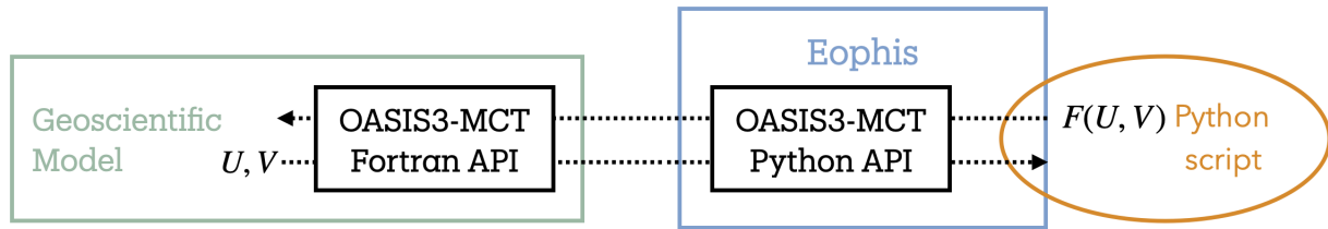
Figure 1. Coupling through OASIS3-MCT with Eophis principle diagram. The geoscientific model and Eophis are executed independently. Both can exchange data through the coupling library. Eophis flexibly automates the configuration of the OASIS3-MCT Python API, and runs a generic Python environment compatible with the OASIS3-MCT usage in which any functions can be imported. In this example, the geoscientific model sends two fields named U and V to Eophis through OASIS3-MCT. These are passed as arguments to the Python function F , imported from a separate Python script, and Eophis leverages OASIS3-MCT Python API to send the result back to the geoscientific model.
