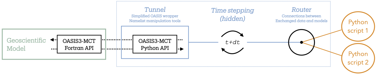
Figure 2. Eophis (dashed line rectangle) elements diagram. The Tunnel component is an OASIS3-MCT wrapper that configures the Python coupling API from the exchanges defined at the Eophis abstraction level. The Router configures the connections between received fields and the inputs of the Python functions, as well as between function outputs and the fields to be sent back. During execution, Eophis emulates the time-stepping to synchronize exchanges as the geoscientific model progresses in time: the Tunnel receives fields from the geoscientific model through OASIS3-MCT. These fields are passed to the Router, which dispatches them to the appropriate Python functions and collects the returned outputs. Once the outputs are available, the time-stepping instructs the Tunnel to send the resulting fields back through OASIS3-MCT, and the cycle repeats.
