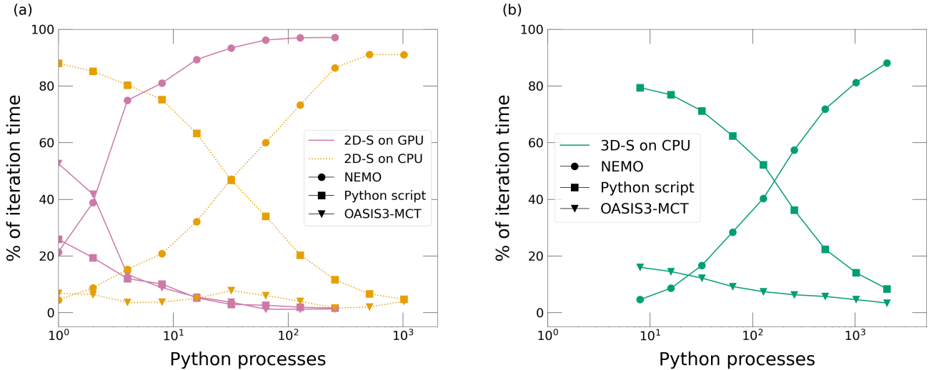
Figure 8. (a) Averaged percentage of time repartition of a NEMO iteration between OASIS3-MCT routines, execution of the 2D case Python script and NEMO routines with the synchronous (-S) implementation for eORCA075.L75 as function of the number of processes allocated to the 2D case Python script. (b) Same with the 3D case Python script executed on CPUs.
