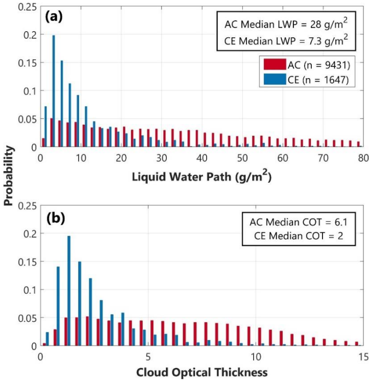
Figure 109: Distributions of (a) LWP and (b) COT for all AC data points (red) and CE data points (blue). Median values for both variables and both subsets of data are also shown.
