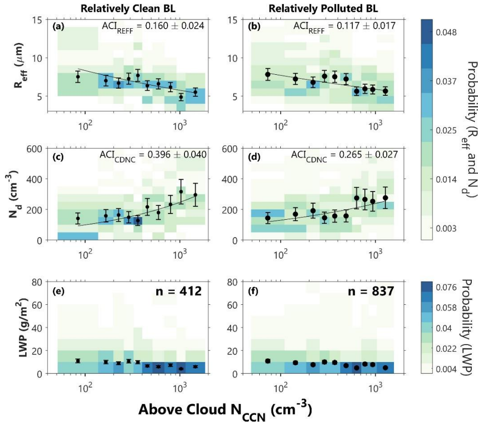
Figure 8: Results of from CE data set ( n = 12491174 ) show the relationship between above-cloud N_{CCN} and (a-b) R_{eff} , (c-d), N_d , and (e-f) LWP for cases with a relatively clean BL (below-cloud N_{CCN} \leq 350 cm^{-3} ) and a relatively polluted BL (below-cloud N_{CCN} > 350 cm^{-3} ). The shading, scatter points, ACI metrics, and fit lines are calculated and displayed in the same way as Fig. 4.
