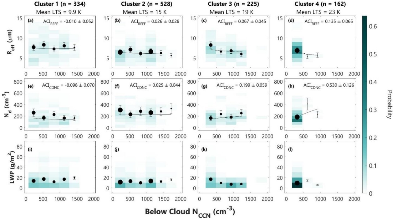
Figure B1: Below-cloud observations from Fig. 7 are assigned to clusters determined in Fig. 5. Results of this clustering show the relationship between below-cloud N_{CCN} and (a-d) R_{eff} , (e-h) N_d , and (i-l) LWP. Average LTS in each cluster increases from left to right. The shading, scatter points, ACI metrics, and fit lines are calculated and displayed in the same way as Fig. 4.
