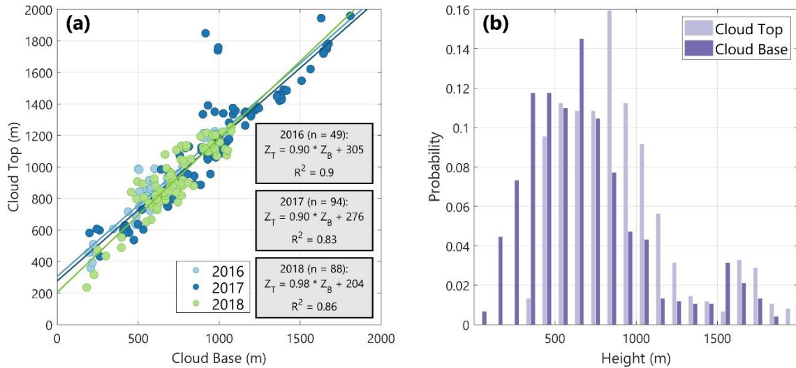
Figure A1: (a) In situ derived relationship between cloud top height ( Z_T ) and cloud base height ( Z_B ) based on the methodology of Gupta et al. (2021). These relationships are applied to HSRL-2 cloud top heights measured at cloud edge for all three deployment years of ORACLES. The distributions of these HSRL-2 measured cloud top heights and resultant calculated cloud base heights are given in panel (b).
