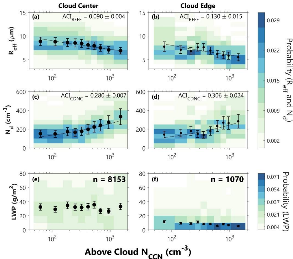
Figure 114: Results from cloud center and CE data sets show the relationship between above-cloud N_{CCN} and (a-b) R_{eff} , (c-d) N_d , and (e-f) LWP. The shading, scatter points, ACI metrics, and fit lines are calculated and displayed in the same way as Fig. 4.
