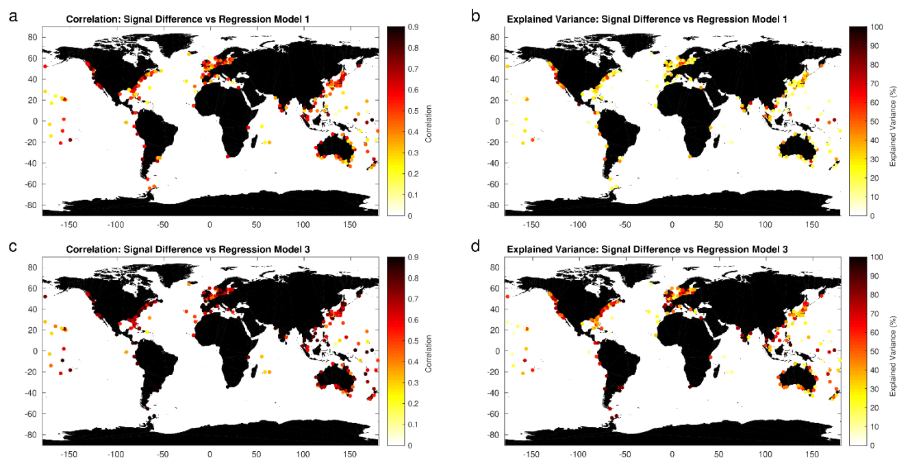
Figure 11 The correlations (a) between the Signal Differences and the regression Model 1, Eq. (3) and the corresponding explained variance (b). The correlations (c) between the Signal Differences and the regression Model 3, Eq. (5) and the corresponding explained variance (d).
