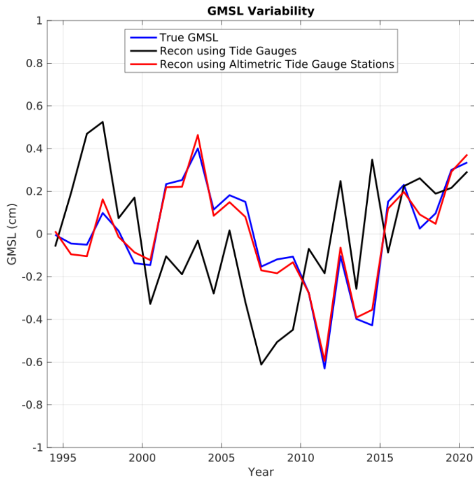
332 Figure 5 Comparison between the true GMSL and our GMSL reconstructions using tide gauge 333 observations (black line) and virtual altimetric tide gauges (red line) for the period 1994 334 to 2020. The ‘true’ GMSL derived from altimetry is shown as a blue line. All timeseries 335 are detrended.
