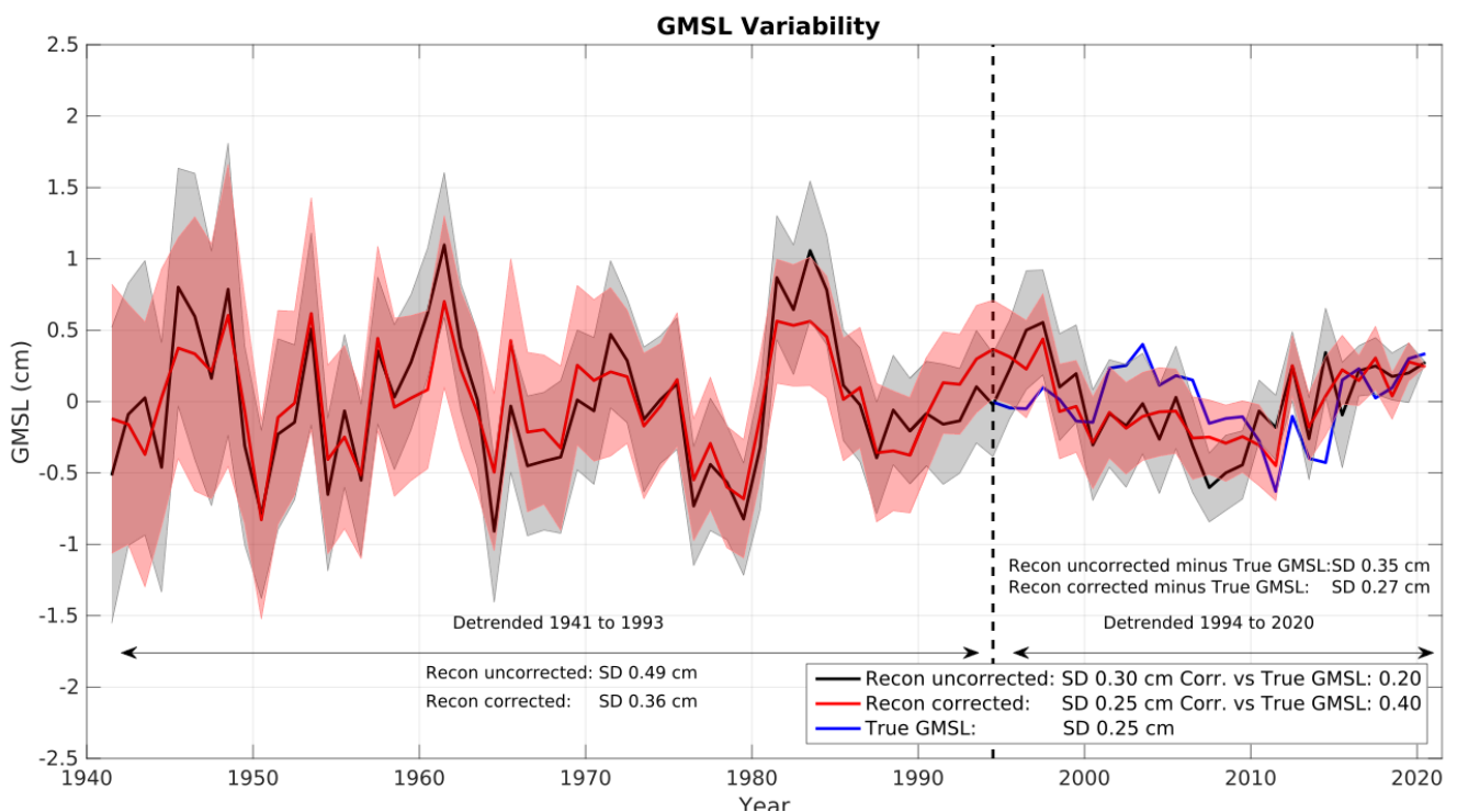
Figure 13 The variability of the GMSL that has been detrended for two time periods 1941 to 1993 and 1994 to 2020 showing the uncorrected EOF reconstruction (black line) derived from Eq. (2) and the corrected EOF reconstruction (red line). The 1-sigma uncertainty intervals shaded grey (uncorrected) and light red (corrected) reflect the sensitivity of the reconstruction to the number of tide gauges as evaluated standard deviation (SD) using a bootstrap method. The detrended ‘true’ GMSL derived from altimetry is shown as a blue line (1994 to 2020).
