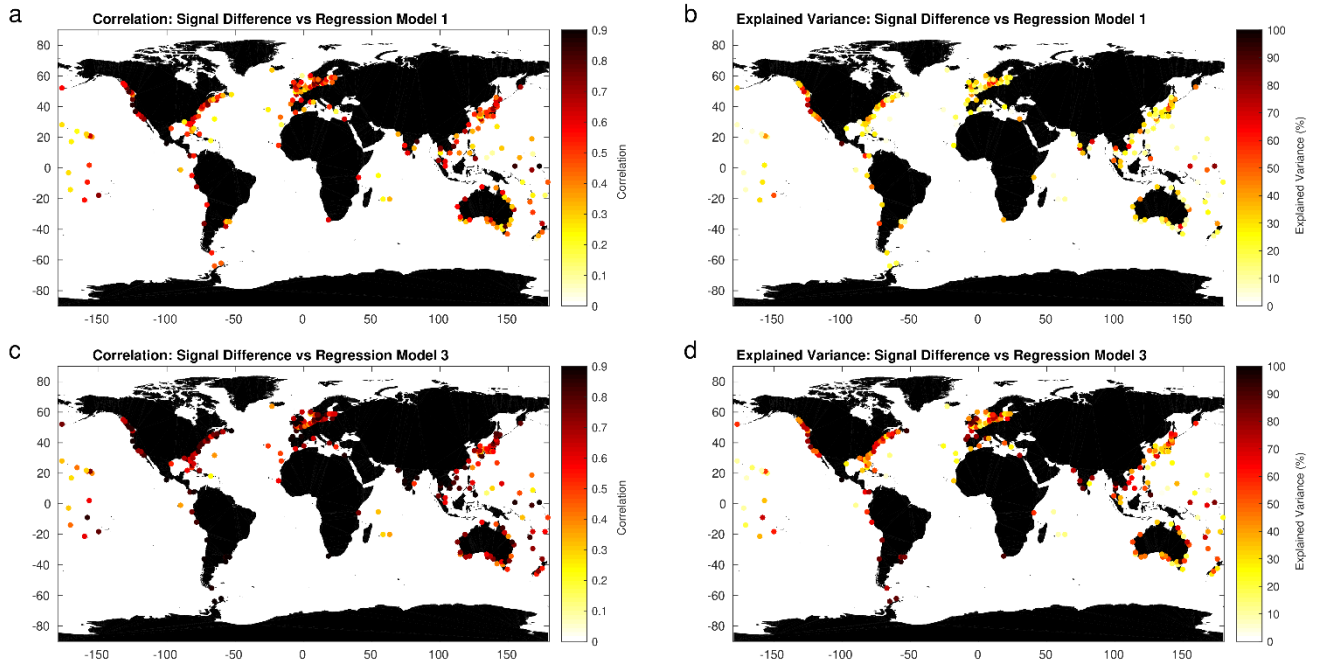
Figure 11 The correlations (a) between the Signal Differences and the regression Model 1, Eq. (23) and the corresponding explained variance (b). The correlations (c) between the Signal Differences and the regression Model 3, Eq. (45) and the corresponding explained variance (d).
