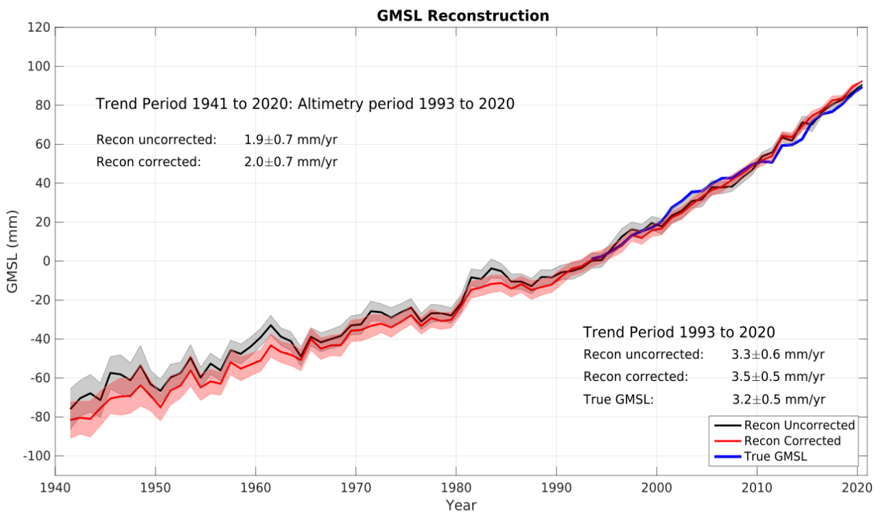
Figure 12 Comparison of uncorrected EOF reconstruction (black line) derived from Eq. (42) and the corrected EOF reconstruction (red line). The 1-sigma uncertainty intervals,
