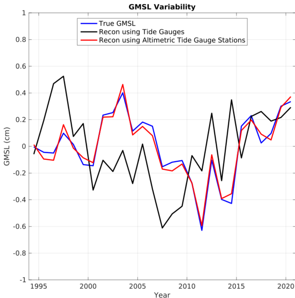
335 Figure 5 Comparison between the true GMSL and our GMSL reconstructions using tide gauge 336 observations (black line) and virtual altimetric tide gauges (red line) for the period 1994 337 to 2020. The ‘true’ GMSL derived from altimetry is shown as a blue line. All timeseries 338 are detrended.
