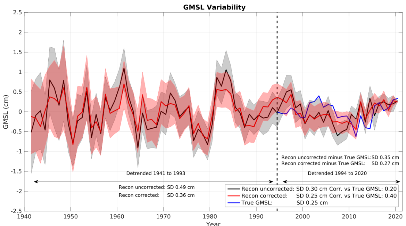
Figure 13 The variability of the GMSL that has been detrended for two time periods 1941 to 1993 and 1994 to 2020 showing the uncorrected EOF reconstruction (black line) derived from Eq. (42) and the corrected EOF reconstruction (red line). The 1-sigma
