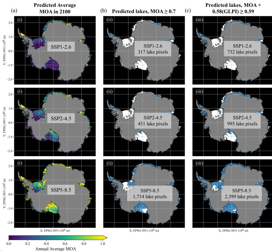
Figure A4: Projections of MOA and lake distribution in 2100 under three emissions pathways across all Antarctic ice-shelves at 27 km resolution. Panels i-iii show (i) projected annual average MOA from 2090-2099, (ii) projected surface meltwater distribution based on the theoretical threshold of \text{MOA} \geq 0.7 , and (iii) projected surface meltwater distribution based on the empirical continent-wide threshold of \text{MOA} + 0.58(\text{GLPI}) \geq 0.59 , under emissions pathways (a) SSP1-2.6, (b) SSP2-4.5, and (c) SSP5-8.5. MOA projections are derived from RACMO2.3p2 climate model outputs (van Wessem et al., 2022).
