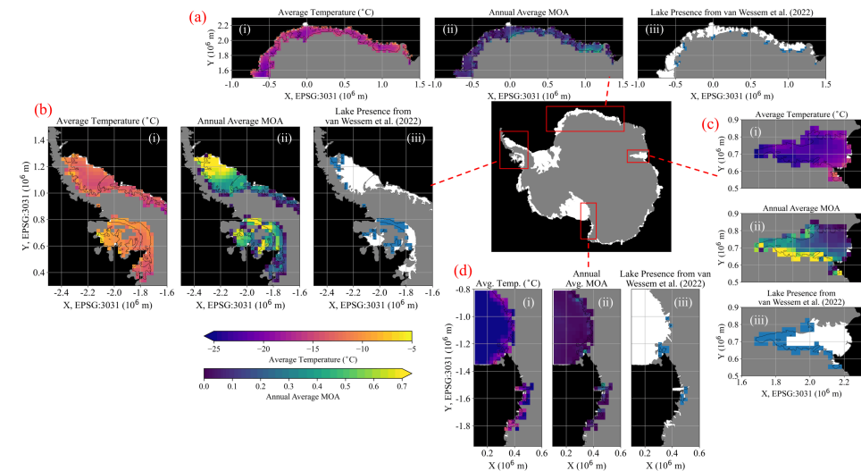
75 Figure 1: Regional climate data and binarized surface meltwater distribution across selected Antarctic ice-shelf areas at 27 km resolution. The central map shows all ice shelves with the four focus areas outlined: (a) Dronning Maud Land, (b) Antarctic Peninsula, (c) Amery Ice Shelf, and (d) western Ross Ice Shelf. For each region, panels i-iii show (i) average 2 m air temperature, (ii) annual average meltwater-over-accumulation (MOA), and (iii) observed surface meltwater distribution from van Wessem et al. (2022). Temperature and MOA are outputs from RACMO2.3p2 averaged over the period 1979-2022. Surface meltwater distribution is derived from Sentinel-2 80 imagery spanning austral summers 2015-2022 (van Wessem et al., 2022).
