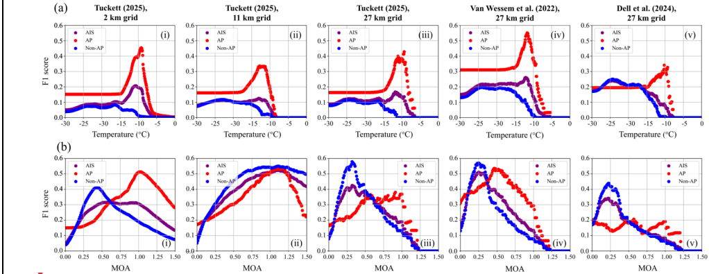
Figure 5: Performance of temperature and MOA thresholds as predictors of surface meltwater distribution across all five comparison scenarios. Each panel shows F1 scores as a function of (a) average temperature or (b) annual average MOA for the entire Antarctic Ice Sheet (AIS; purple), the Antarctic Peninsula (AP; red), and the remainder of the ice sheet excluding the Peninsula (Non-AP; blue). Results are shown for lakes datasets from Tuckett et al. (2025) at 2, 11, and 27 km resolutions (i), (ii), (iii)), van Wessem et al. (2022) at 27 km resolution (iv), and Dell et al. (2024a) at 27 km resolution (v). Temperatures and annual MOA's are averaged over the period 1979-2022 or 2023, as indicated in Table 1.
