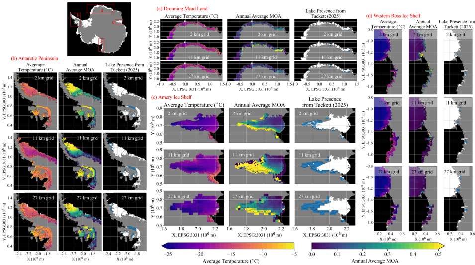
Figure A1: Regional climate data and binarized surface meltwater distribution across selected Antarctic ice-shelf areas at 2 km, 11 km, and 27 km resolutions. The map in the upper left shows all ice shelves with the four focus areas outlined: (a) Dronning Maud Land, (b) Antarctic Peninsula, (c) Amery Ice Shelf, and (d) western Ross Ice Shelf. For each region, panels show average 2 m air temperature (left columns), annual average meltwater-over-accumulation (MOA) (center columns), and observed surface meltwater distribution from Tuckett (2025) (right columns). Data is shown at 2 km resolution (top rows), 11 km resolution (center rows), and 27 km resolution (bottom rows). Surface meltwater distribution is derived from Landsat 7 and 8 imagery spanning 2006-2021 (Tuckett, 2025). RACMO climate model iterations and time spans for temperature and MOA outputs can be seen in Table 1.
