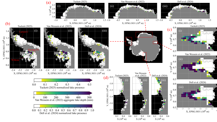
Figure 4: Surface meltwater distribution across selected Antarctic ice-shelf areas at 27 km resolution. The central map shows all ice shelves with the four focus areas outlined: (a) Dronning Maud Land, (b) Antarctic Peninsula, (c) Amery Ice Shelf, and (d) western Ross Ice Shelf. For each region, panels i-iii show observed surface meltwater aggregated on to the 27 km RACMO2.3p2 grid as follows: (i) normalized lake presence from 2006-2021 (Tuckett, 2025) (ii) aggregate meltwater depth from austral summers 2015-2022 (van Wessem et al., 2022), and (iii) normalized lake presence from austral summers 2013-2021 (Dell et al., 2024a). White areas indicate insufficient meltwater to reach the binarizing threshold for each data set (see text for more details). Locations of Antarctic Peninsula ice shelves mentioned in the text are indicated in panel (b) (i).
