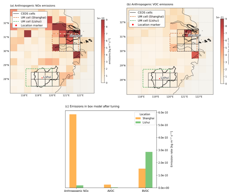
Figure 2. Anthropogenic and biogenic emission fields and box-model emission inputs. (a) CEDS anthropogenic NO x emissions over the study region for JJA 2022 ( \text{kg NO m}^{-2} \text{s}^{-1} ). (b) CEDS anthropogenic VOC species included in the box-model emission input, calculated as the sum of C 2 H 6 , C 3 H 8 , and HCHO emissions ( \text{kg VOC m}^{-2} \text{s}^{-1} ). (a,b) Spatial selection used to define the Shanghai and Lishui model emissions: municipal outlines (black); Grey cells indicate the CEDS grid cells selected to calculate the Shanghai and Lishui anthropogenic emission inputs. The dashed orange (Shanghai) and green (Lishui) outlines show the corresponding grid cells used in the UKESM-AMIP and are included only to show their spatial relationship to the selected CEDS cells. (c) Final box-model emission inputs for anthropogenic NO x , sum of AVOC species included in the box-model input, and BVOCs (units: \text{kg m}^{-2} \text{s}^{-1} ). Coastlines from Natural Earth ( naturalearthdata.com ). Administrative boundaries from the GADM database ( www.gadm.org ).
