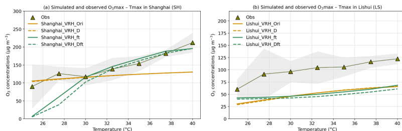
Figure 8. Comparison of observed and simulated O 3 max-T max relationships for (a) Shanghai and (b) Lishui (summer, JJA). Observations are shown as olive triangles connected by a line; the grey envelope denotes the 95% confidence interval of the observed bin means (2.5 °C T max bins; e.g., the 25 °C bin denotes summer days with T max 23.75-26.25 °C). Colored solid/dashed lines show the four model configurations (VRH_Ori, VRH_D, VRH_ft, VRH_Dft; see Table 3).
