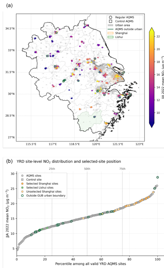
Figure 1. (a) Spatial distribution of Air Quality Monitoring Sites (AQMS) across the YRD in summer 2022, coloured by JJA 2022 mean \text{NO}_2 . Grey shading indicates the 2018 Global Urban Boundaries (GUB) urban settlement extent. Circular markers denote regular AQMS, square markers denote control sites, and green outlines indicate sites located outside the GUB urban settlement boundary. Shanghai and Lishui are highlighted by coloured city polygons. (b) Ranked distribution of JJA 2022 mean \text{NO}_2 across all valid YRD AQMS, expressed as site percentile. Selected Shanghai and Lishui sites (listed in Table 1) are highlighted in orange and green, respectively; unselected Shanghai sites are shown in pale orange, and sites outside the GUB urban boundary are outlined in dark green. Administrative boundaries from the GADM database ( www.gadm.org ).
