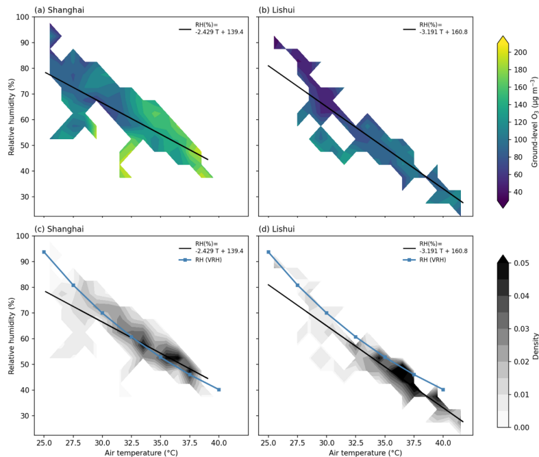
Figure 5. Observed air temperature-relative humidity space for (a, c) Shanghai and (b, d) Lishui (daytime, T \geq 25^\circ\text{C} ). Panels (a-b) show the ground-level \text{O}_3 ( \mu\text{g m}^{-3} ) binned on a 1^\circ\text{C} \times 5\% RH grid; panels (c-d) show the data density (fraction of site samples per bin) on the same grid. The solid black line in each panel is the ordinary-least-squares fit of RH to T from the unbinned 3-hourly records. Ozone: hourly observations averaged from 8 AQMS (Shanghai) and 3 AQMS (Lishui); meteorology: three-hourly MMS data; all aggregated to 3-h means. The blue solid line with square markers in panels (c-d) is the RH curve with conserved absolute humidity ( q=0.0184 \text{ kg kg}^{-1} ) used in the VRH model scenario.
