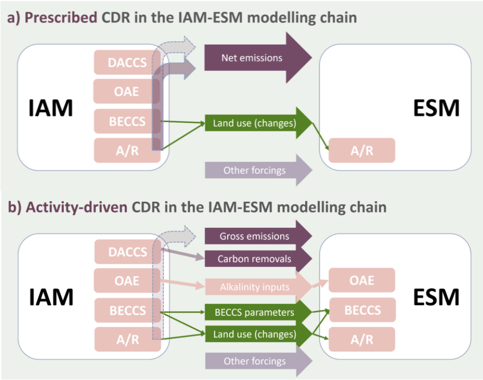
Figure 1: Schematic of prescribed (a) and activity-driven (b) CDR in the IAM-ESM modelling chain. Panel a depicts the current state-of-the-art, which has been used for CMIP5 and 6, and is planned for CMIP7. Panel (b) depicts activity-driven CDR as discussed in this paper.
