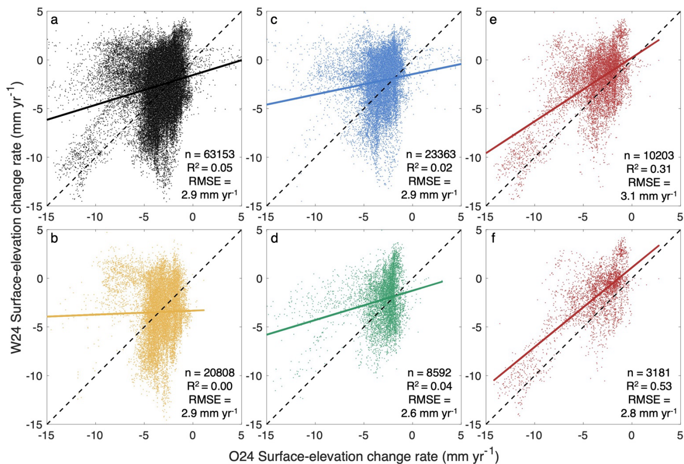
Figure 2. Pixel-by-pixel comparison of surface-elevation change (SEC) rates between the O24 (Ohenhen et al., 2024) and W24 (Wang et al., 2024) datasets. (a) All pixels; (b) Agricultural land; (c) Wetlands; (d) Upland vegetation; (e) Developed land; (f) Medium to high developed land. The thick line in each panel represents the best-fit linear regression between the two datasets. Dashed lines indicate the 1:1 reference line. The number of pixels, corresponding R^2 value, and root-mean-square error (RMSE) relative to the 1:1 line are shown in the lower right corner.
