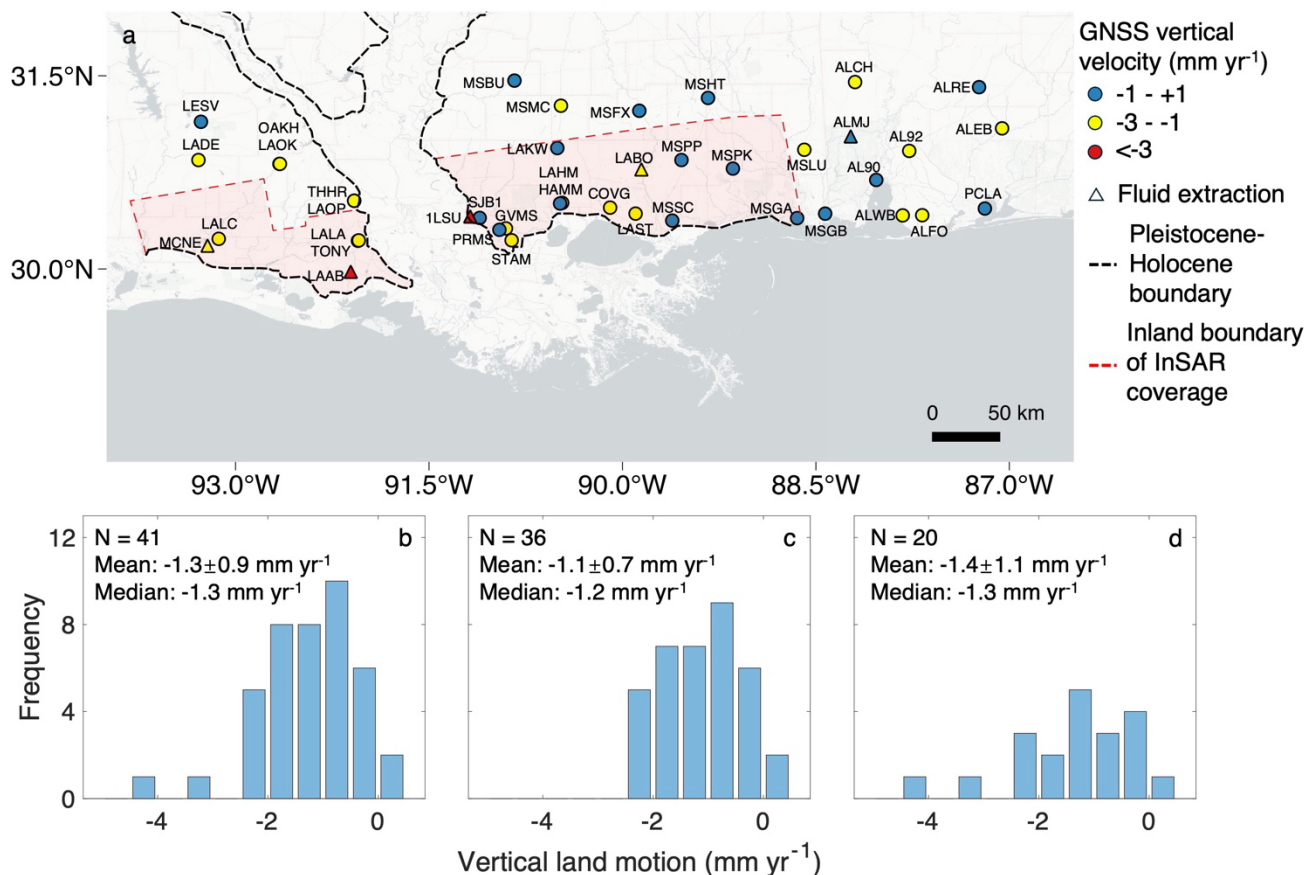
Figure 3. Distribution of GNSS sites and frequency histograms of corresponding vertical land motion in the Pleistocene landscape along the central U.S. Gulf Coast. Data are provided in the Data Set S1 (a) Map with the GNSS sites. The Pleistocene-Holocene boundary is simplified based on the Quaternary geologic map of the Lower Mississippi Valley (Autin et al., 1991; Saucier, 1994). Frequency histograms and associated statistics are shown for (b) all 41 GNSS sites; (c) 36 GNSS sites with minimal human influence; and (d) all 20 GNSS sites within the InSAR coverage area (pink shaded area).
