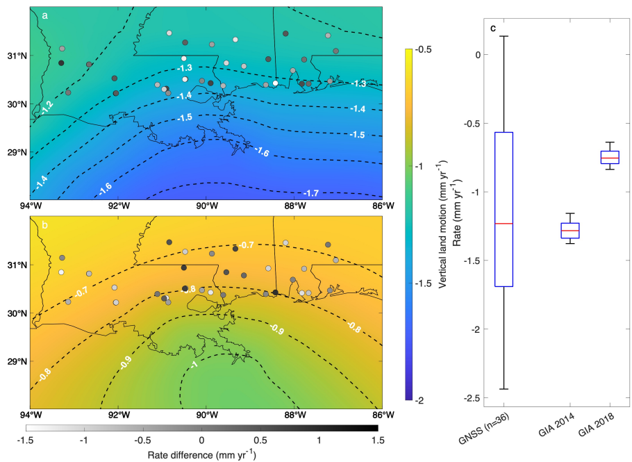
Figure 5. Modeled vertical land motion (VLM) induced by glacial isostatic adjustment (including sediment loading) and rate differences with GNSS observations along the central U.S. Gulf Coast (sites from Figure 3c). (a) VLM from Wolstencroft et al. (2014) and rate difference between GNSS-derived VLM and modeled VLM within 50 km of each GNSS site. (b) VLM from (Kuchar et al., 2018) and rate difference between GNSS-derived VLM and modeled VLM within 10 km of each GNSS site. (c) Boxplots of VLM rates from GNSS (Wolstencroft et al., 2014); GIA 2014) and (Kuchar et al., 2018); GIA 2018).
