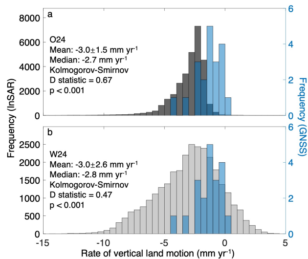
Figure 4. Comparison of InSAR and GNSS-derived vertical land motion in the Pleistocene landscape by means of frequency histograms. (a) O24 (Ohenhen et al., 2024); (b) W24 (Wang et al., 2024). GNSS sites are located within the InSAR coverage area (Figures 3a, d).
