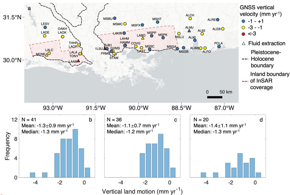
Figure 3. Distribution of GNSS sites and frequency histograms of corresponding vertical land motion in the Pleistocene landscape along the central U.S. Gulf Coast. Data are provided in the Supplementary Spreadsheet. (a) Map with the GNSS sites. The Pleistocene-Holocene boundary is simplified based on the Quaternary geologic map of the Lower Mississippi Valley (Autin et al., 1991; Saucier, 1994). Frequency histograms and associated statistics are shown for (b) all 41 GNSS sites; (c) 36 GNSS sites with minimal human influence; and (d) all 20 GNSS sites within the InSAR coverage area (pink shaded area).
