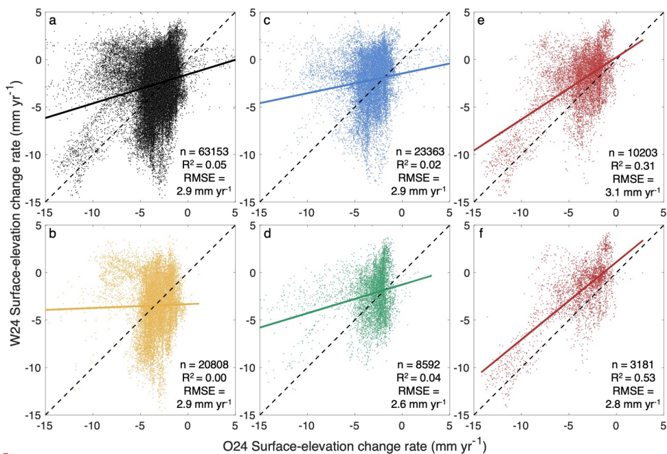
Figure 2. Pixel-by-pixel comparison of surface-elevation change (SEC) rates between the O24 (Ohnenhen et al., 2024) and W24 (Wang et al., 2024) datasets. (a) All pixels; (b) Agricultural land; (c) Wetlands; (d) Upland vegetation; (e) Developed land; (f) Medium to high developed land. The thick line in each panel represents the best-fit linear regression between the two datasets. Dashed lines indicate the 1:1 reference line. The number of pixels, corresponding R² value, and root-mean-square error (RMSE) relative to the 1:1 line are shown in the lower right corner.
