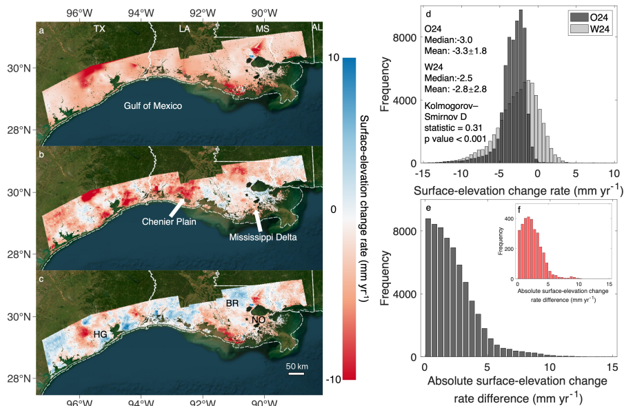
Figure 1. Maps of InSAR-derived surface-elevation change (SEC) rates and corresponding frequency histograms. (a) SEC data from the Ohenhen et al. (2024) dataset (O24), converted to match the resolution of the Wang et al. (2024) dataset (W24). TX: Texas, LA: Louisiana, MS: Mississippi, AL: Alabama; (b) SEC data from the W24 dataset; (c) SEC difference between O24 and W24. HG: Houston-Galveston area, BR: Baton Rouge, NO: New Orleans; (d) Frequency histograms and statistics of O24 and W24 SEC rates; (e) Frequency histogram of absolute SEC rate differences between O24 and W24; (f) Same as (e), but for medium to high developed land, where the impervious surface cover exceeds 50%.
