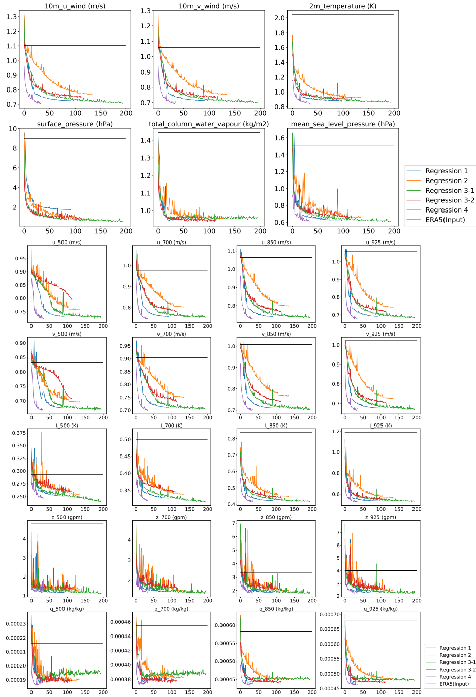
Figure 2. Validation curves of regression models for surface variables (top) and pressure level variables (bottom). Each subplot corresponds to a target variable. The curves plot the Mean Absolute Error (y-axis) against the number of training epochs (x-axis). ERA5 is used as the ground truth.
