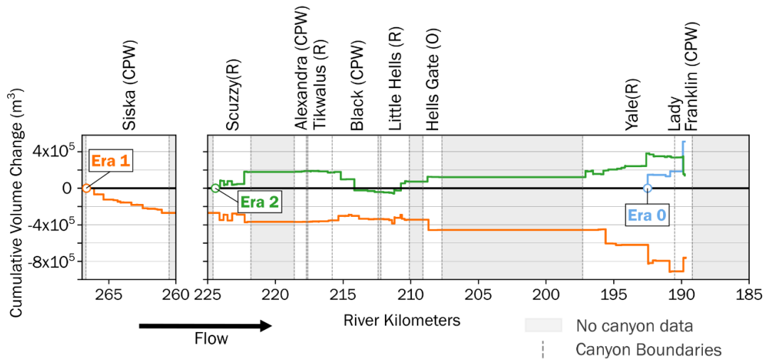
Figure 10. Flux divergence through the surveyed canyons for each Era, calculated as cumulative change in patch volume summed from upstream to downstream. Analysis shows that Era 0 and Era 2 were dominated by deposition while erosion dominated during Era 1. The upstream-most point with data is labeled for each Era. Regions without survey data are shaded grey, so flux divergence is assumed to be constant throughout these reaches. In brackets after canyon names their morphology is noted (“CPW” for constriction-pool-widenings, “R” for rapids, and “O” for the overfall).
