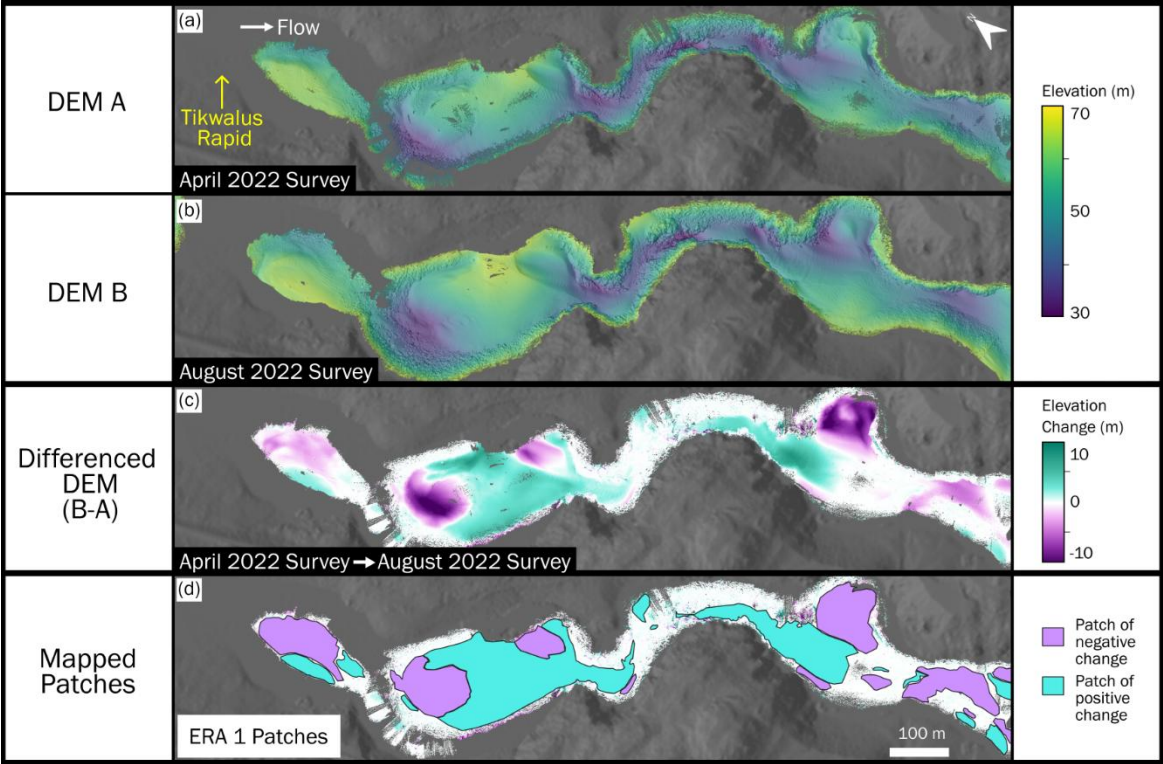
Figure 3. Visualization of the change detection workflow using repeat surveys at Tikwalus Rapid over Era 1 as an example: (a) bathymetry at Tikwalus Rapids in April 2022; (b) bathymetry at Tikwalus Rapid in August 2022; (c) elevation differences between the two surveys representing change in Era 1 through the 2022 freshet; (d) manually mapped patches of change from Era 1 at Tikwalus Rapid.
