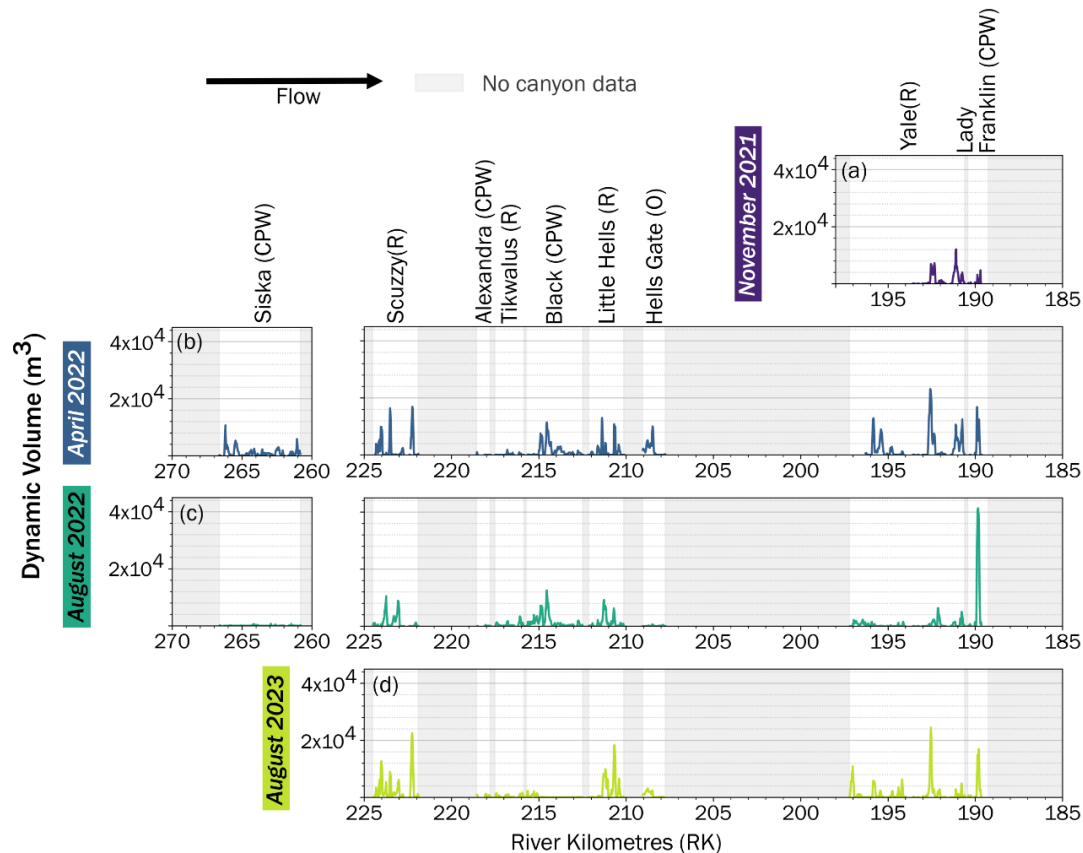
Figure 7. Dynamic sediment storage volume, calculated as difference from minimum elevation observed over all surveys for each canyon and Era surveyed. Canyon survey locations are plotted along river kilometers. Volume is summed over 20 m longitudinal increments. In brackets after canyon names their morphology is noted (“CPW” for constriction-pool-widenings, “R” for rapids, and “O” for the overfall).
