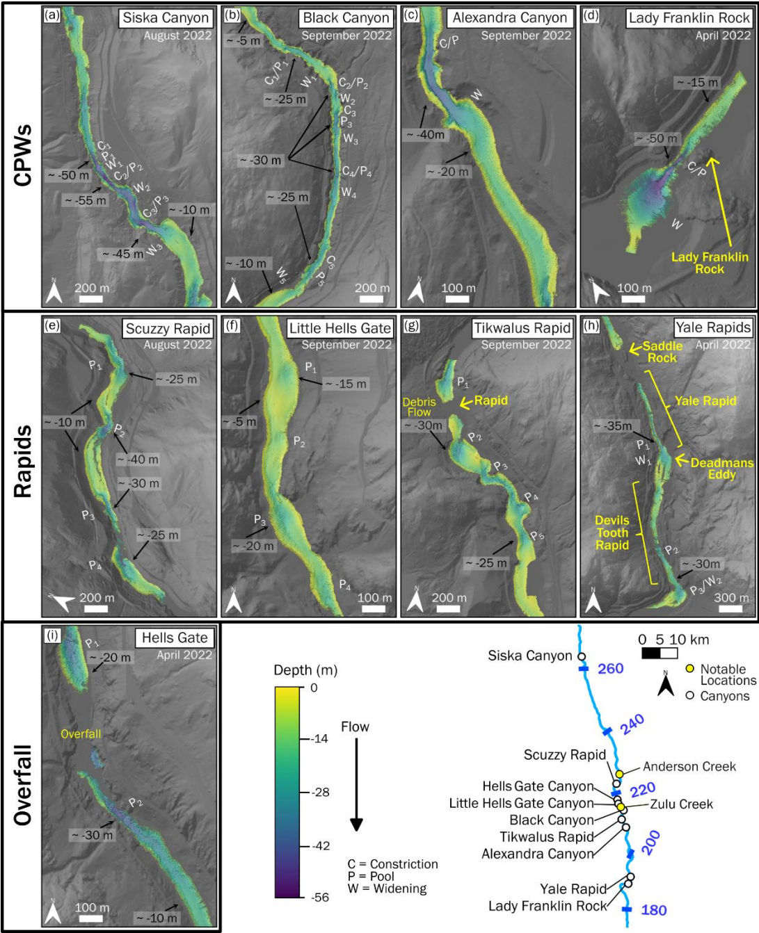
Figure 4. Canyon bathymetry as depth below water surface at sites with repeat surveys. Reaches are categorized based on morphodynamic type. Approximate depth values are labelled at select locations with notable features. Prominent morphologic features are labelled as well. Streamwise positions are mapped. See supplement for bathymetric maps of all surveys.
