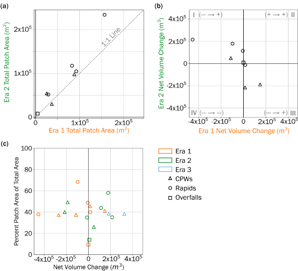
Figure 11. (a) Comparison of total patch area mapped within each canyon over Era 1 and 2. All canyons with surveys bracketing both Eras were plotted (Siska Canyon therefore excluded). The dashed line indicates 1:1. (b) Comparison of net volume change within each canyon over Era 1 and 2 (again, Siska Canyon therefore excluded). Quadrants I and III indicate a shift between deposition and erosion for canyons depending on the Era. Quadrants II and IV indicate a consistent direction of change over both Eras. (c) Plot of the percentage of patch area of the total survey area against the net volume change observed for each canyon in each Era.
