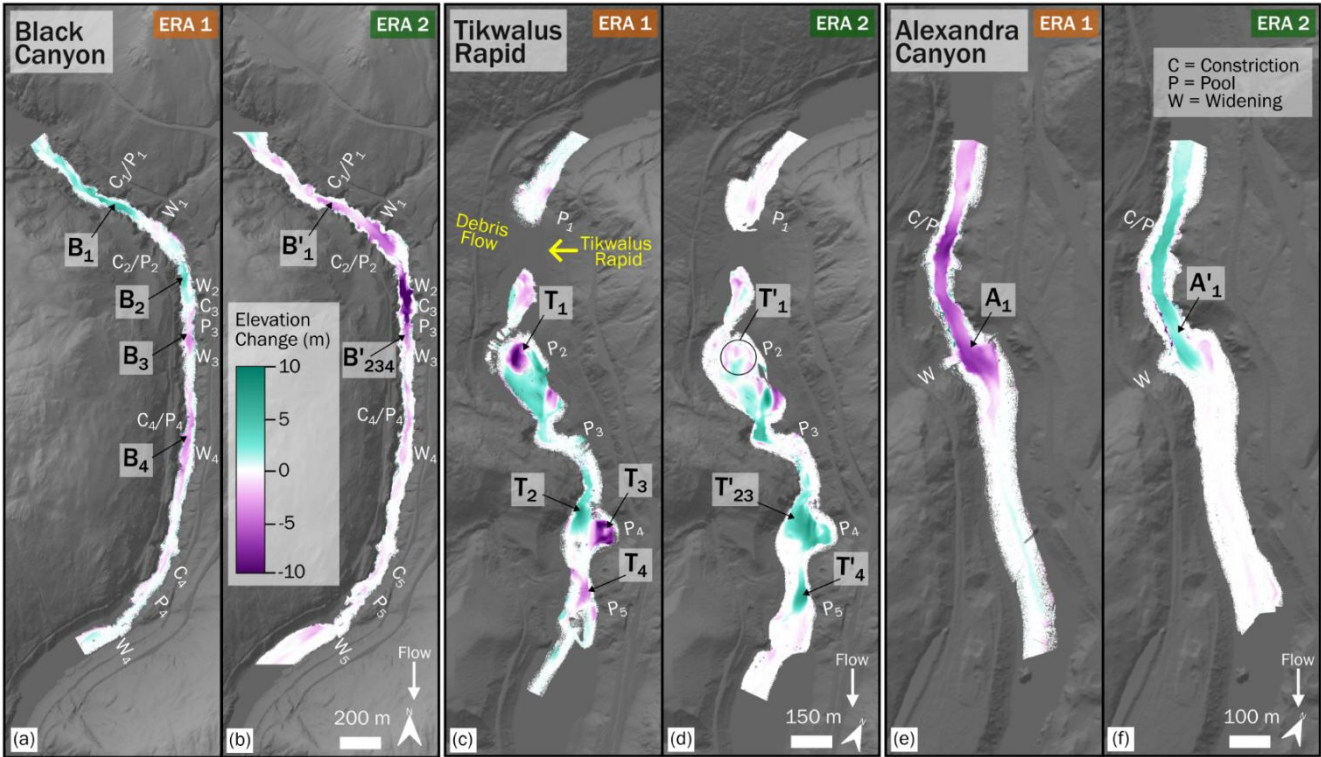
Figure 8. Elevation changes at Black Canyon, Tikwalus Rapid, and Alexandra Canyon for Era 1 and Era 2. Prominent morphological features are labeled. Patches discussed in text are labeled with the first letter of the canyon name, and a numbered subscript for identification, while prime notation is used to distinguish between Eras.
