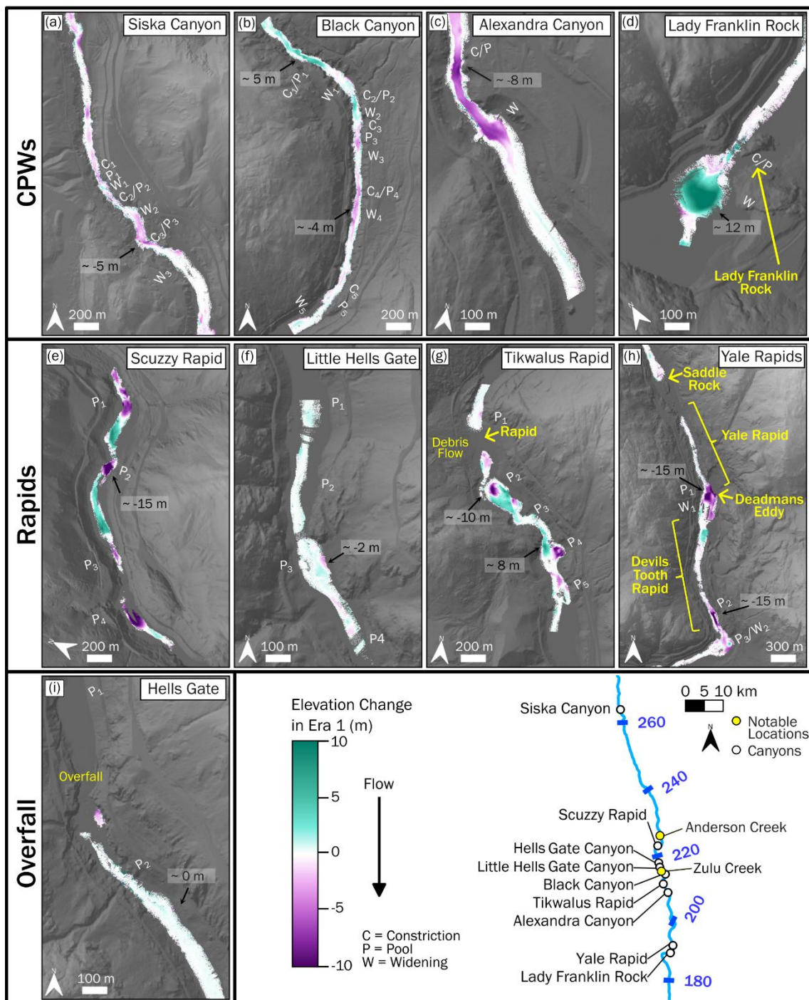
Figure 6. Change in elevation during Era 1 at all sites, with regions of deposition represented by positive change, and erosion by negative change. Approximate elevation change values are labelled at select locations with notable features. Prominent morphologic features labelled in Figure 5 are also visible. Streamwise positions are mapped. See supplement for maps of change in bathymetry over all the Eras.
