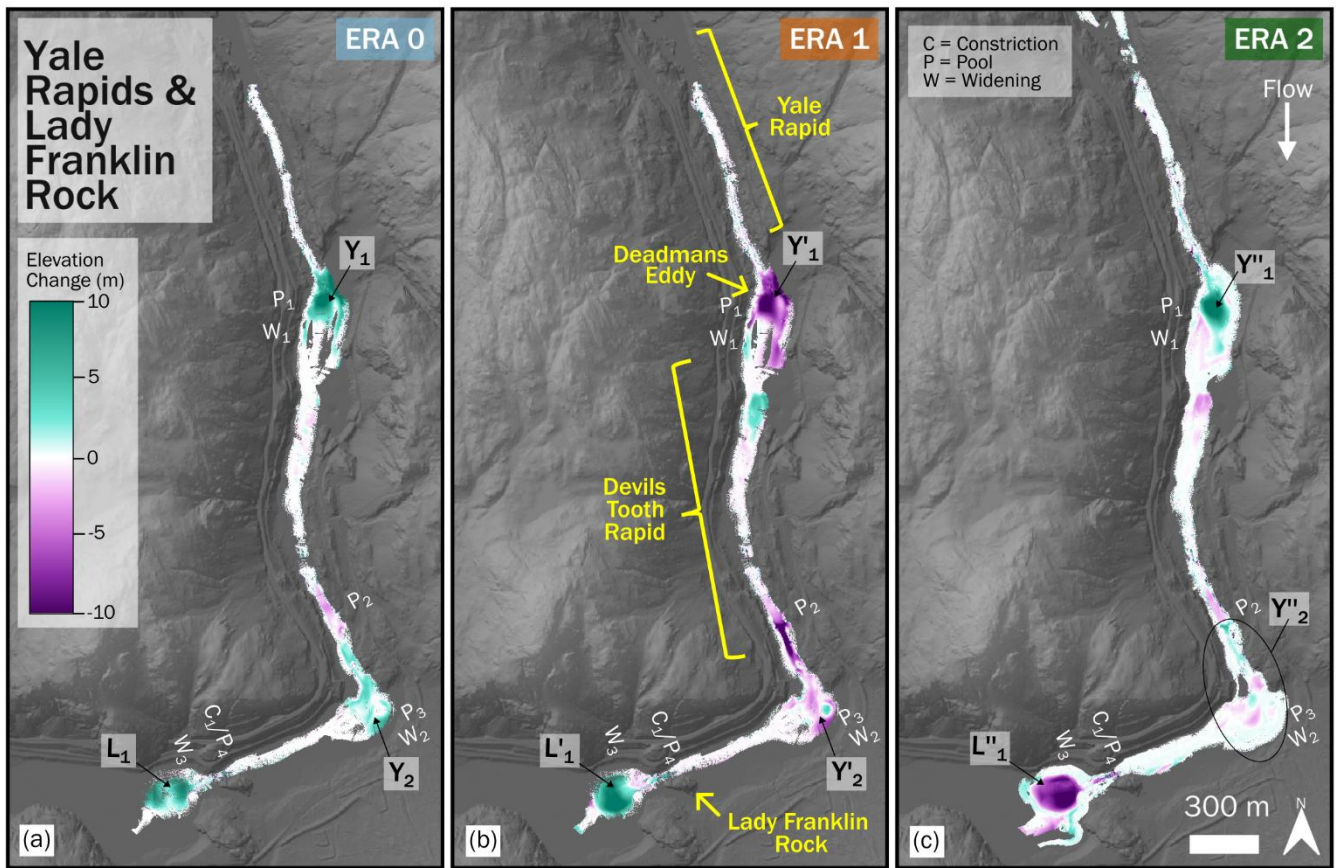
Figure 9. Elevation changes at Yale Rapids and Lady Franklin Rock for Era 0, Era 1 and Era 2. Prominent morphological features are labeled. Patches discussed in text are labeled with the first letter of the canyon name, and a numbered subscript for identification, while prime notation is used to distinguish between Eras.
