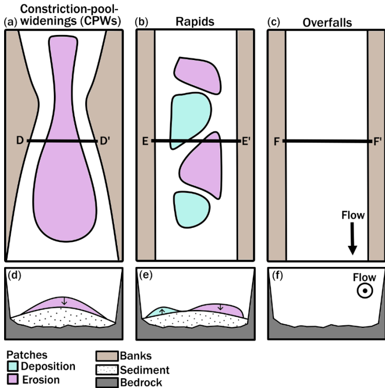
Figure 12. Cartoon of general patterns of elevation change observed at each morphology. Planform view of patch patterns for (a) CPWs, (b) rapids, and (c) overfalls is simplified based on observations for comparison of general patterns. Additionally, simplified cross sectional views of patch dynamics are shown in (d) for typical CPW morphology (although change may be erosional or depositional), (e) for potential rapid morphology, and (f) for likely overfall morphology based on observations.
