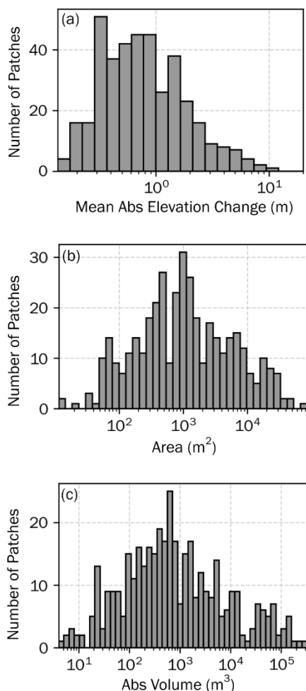
Figure 5. Distribution of mapped patches from all Eras, morphodynamic types, and directions of change based on patch (a) mean absolute elevation change, (b) area, and (c) absolute volume. See Table 2 for measured statistics.
