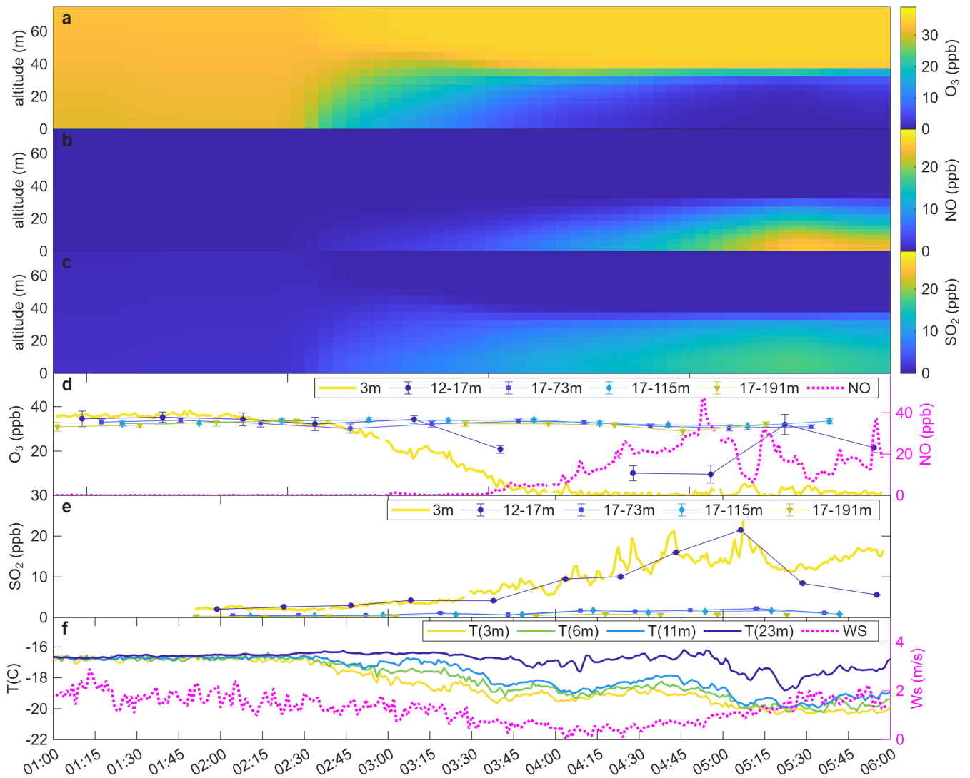
Figure 9. Formation of the PSL on February 4, 2022. The top three panels (a, b, and c) show the model results for this event. Panel d shows the path-averaged LP-DOAS and in-situ ozone data (left y-axis) and the surface NO data (magenta, right y-axis). The light path above 17 m height shows a constant O_3 mixing ratio of \sim 35 ppb, while the PSL mixing ratios drop at the onset of the event at around 2:45. Panel e shows the observations of SO_2 for LP-DOAS and in-situ data. The PSL observations of the two instruments agree very well, and also show an increase in SO_2 during this event. Temperature gradients (panel f, left y-axis) form around 2:15, during a time when the wind speed (magenta, right y-axis) is around 2 m/s.
