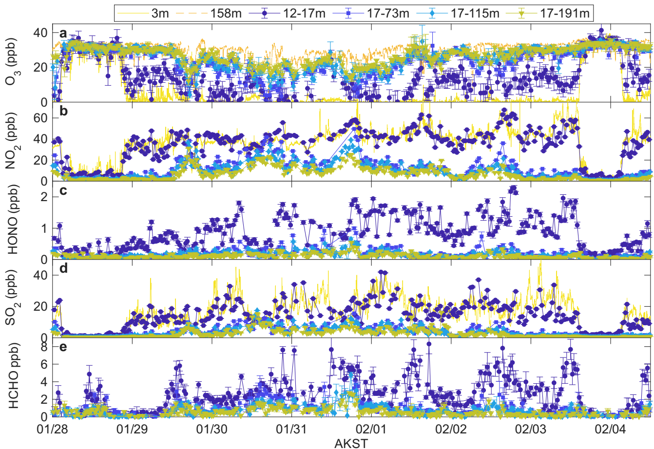
Figure 2. Overview of one week of path-averaged LP-DOAS data along the four different lightpaths using the same color coding as in Figure 1. Surface (3 m) in-situ data is shown as a yellow line, while the Birch Hill data (158 m) is shown as a dashed dark yellow line. The full dataset is shown in Figure S1.
