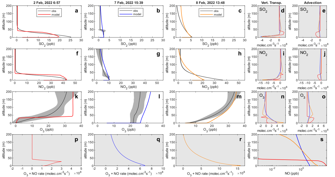
Figure 8. Examples of retrieved and modeled vertical mixing ratio profiles of SO 2 , NO 2 , and O 3 . The shaded area shows the profile uncertainty due to the measurement error. Shaded panels on the right depict the modeled vertical and advective transport rates of SO 2 (d,e), NO 2 (i,j), and O 3 (n,o). The bottom three panels (p,q,r) show the vertical profiles of the O 3 + NO reaction rate for the three examples, where the respective NO vertical profiles from the model are shown in panel (s).
