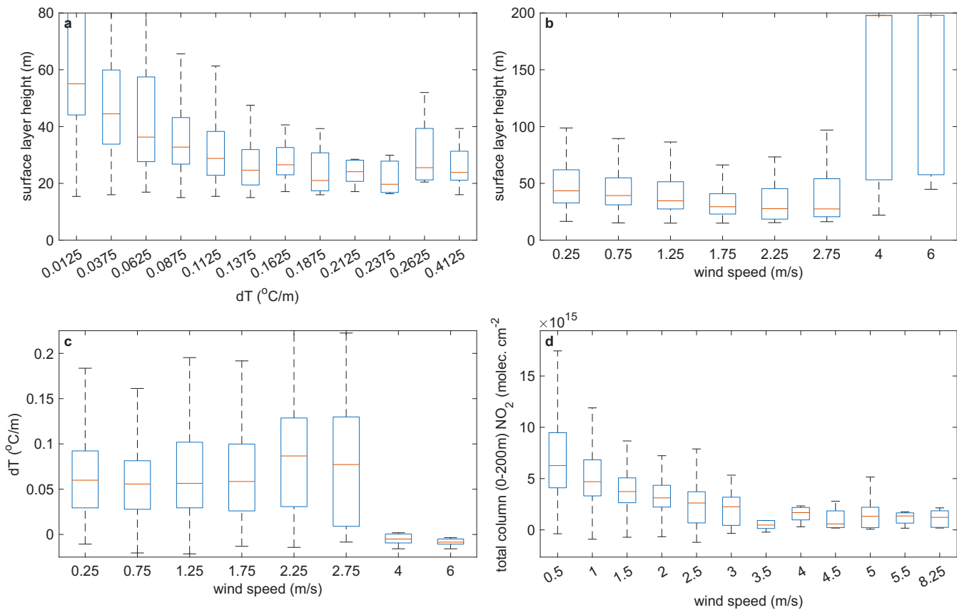
Figure 4. Statistical analysis of the dependence of (a) surface layer height on temperature gradient; (b) surface layer height on 23 m wind speed; (c) surface temperature gradient on 23 m wind speed, and (d) NO 2 column density on wind speed.
