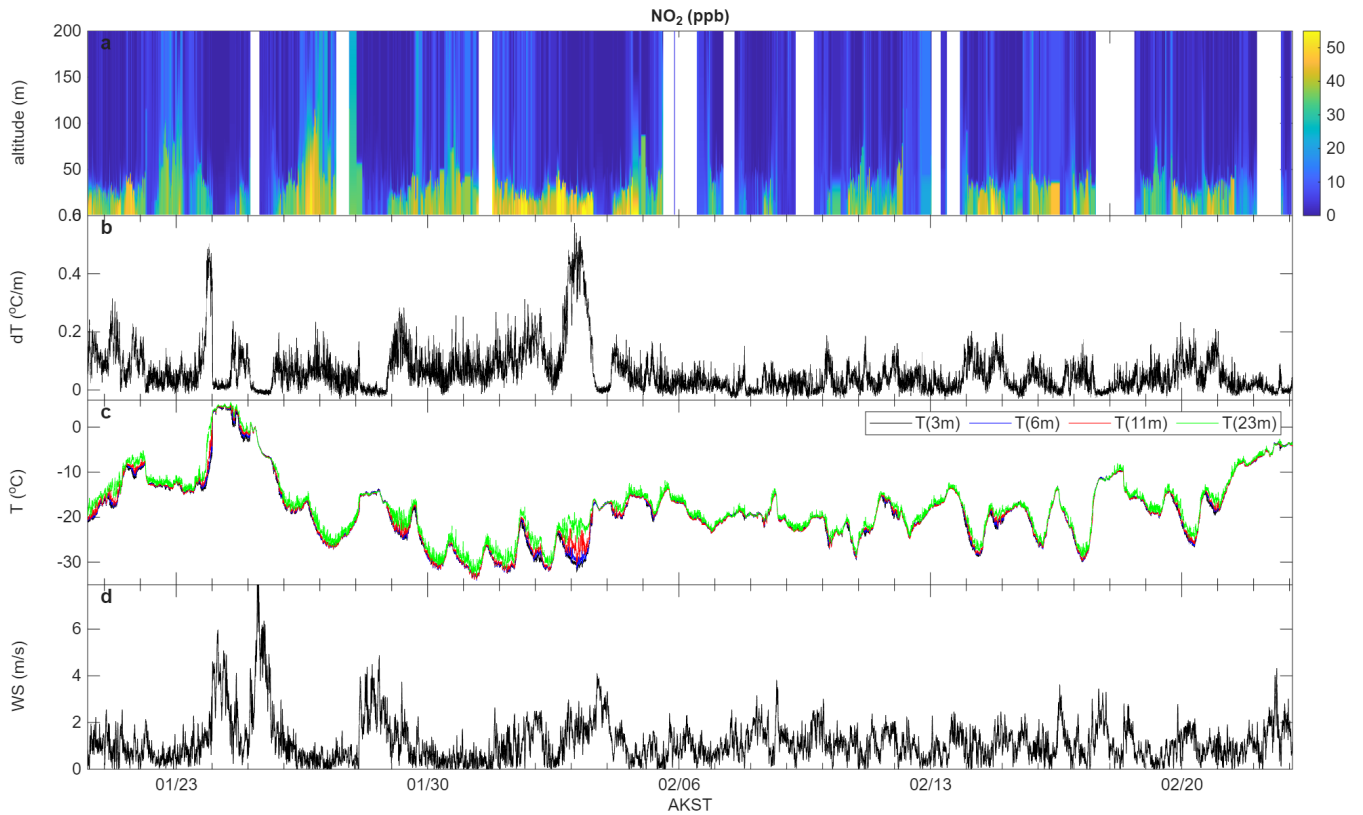
Figure 3. Retrieved vertical profiles of NO 2 (a) compared to temperatures at 3, 6, 11, and 23m (c) and temperature gradients gradients (b). Wind speeds at 23 m are displayed in panel (d).
