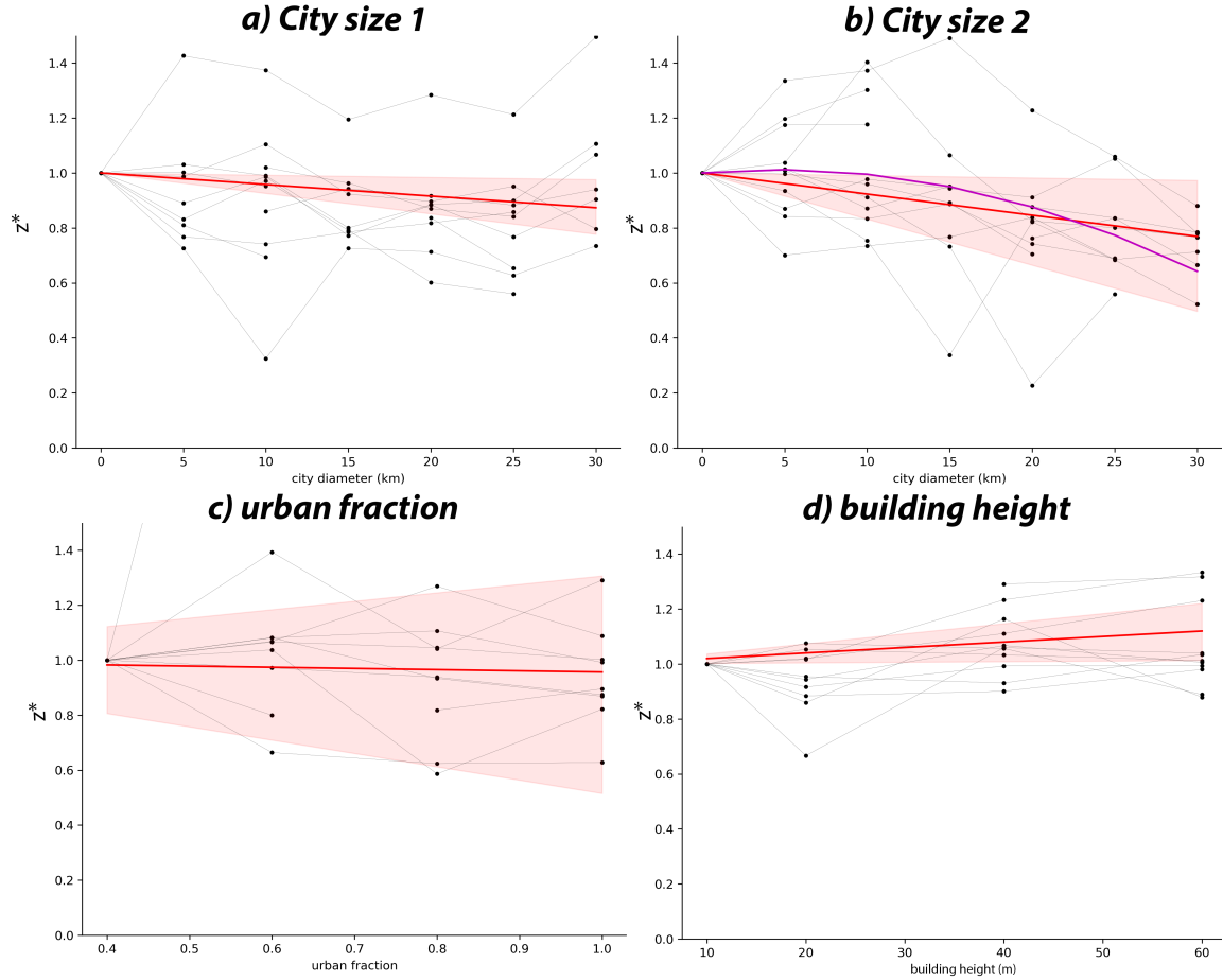
Figure 5. a) Normalized mean UH ( z^* ) in each ensemble member (black dots) of the city size 1 set of experiments (Table 4) in function of the city diameter (km) in the city region . Ensemble members obtained with the same seed are connected. The mean linear fit is shown with a red line, while the 5-95% confidence interval is red shaded. b), c) and d) as in a) but for the city size 2 , urban fraction and building height set of experiments, respectively. In b), a quadratic fit is shown with a purple line.
