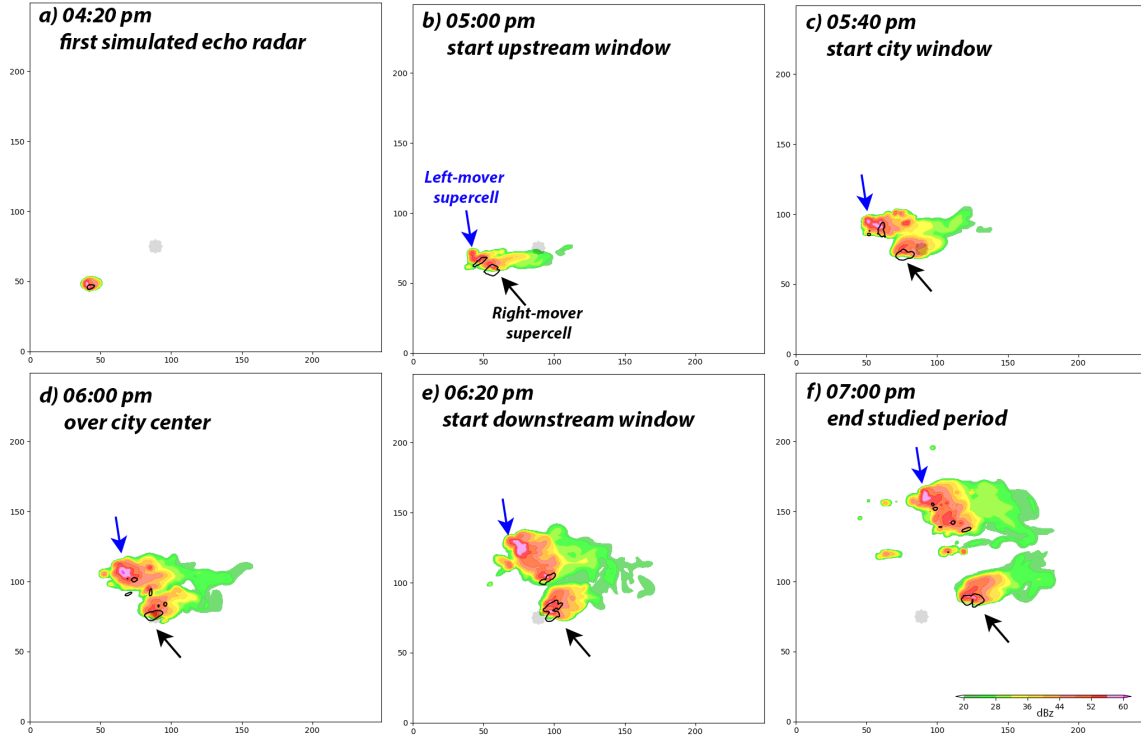
Figure 3. Maximum simulated reflectivity (colour shading) at a) 04:20 pm, b) 05:00 pm, c) 05:40 pm, d) 06:00 pm, e) 06:20 pm, f) 07:00 pm by the control run of numerical experiment 10km_1 . The city is shown with a grey shading. UH value higher than 100 \text{ m s}^{-1} are highlighted with a black contour. The black (blue) arrow indicates the right-mover (left-mover) supercell.
