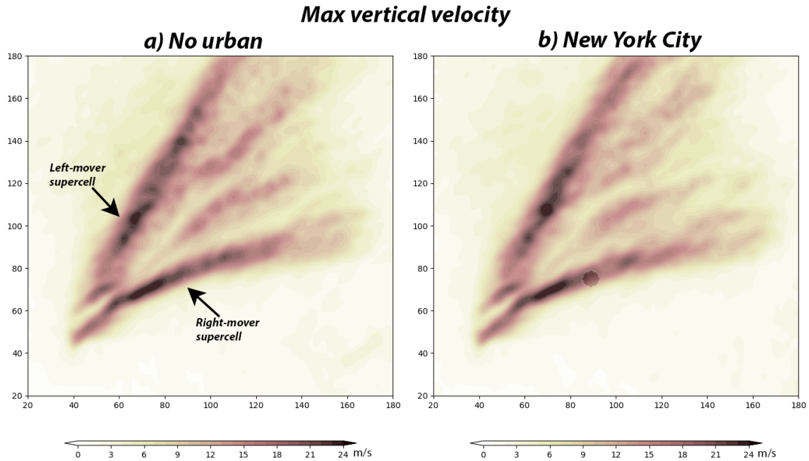
Figure 9. Ensemble mean of cumulated maximum vertical velocities in the a) no_urban and b) NYC experiment (Table 3). The city location is shown with a grey circular shading in b).
