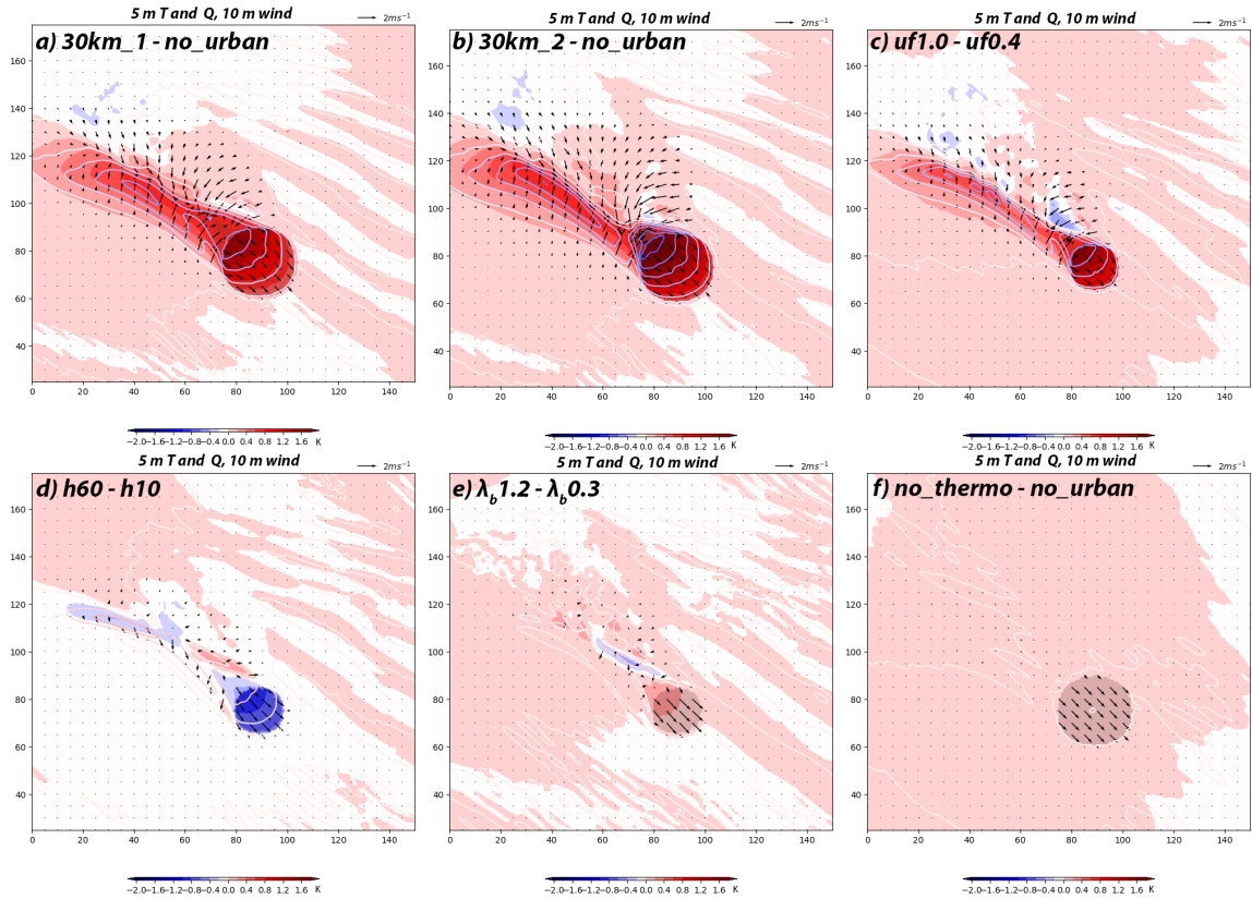
Figure 10. Ensemble mean of temperature (color shading) and specific humidity (contours every 0.5 \text{ g kg}^{-1} , blue negative, red positive) in the first model level (about 5 m AGL), and 10-m wind difference (vectors) at 04:00 pm between a) 30km_1 and no_urban experiments; b) 30km_2 and no_urban experiments; c) uf1.0 and uf0.4 experiments; d) h60 and h10 experiments; e) \lambda_b 1.2 and \lambda_b 0.3 experiments; f) green roofs and no_urban experiment. The city is shown with grey shading.
