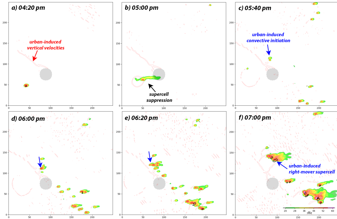
Figure 7. As in Fig. 3, but for the ensemble member 1 of the 30km_2 numerical experiment. Vertical velocities at 950 hPa higher than 0.5 \text{ m s}^{-1} are plotted with red contours. The blue arrows indicate the triggering of the urban-induced right-mover supercell.
