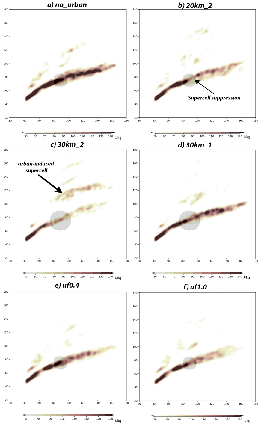
Figure 6. Cumulated UH ensemble mean in a) the no_urban experiment (Table 5), b) in the 20km_2 experiment, c) in the 30km_2 experiment, d) in the 30km_1 experiment (Table 4), e) in the uf0.4 experiment (Table 6), f) in the uf1.0 experiment. The city is highlighted in grey shading. In a) the city of the 20km experiment is shown just for reference, in the experiment there are croplands everywhere.
