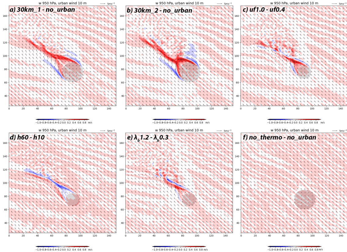
Figure 14. As in Fig. 11, but for vertical velocities at 950 hPa.
