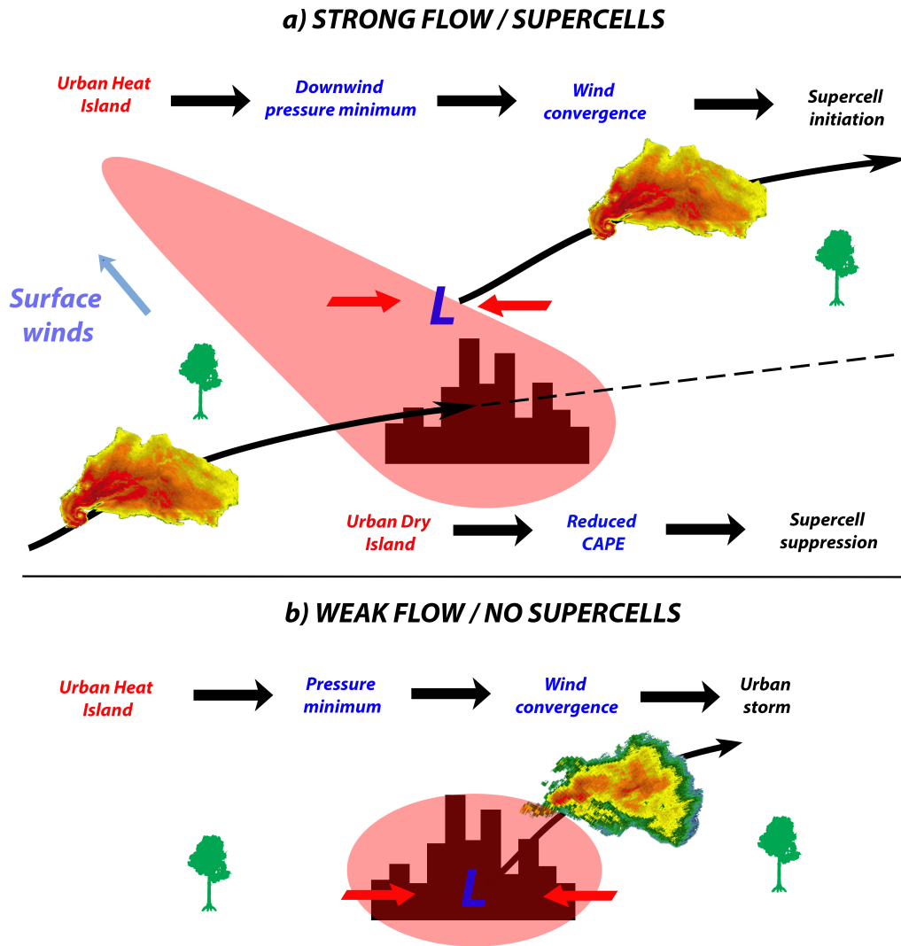
Figure 16. a) Summary of the results obtained in this study regarding the interaction between supercell storms and a city: the UHI and UDI (red shading), city (black histogram), supercell (yellowish-reddish shading with hook-echo shape), pressure minimum (letter L) and wind convergence (red arrows) are shown. b) as in a), but for a weak flow situation without supercells.
