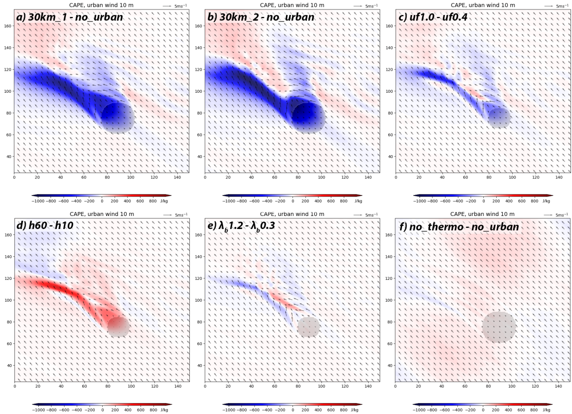
Figure 13. As in Fig. 11, but for CAPE.
