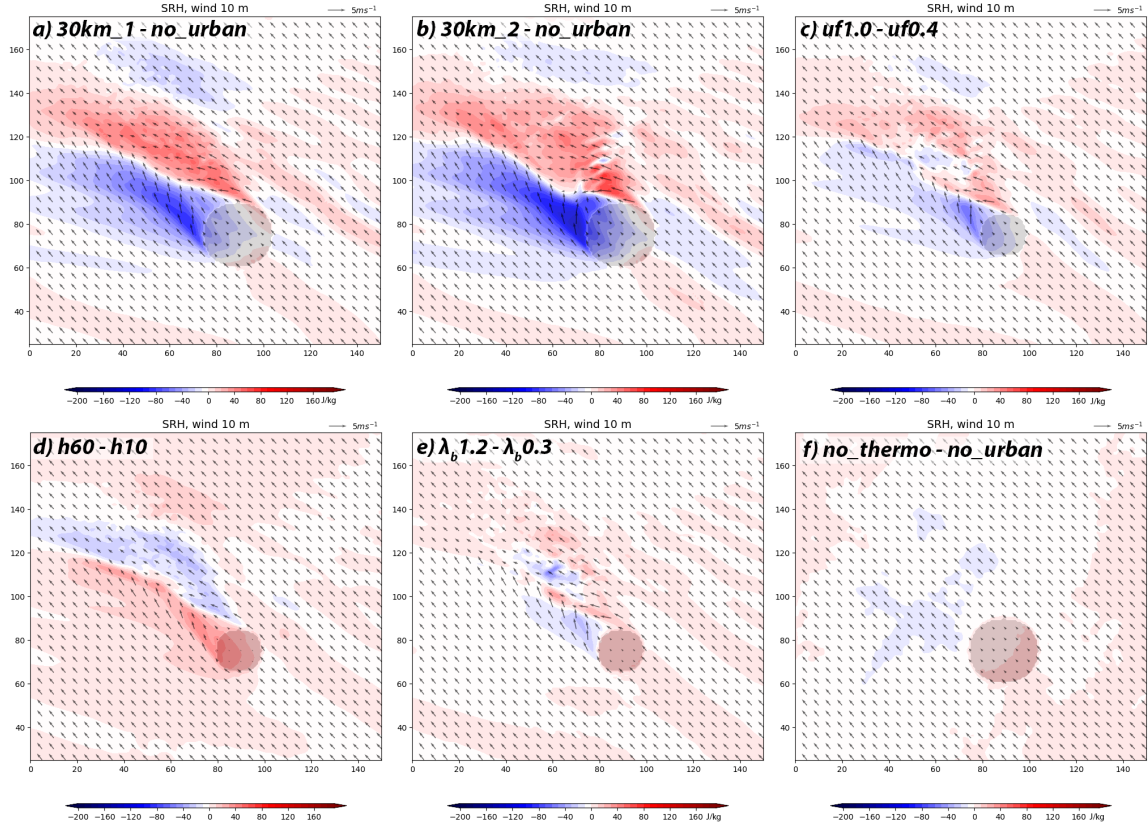
Figure 15. As in Fig. 11 but for SRH 0-3 km.
