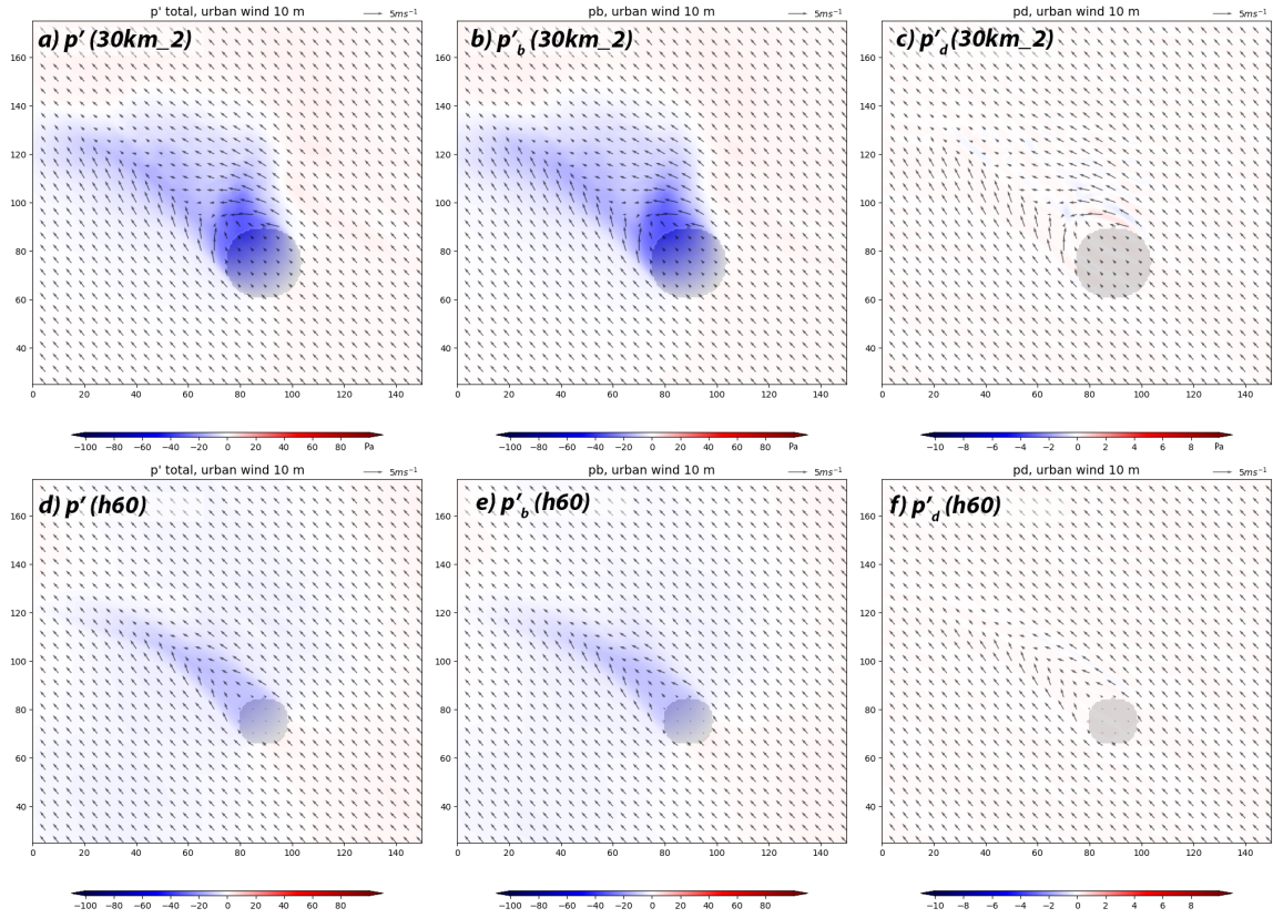
Figure 12. Ensemble mean of a) total pressure perturbations p' at 300m AGL in the 30km_2 experiment at 04:00 pm; b) as in a) but for buoyancy pressure perturbations p'_b ; c) as in b) but for dynamic pressure perturbations p'_d ; d), e) and f) as in a), b) and c), respectively, but for the h60 experiment.
