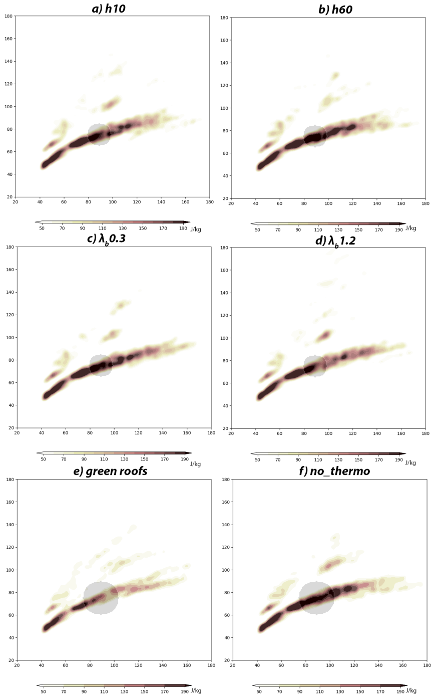
Figure 8. As in Fig. 6, but for a) h10 experiment (Table 7), b) h60 experiment, c) \lambda_b 0.3 experiment (Table 7), d) \lambda_b 1.2 experiment, e) green roofs experiment (Table 3) and f) no_thermo experiment (Table 3).
