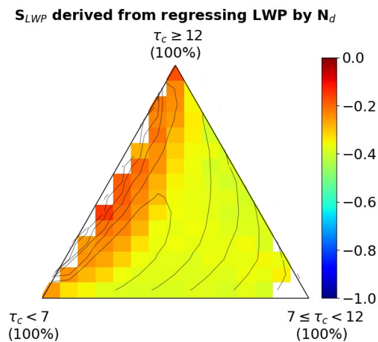
Figure A2. LWP susceptibility derived from the regression between \ln\text{LWP} and \ln N_d within each ternary bin. Contours represent scene occurrence, as in Figure 2b.
