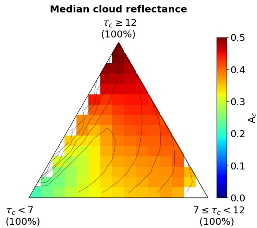
Figure A3. Median ternary-bin values of A_c . Contours indicate scene occurrence, as in Figure 2b.
