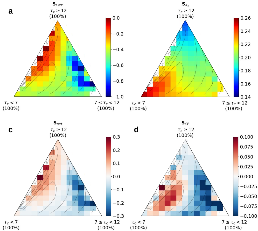
Figure 4. Cloud albedo susceptibility to N_d for (a) LWP, (b) A_c (Twomey effect), (c) net cloud albedo, and (d) CF. Contours represent scene occurrence, as in Figure 2b.
