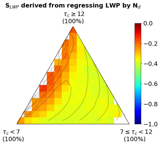
Figure A2. LWP susceptibility derived from the regression between \ln LWP and \ln N_d within each ternary bin. Contours represent scene occurrence (as in Figure 2a ) .
