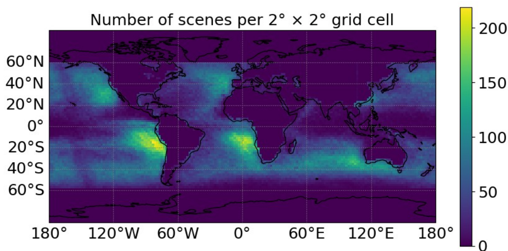
Figure A1. Number of scenes per 2° × 2° grid cell used in the analysis. It can be seen that most scenes derive from the stratocumulus regions in the eastern subtropical oceans.
