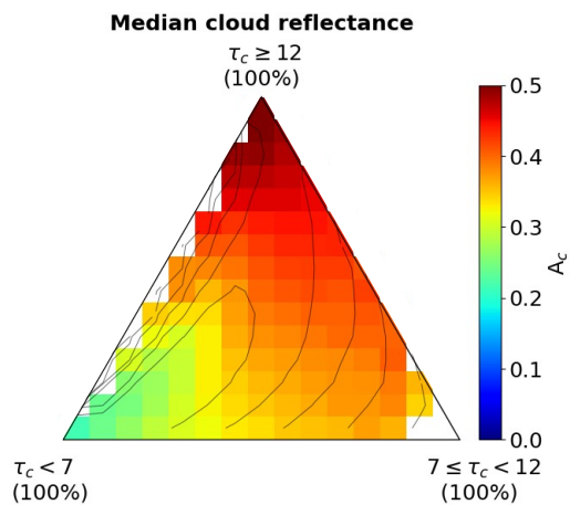
Figure A3. Median ternary-bin values of cloud reflectance at 0.84 \mu\text{m} A_c . Contours indicate scene occurrence (as in Figure 2 ) .
