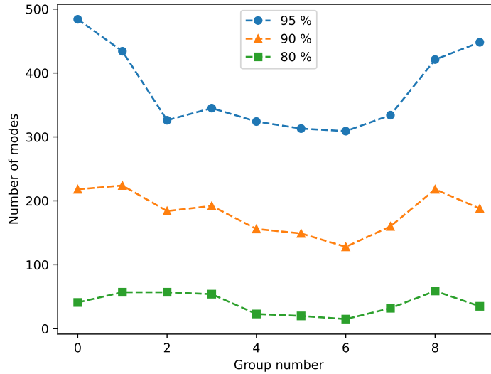
Figure 9. Percentage of variability explained by a reduced number of modes. Generally, a relatively low number of PCs is needed to reconstruct most of the spectrum variability. Higher number of components is needed in the mid-latitudes.
