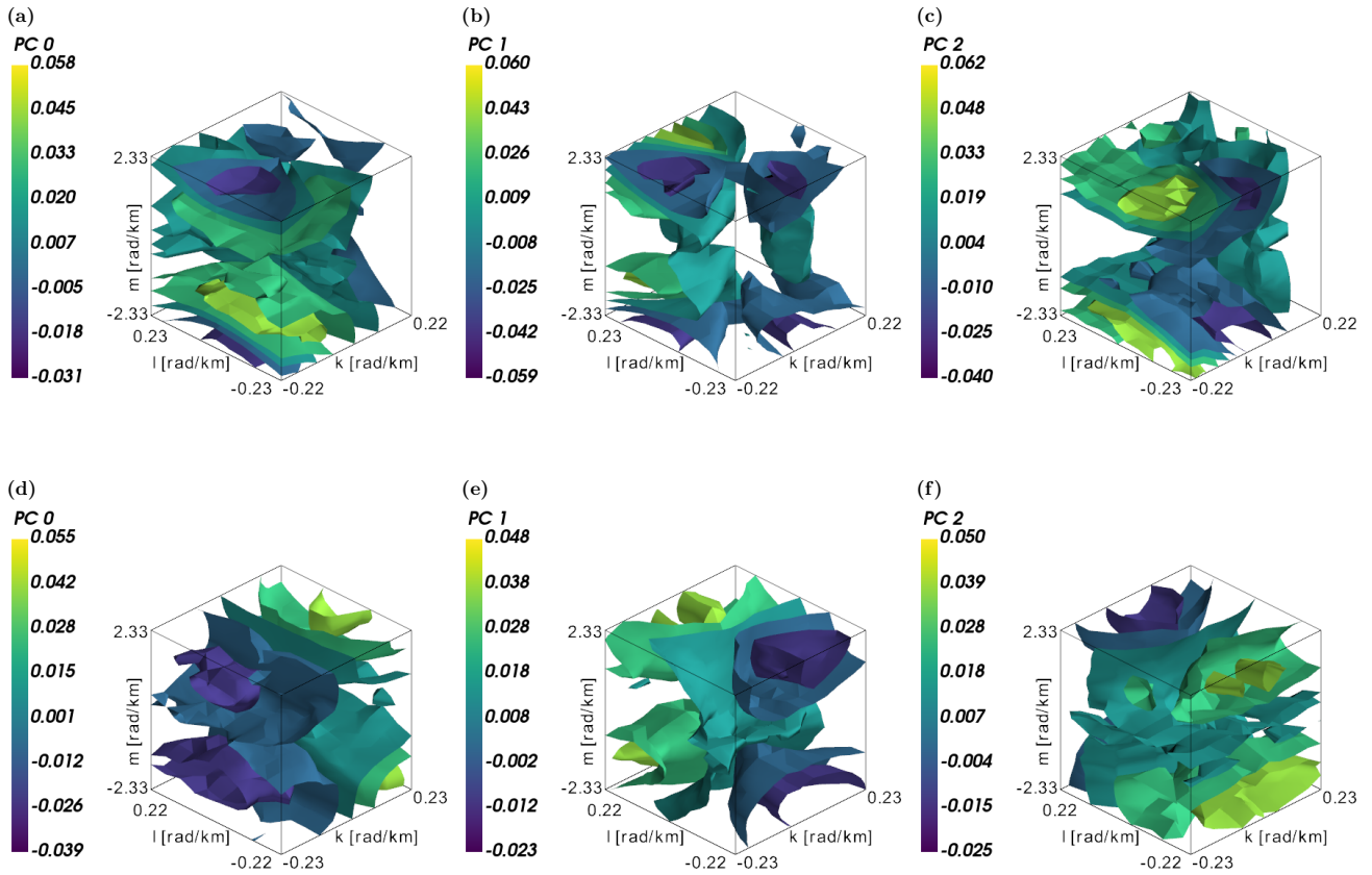
Figure 8. Principal Individual principal components 0,1 and 2 (columns) of wave action density in groups 1 (top) and 4 (bottom). The first few components mainly estimate the major structure in zonal, meridional and vertical directions, which is notable-noticeable especially for group 4.
