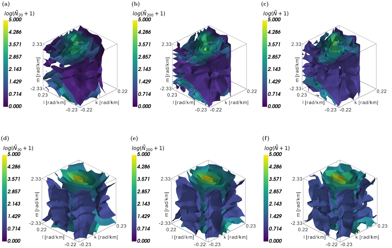
Figure 10. Representation of a random single spectrum ( right third column ) from groups 1 (top) and 4 (bottom) by 20 (first column) and 200 PCs (second column). With the 200 components, the main structure of the 3D spectrum is well represented, especially for the more symmetric case of group 4.
