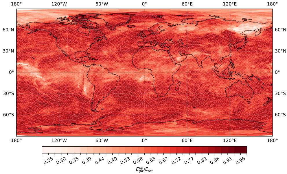
Figure 5. Global distribution Percentage of the GW upward propagating waves on 23 January 2020. (a) Total energy of GW spectra 2020, visualising particularly GW hotspots above orography, and also weaker GW signal in mid-latitudes and above described by the equator. (b) Fraction between the projected GW part and the 3D spectrum of total energy, describing the effect of GW projection compared to simple removal of larger scales GWs.
