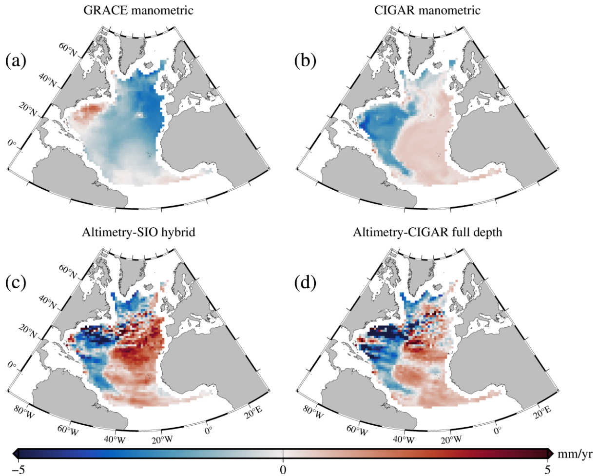
Figure 4. Manometric sea level trends in the North Atlantic over 2004.01-2022.12 derived from (a) the mean of three GRACE mascon solutions, (b) the CIGAR ocean reanalysis, (c) 'Altimetry minus SIO hybrid' and (d) 'Altimetry minus CIGAR full depth'.
