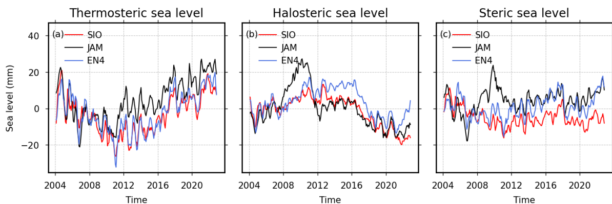
Figure 3. Upper ocean time series of thermosteric (a), halosteric (b), and steric (c) sea level time series in the North Atlantic derived from Argo products (SIO, JAMSTEC, EN4). All-time series have applied three-month moving average filtering.
