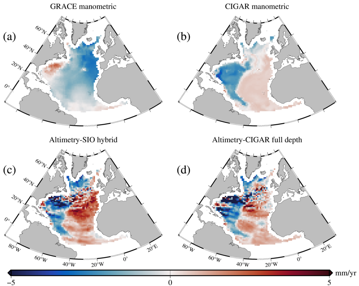
386 Figure 4. Manometric sea level trends in the North Atlantic over 2004.01-2022.12 derived from 387 (a) the mean of three GRACE mascon solutions, (b) the CIGAR ocean reanalysis, (c) ‘Altimetry 388 minus SIO hybrid’ and (d) ‘Altimetry minus CIGAR full depth’.
