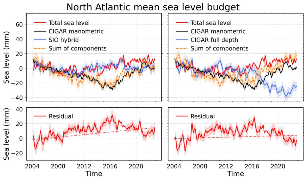
443 Figure 6. Time series of North Atlantic sea level change components (top) and budget residuals 444 (bottom). The left panels use the SIO hybrid steric estimate ( SIO for 0–2000m combined with 445 CIGAR for 2000–6000m ), while the right panels use the full-depth CIGAR steric estimate ( full- 446 depth ). In both left and right panels, CIGAR manometric components are considered. All time 447 series have applied three-month moving average filtering . The global mean trend of each 448 component is removed. Shaded areas represent data uncertainties.
