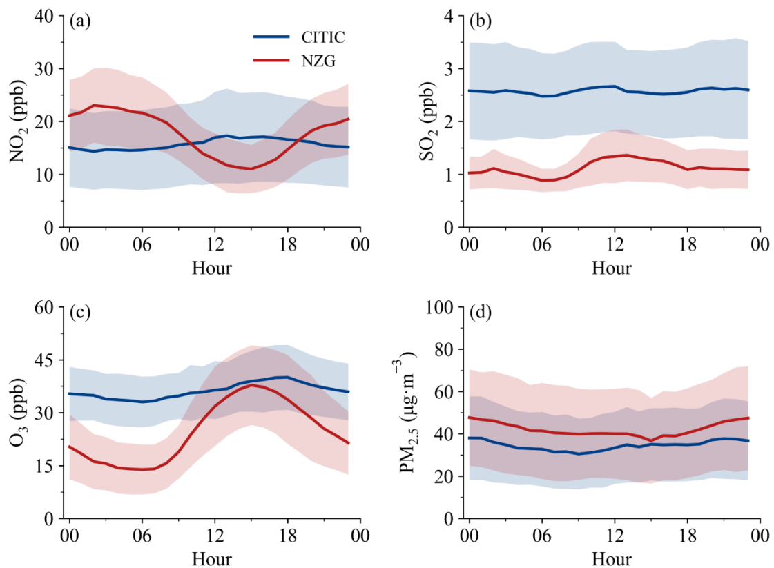
Figure 9. Diurnal variations of \text{NO}_2 , \text{SO}_2 , \text{O}_3 , and \text{PM}_{2.5} during observational period (2020-2024) at the CITIC (blue) and NZG (red) stations, respectively. The shaded areas denote 50% standard deviation.
