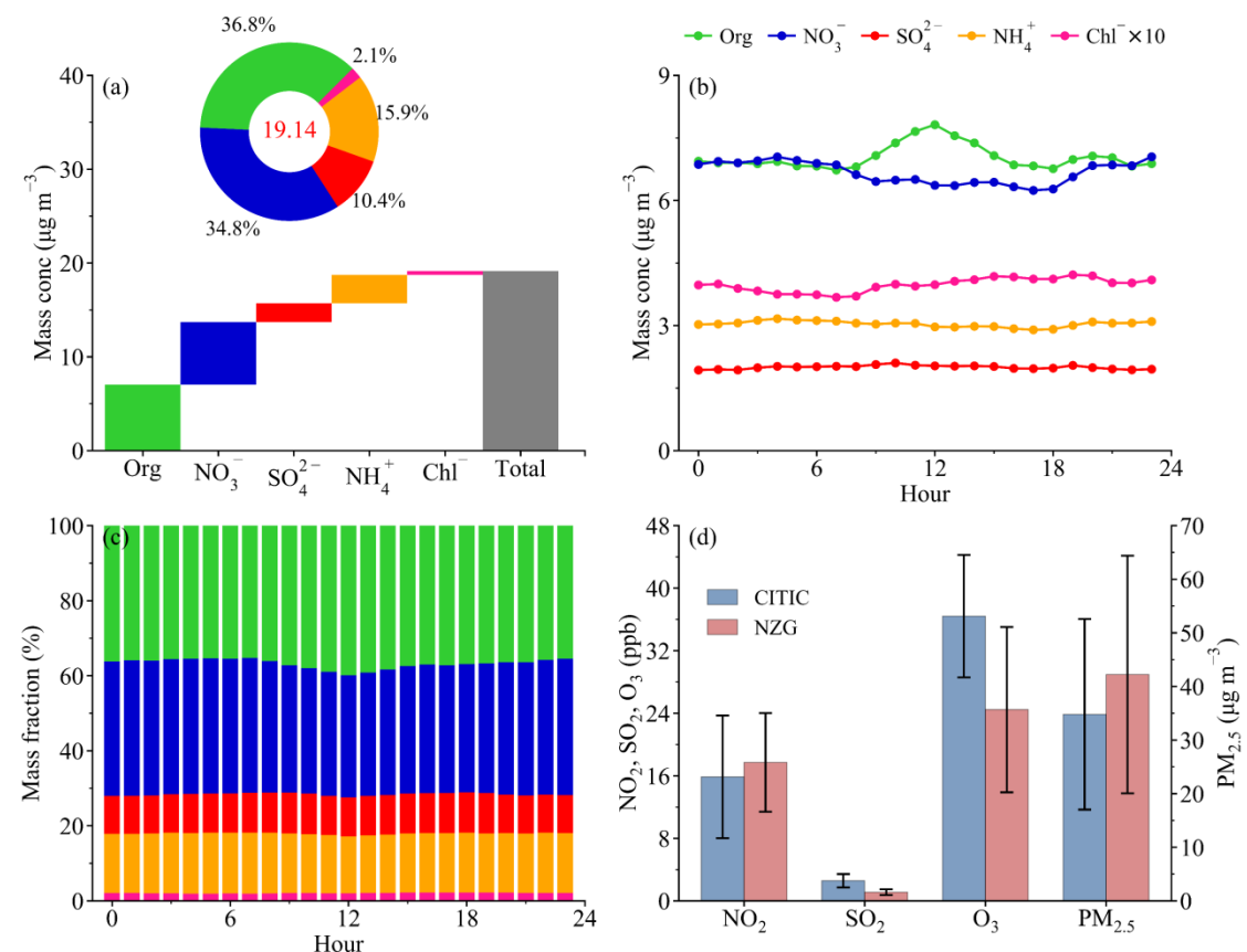
Figure 2. The mean mass concentration and aerosol composition of NR- \text{PM}_{2.5} observed at the CITIC station (a); diurnal variations of the mean mass concentration
