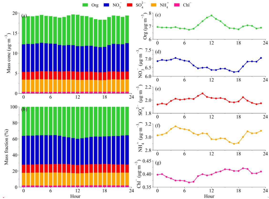
Figure 2. Diurnal variations of mass concentrations (a) and fraction (b) of NR- \text{PM}_{2.5} and each component (c-g) during observational period (2020-2024).
