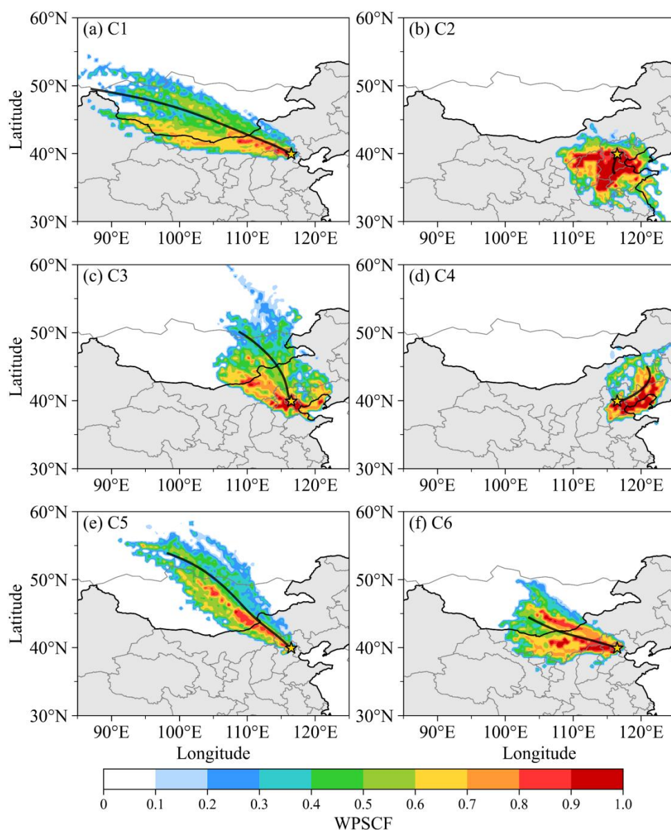
Figure 4. Potential source contribution at altitude of 500 m over Beijing in the six clusters. The WPSCF represents weighted potential source contribution function.
