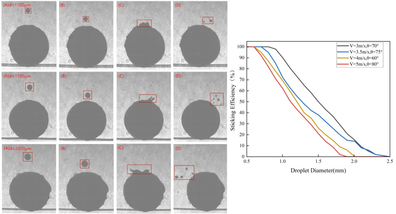
Figure 7: Variation in experimentally measured sticking efficiency with droplet diameter.
