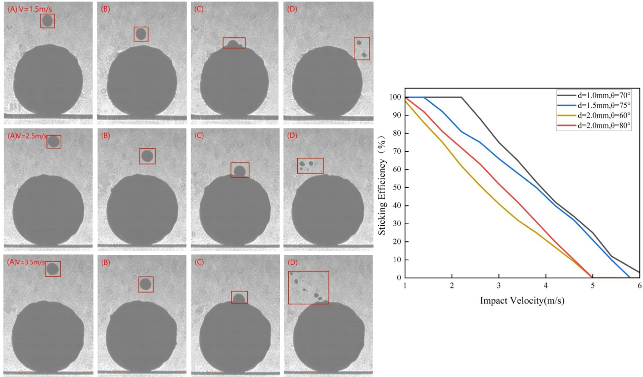
Figure 6: Variation in experimentally measured sticking efficiency with impact velocity.
