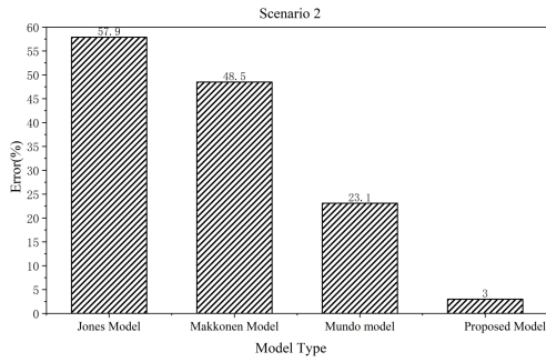
Figure 10: Comparison of sticking efficiency prediction errors for actual case 2.
