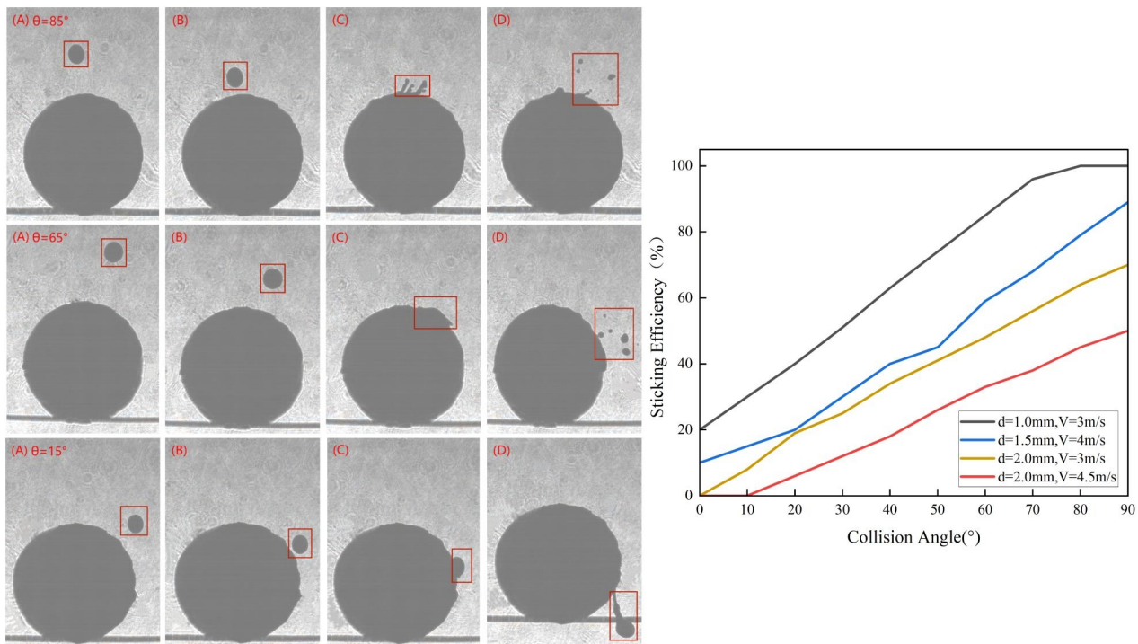
Figure 5: Variation in experimentally measured sticking efficiency under different collision angles.
