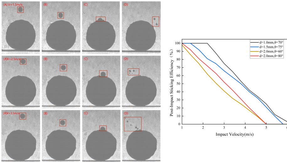
Figure 6: Effect of impact velocity on experimentally measured post-impact sticking efficiency. Representative impact images and the retained-fraction curve are shown.
