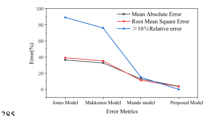
285 Figure 8: Sticking efficiency results calculated by various models using the laboratory data.
