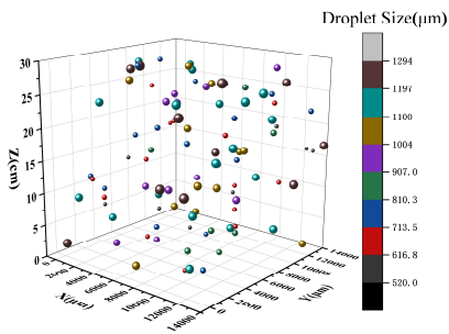
155 Figure 2: Reconstructed three-dimensional spatial distribution of droplets.
