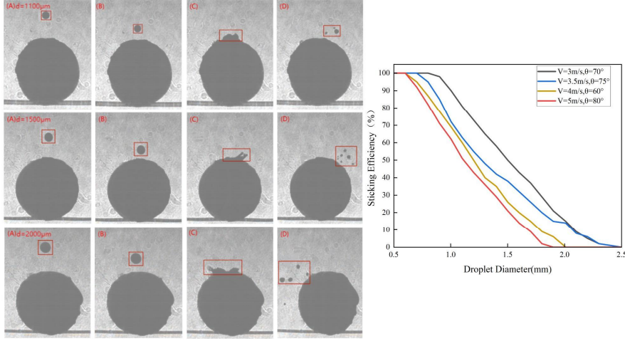
205 Figure 7: Variation in experimentally measured sticking efficiency with droplet diameter.
