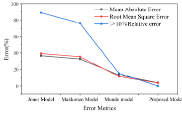
Figure 8: Sticking efficiency results calculated by various models using the laboratory data.
