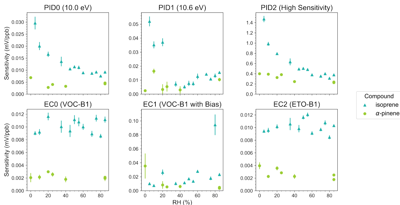
Figure 5: Sensitivities (in mV/ppb) of 3 PIDs (top row) and 3 EC sensors (bottom row) to isoprene and \alpha -pinene as a function of RH. Vertical bars denote 1\sigma confidence intervals. Note that each panel features a different y-axis.
