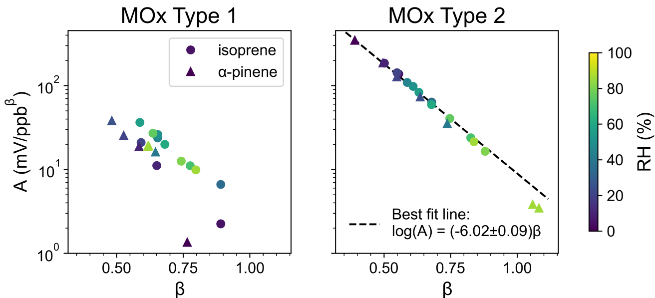
Figure 6: MOx responses to isoprene (circles) and \alpha -pinene (triangles), plotted in the parameter space of the power-law parameter. The dotted black line gives the best fit line for all data measured for MOx Type 2.
