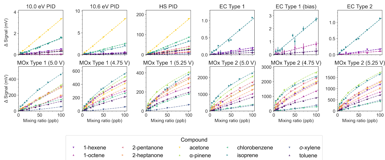
260 Figure 3: Summary of sensor responses (in mV over baseline) to various VOC mixing ratios between 5-100 ppb at 30% RH. Dotted lines represent the linear least-squares regression (PID and EC) or the power-law fit (MOx) of the measured values, denoted by triangles. Note that y-axes are not shared across panels, reflecting the wide range of sensitivities across sensors. If a compound is missing from a sensor’s subplot, as is the case with EC sensors, it means that the sensor does not exhibit sensitivity to that compound above its baseline noise. Error bars denote the standard deviation of measurements taken for each data point.
