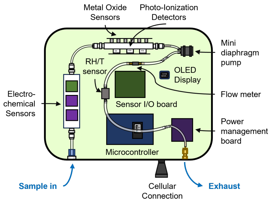
165 Figure 1: Schematic of the VOC air sensor array. Sample air is pulled in by a miniature diaphragm pump through custom flow cells that house 12 different VOC sensors. Several custom circuit boards manage power and sensor inputs/outputs.
