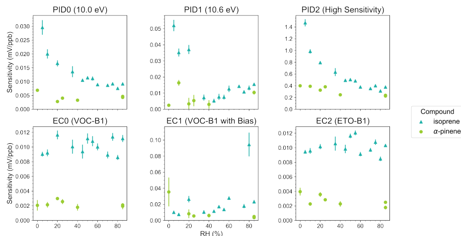
Figure 5: Sensitivities (in mV/ppb) of 3 PIDs (top row) and 3 EC sensors (bottom row) to isoprene and \alpha -pinene as a function of RH. Vertical bars denote 1 \sigma confidence intervals. Note that each panel features a different y-axis.
