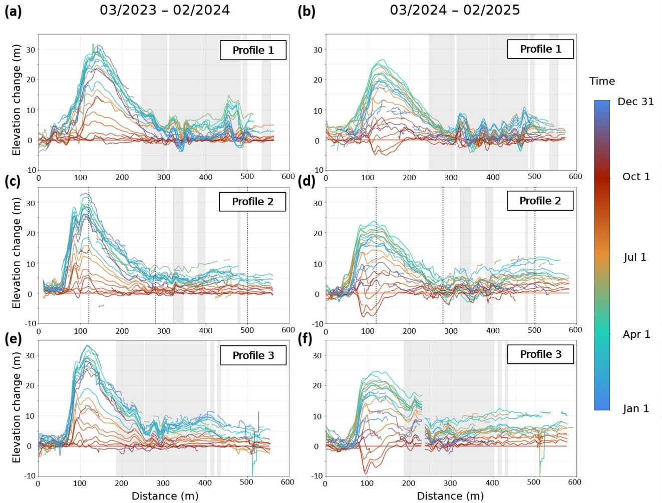
Figure 5: Elevation change between the time-lapse DEMs and a reference end-of-summer time-lapse DEM for the periods 03/2023 - 02/2024 (year 1; a, c, e) and 03/2024 - 02/2025 (year 2; b, d, f) along the profiles indicated in Fig. 4a. We used the 27/09/2023 time-lapse DEM as reference for year 1 and the 29/09/2024 time-lapse DEM for year 2. The shaded grey zones correspond to zones affected by crevasses during the study period. The vertical dashed lines correspond to the points used to plot the time series in Fig. 9.
