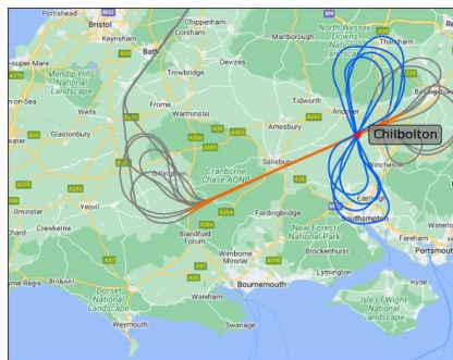
185 Figure 1 A typical CCREST-M flight track (shown as the grey, orange and blue colours) towards and over the Chilbolton- based triple-frequency radars. The figure-of-eight patterns (blue) were flown over Chilbolton when all the radars were pointing
