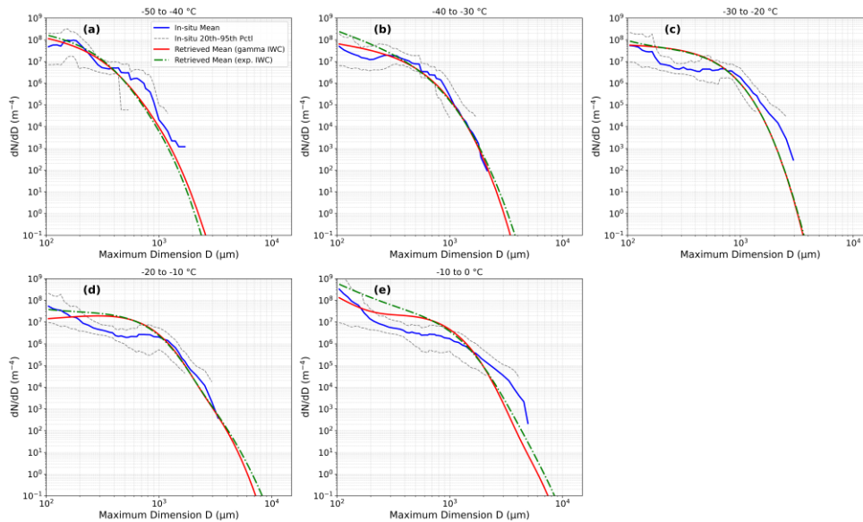
Figure 11 Comparison of retrieved and in-situ composite PSDs for flight C374 as a function of temperature. Retrieved mean PSDs assuming the gamma and exponential PSDs for the retrieval of the 3 GHz IWC are shown as red solid lines and green-dotted lines, respectively. The composite mean in-situ PSDs are shown as solid blue lines and the in-situ 20 th and 95 th
