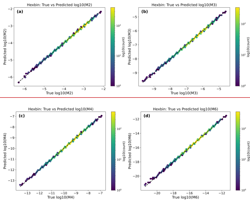
Figure 4 Hexagonally binned scatter plots of predicted versus true \log_{10}(M_n) from the ensemble of ML models for the PICASSO validation subset for (a) n=2 , (b) n=3 , (c) n=4 , and (d) n=6 . The colour scale shows the logarithm to the base 10 of the number of points in each of the hexagonal bins and the dashed line in each of the panels indicates the 1:1 line.
