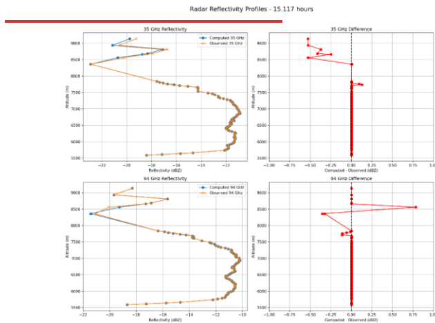
090 Figure 23 Same as Fig. 12, but for case C382 at the time of 15.117 hrs. Effects of a thin cirrus layer detached from the main ice-layer can be seen at altitudes between about 8.5 and 9 km.
