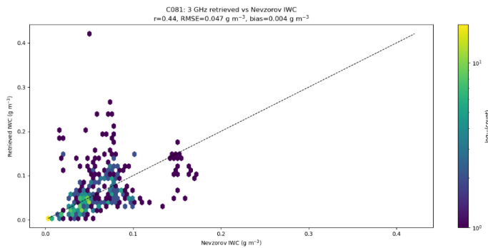
Figure 8 Hexagonally binned scatter plots of retrieved IWC from the 3 GHz radar plotted against in-situ Nevzorov-derived IWC for the PICASSO flight C081 and for altitudes greater than 3200 m. The colour scale on the right-side shows the \text{Log}_{10} of the number collocated samples per bin, with the dashed line indicating a slope of unity. The correlation coefficient, r , the root mean square error (RMSE) and the bias are shown at the top of the figure.
