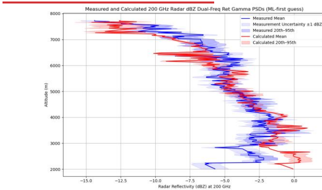
Figure 13 Comparison of the time-averaged forward model simulations (red lines and shade) assuming the retrieved PSDs and the gamma PSD for the retrieval of IWC at 3 GHz with the 200 GHz GRaCE radar observations (blue lines and shade). The key is shown in the top right of the figure.
