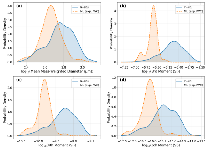
Figure 16 As Fig. 14, but for C382.
