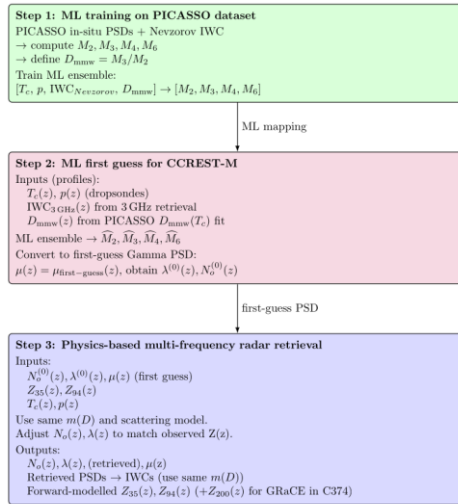
485 Figure 6 A schematic overview of the retrieval framework. Step 1: an ensemble ML model is trained on the PICASSO dataset using in-situ PSDs and the Nevzorov IWC to compute the PSD moments M_2, M_3, M_4 and M_6 and the mean mass-weighted diameter D_{mmw}=M_3/M_2 . Step 2: for each CCREST-M case, profiles of T_c, p , 3 GHz-retrieved IWC and D_{mmw}(T_c) are passed through the ML ensemble to predict the moments, which are converted into first-guess gamma PSD parameters, with \mu(z) =\mu_{first-guess}(z) , where z is the altitude, and corresponding \lambda^{(0)}(z) and N_d^{(0)}(z) . Step 3: a physics-based multi-frequency radar 490 retrieval adjusts N_o(z) and \lambda(z) using the same m(D) and scattering model so that simulated reflectivities Z_{35}(z) and Z_{94}(z) match the observations, yielding retrieved PSD parameters, PSDs and estimated IWCs, and forward-modelled reflectivities.
