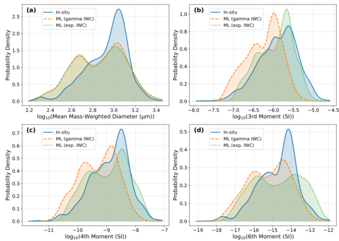
Figure 9 The normalised PDFs of the logarithm (base 10) of the predicted and observed moments for case C374. In-situ size distributions derived from the composite PSDs are shown as solid blue lines and a blue shaded fill. The ML ensemble predictions are presented for the gamma and exponential PSD assumptions used in the retrieval of the 3 GHz IWC. The gamma and exponential PSD assumptions are shown as the orange-dashed line with orange fill, and green-dashed line with green fill, respectively. Comparisons are presented for (a) D_{mmw} , (b) M_3 , (c) M_4 and (d) M_6 . The key is shown in the top-left corner of each panel.
