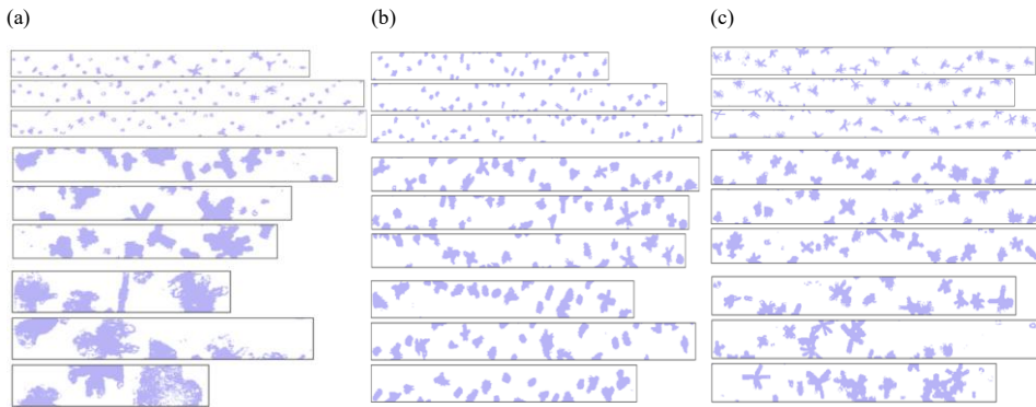
Figure 3 Representative CIP-15 imagery obtained during three distinct altitude levels. In each panel, the top three rectangular strips correspond to cloud top, followed by the next three representing the cloud mid-level, and the bottom three rectangular strips represent the cloud base during descent through the ice layer for cases (a) C374, (b) C379, and (c) C382. Each rectangular strip spans 64 pixels across the CIP-15 array, corresponding to a physical width of 960 \mu\text{m} at 15 \mu\text{m} per pixel. The length of each strip is variable.
