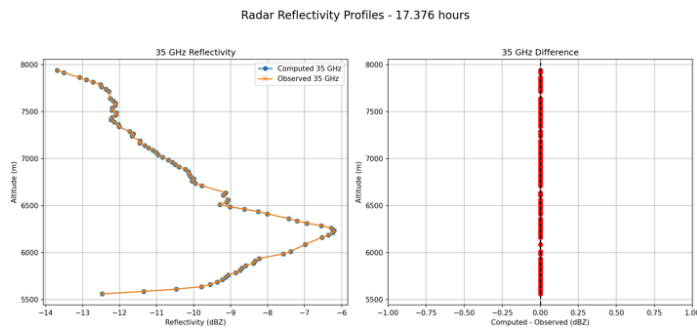
970 Figure 18 As Fig. 12 but for C379 and the 35-GHz radar reflectivity simulations (blue lines) and observations (light brown lines) shown in the left panel and measurement residuals shown in the right panel. The key to the left panel is shown in the top right of the panel.
