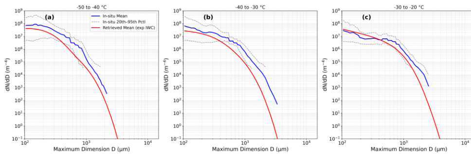
Figure 1720 As Fig. 154 but for C382 and temperature bins of (a) -50 to -40°C, (b) -40 to -30°C, and (c) -30 to -20°C.
