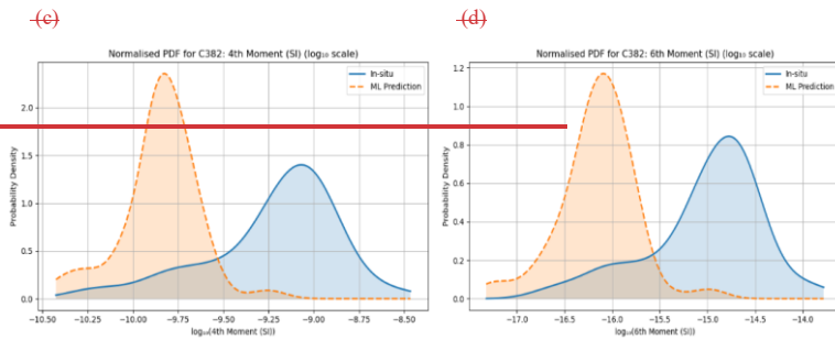
Figure 19 As Fig. 10 but for C382.
