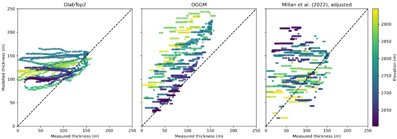
255 Figure 5: Comparison between measured and modelled ice thickness across the GPR-surveyed area, with points coloured by elevation. The dashed line represents 1:1 agreement.
