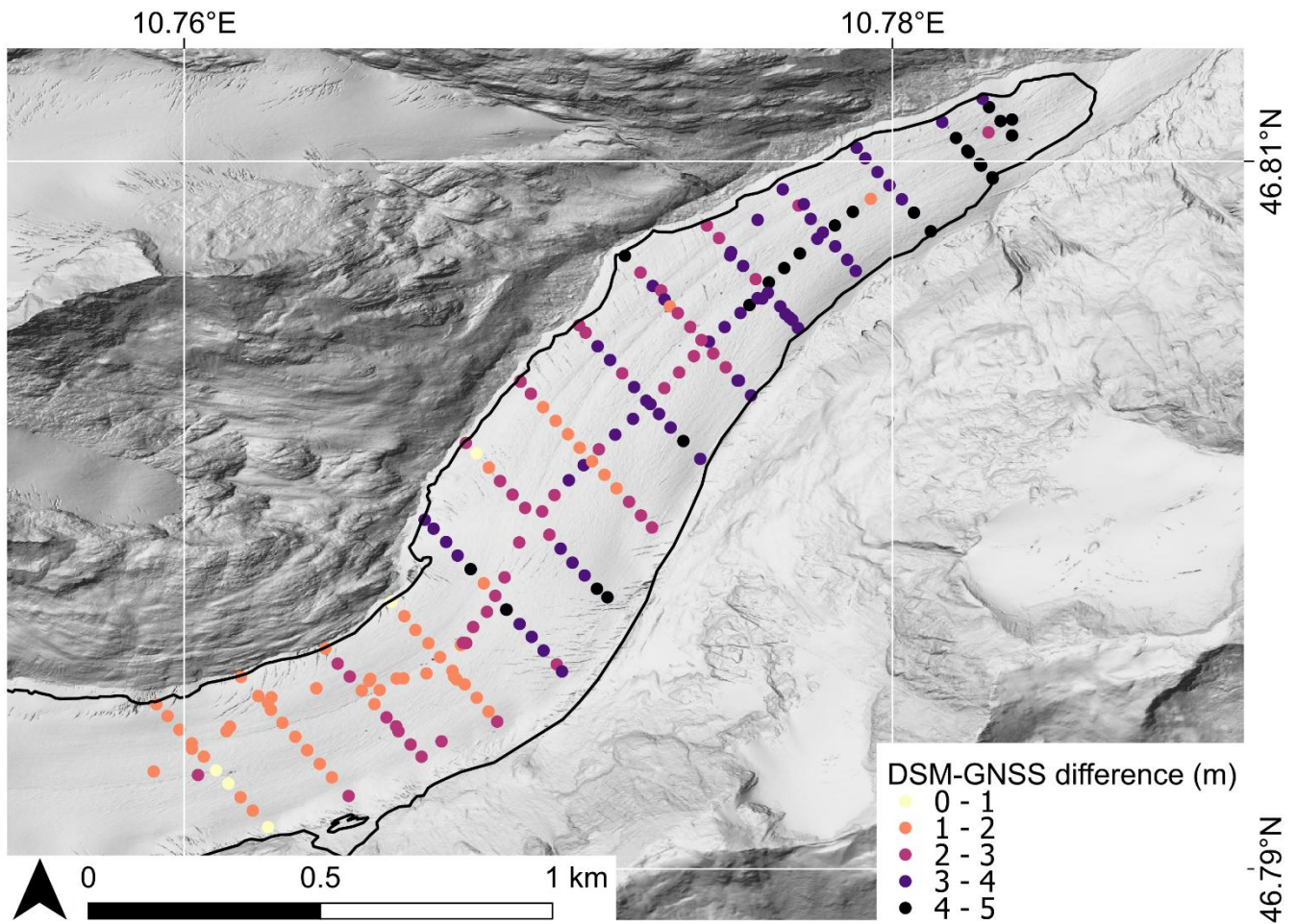
380 Figure A2: Spatial distribution of elevation differences between the 2022 DSM and GNSS-surveyed points (n=193) collected during the August 2023 GPR survey. Differences range from 0.4-4.9 (mean 2.8 \pm 0.9 m , \pm 1\sigma ). Background hillshaded DEM data source: basemap.at (basemap.at, 2024).
