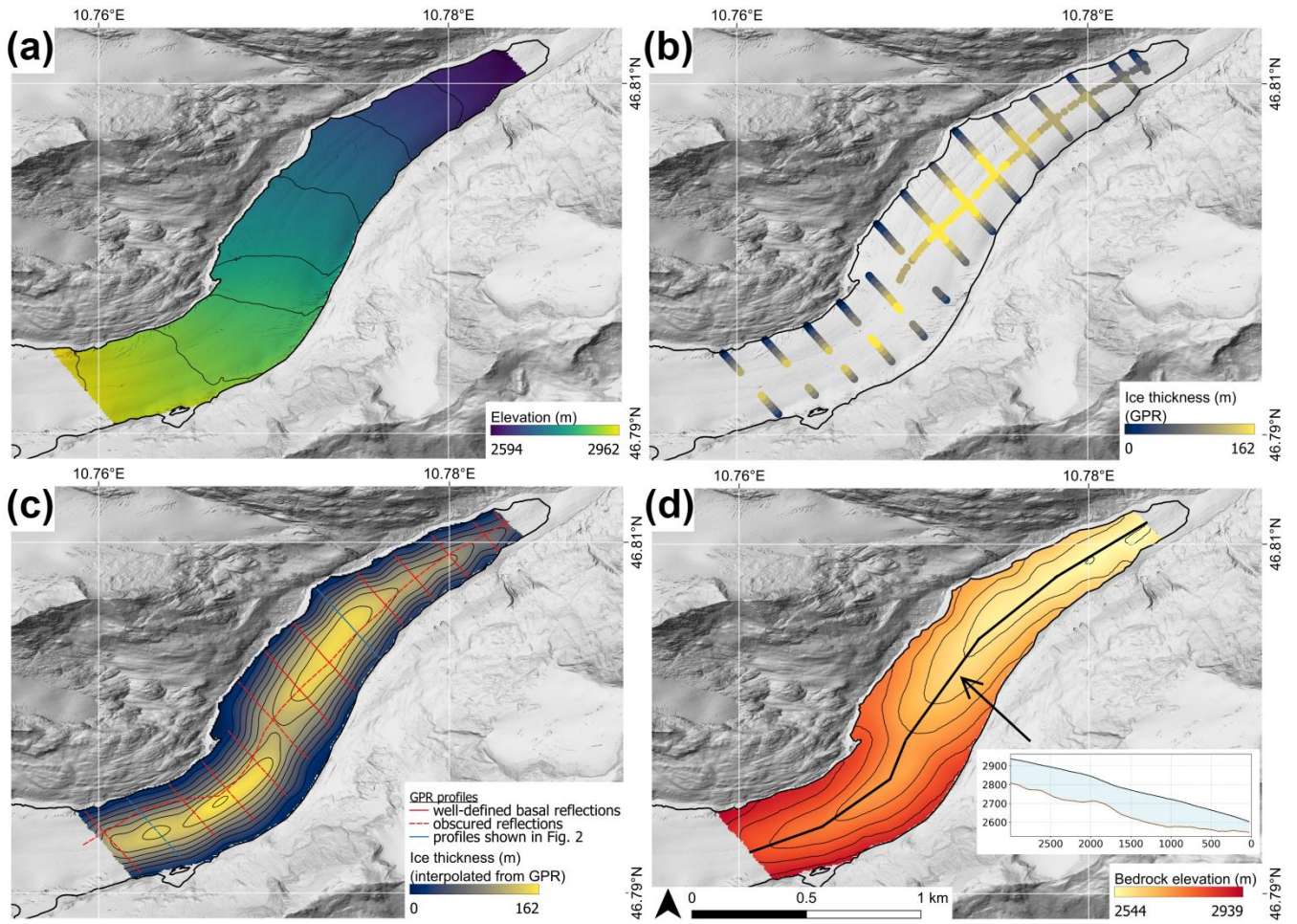
Figure 3: (a) Surface elevation from the 2022 DSM (contour interval 50 m). (b) Measured GPR ice thickness points. (c) Interpolated ice thickness distribution (contour interval 20 m). (d) Bedrock elevation (contour interval 50 m) derived from interpolated GPR data with longitudinal profile along the central flowline (inset). Background hillshaded DEM data source: basemap.at (basemap.at, 2024).
