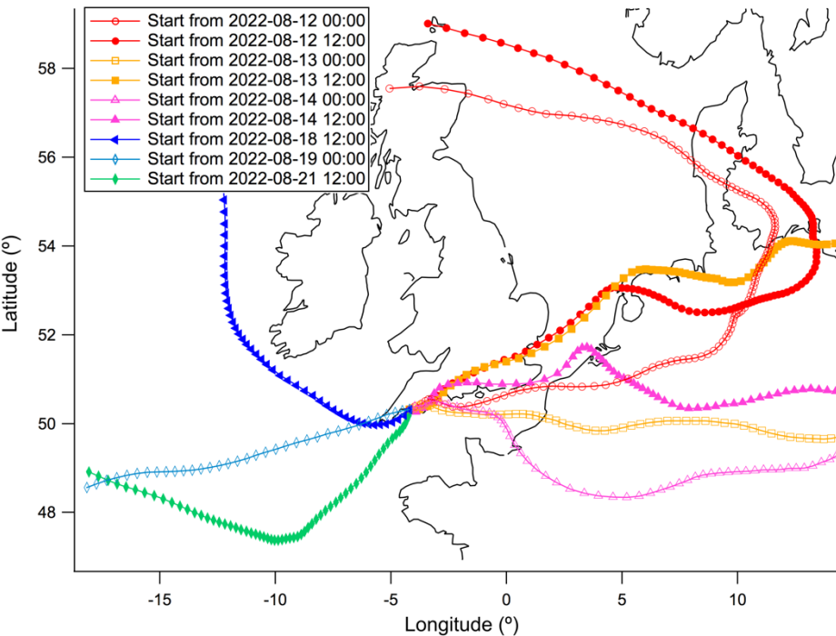
Figure A4. Examples of HYSPLIT back trajectories for selected days in Aug 2022. Even using the high resolution GFS meteorological data (0.25 deg resolution), the trajectories do not well capture the sea breeze events. Trajectories started between 12 and 14 August 2022 only showed the prevailing (night time) northeasterly winds, and did not show the daytime switch to onshore flow. Trajectories started between 18 and 19 August 2022 showed winds mostly from the North Atlantic and did not capture the briefly periods when the winds switched to offshore at night/predawn.
