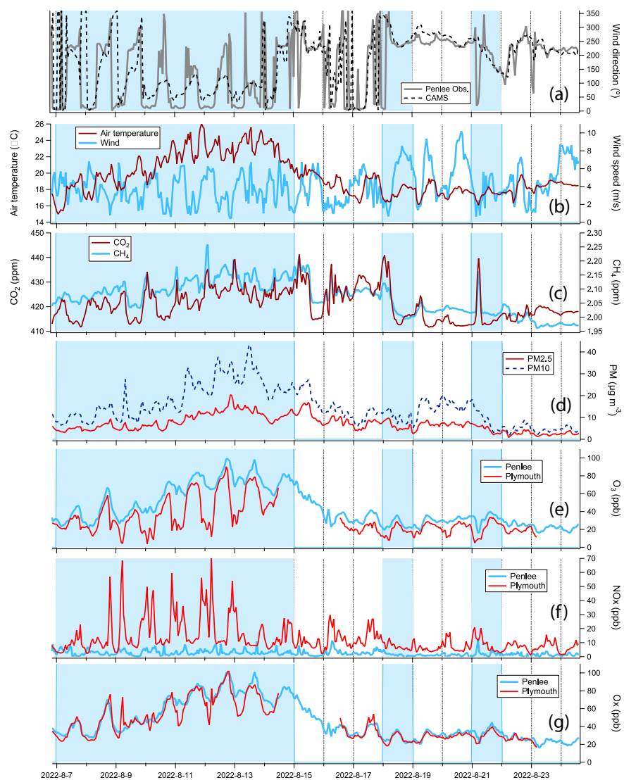
Figure 5. Example of DSB events at PPAO and Plymouth City Centre, with blue shading indicating DSB events. (a) wind direction; (b) air temperature and wind speed from PPAO; (c) CO 2 and CH 4 from PPAO; (d) PM 2.5 and PM 10 from Plymouth; (e) O 3 at PPAO and Plymouth; (f) NO x at PPAO and Plymouth; (g) Ox at PPAO and Plymouth. The ECMWF model forecast wind direction is also shown in panel a.
