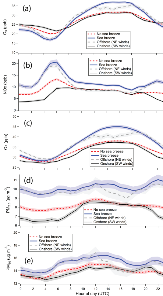
Figure 7. Mean diurnal cycles of (a) O_3 ; (b) NO_x ; (c) Ox ; (d) PM_{2.5} ; (e) PM_{10} with and without sea breeze events in Plymouth City Centre during May, June, and July from 2014 to 2024. Diurnals during offshore wind flow (hourly wind direction from NE) and onshore wind flow (hourly wind direction from SW) are also shown. Shading corresponds to standard error.
