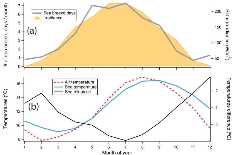
160 Figure 2. Mean annual cycles (2014 – 2024) in (a) DSB events and solar irradiance; (b) air (PPAO), water (L4) temperatures and 165 their difference. DSB events closely track the annual cycle in solar irradiance and correlate negatively with the temperature difference.
