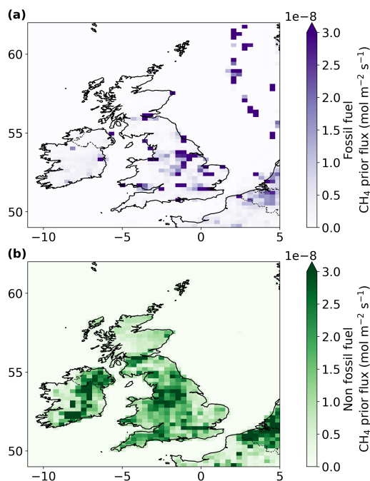
Figure 2. A priori 2023 \text{CH}_4 fluxes from CEH’s UKGHG model and EDGAR, for the (a) FF and (b) non-FF sectors. The FF prior includes fluxes from domestic and industrial combustion and processes, energy production and use and transport. The non-FF prior includes fluxes from enteric fermentation, manure management, waste water treatments, landfills and waste burning.
