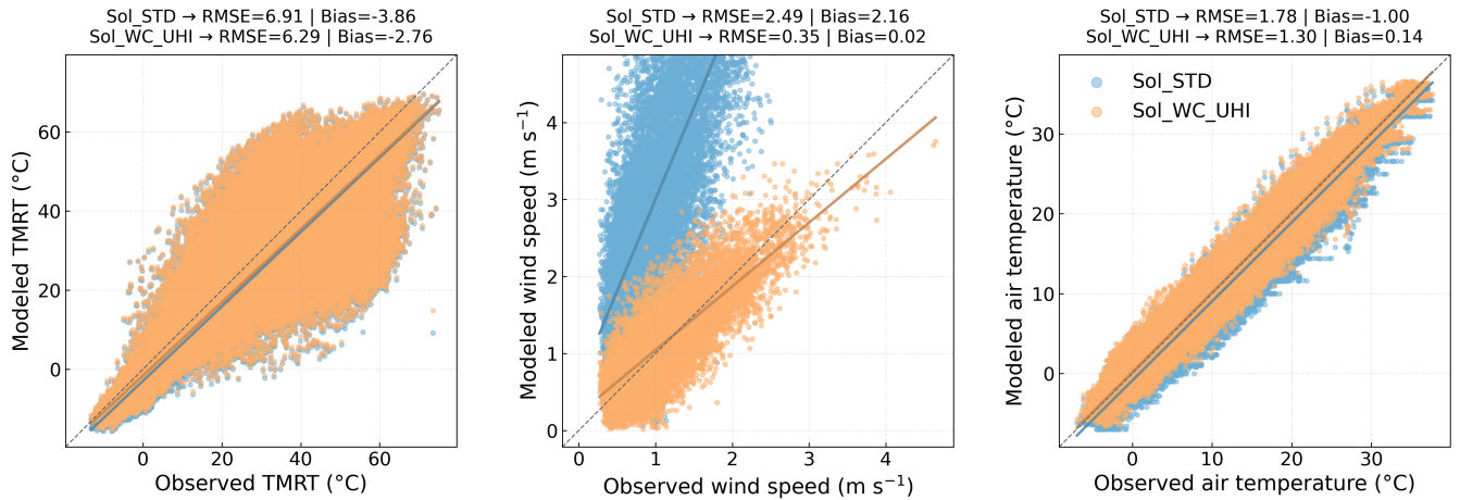
Figure 7. Observed vs. modeled (left) T_{mrt} , (center) canopy wind speed V_{can} , and (right) air temperature for all stations and hours. The baseline run ( Sol_STD ; labeled Sol_STD in the panel titles) shows large wind-speed overestimation and a cold bias in T_a , while the diagnostic wind and UHI corrections in Sol_WC_UHI reduce bias and RMSE, particularly for V_{can} .
