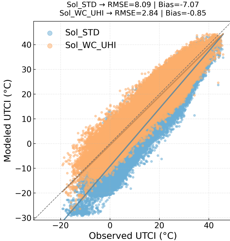
Figure 6. Observed vs. modeled UTCI for all stations and hours. The baseline Sol_STD shows a systematic cold bias, whereas Sol_WC_UHI concentrates closer to the 1:1 line, consistent with improved wind and temperature forcing.
