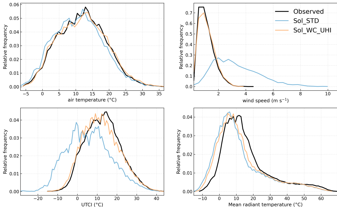
Figure 8. Probability density functions for canopy air temperature, canopy wind speed V_{\text{can}} , UTCI, and T_{\text{mrt}} . Model curves are compared with observations (black). The combined wind and UHI corrections in Sol_WC_UHI suppress the spurious high-wind tail and remove most of the UTCI cold shift present in Sol_STD .
