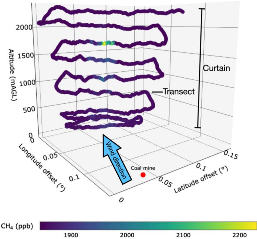
Fig. 3. Three-dimensional visualisation of measured downwind CH 4 enhancements from a flight performed by the in-situ aircraft on 28 September 2023. The red dot marks a quantified coal mine, and the colour bar indicates measured CH 4 mole fractions downwind of the coal mine.
