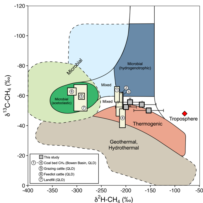
Fig. 9. \delta^{13}\text{C}-\text{CH}_4 vs \delta^2\text{H}-\text{CH}_4 plot after Whiticar (1990) and Haghnegahdar et al. (2023). Coal bed \text{CH}_4 data from the Bowen Basin are from Golding et al. (2013; labelled 1), Hamilton et al. (2020; labelled 2), Kinnon et al. (2010; labelled 3) and Draper and Boreham (2006; labelled 4). \text{CH}_4 isotopic signatures from grazing cattle (labelled 5), feedlot cattle (labelled 6) in Queensland are taken from Lu et al. (2021). \text{CH}_4 isotopic signatures from landfill (labelled 7) are taken from Obersky et al. (2018). Error bars represent the 95% CI bounds on the Keeling plot intercept.
