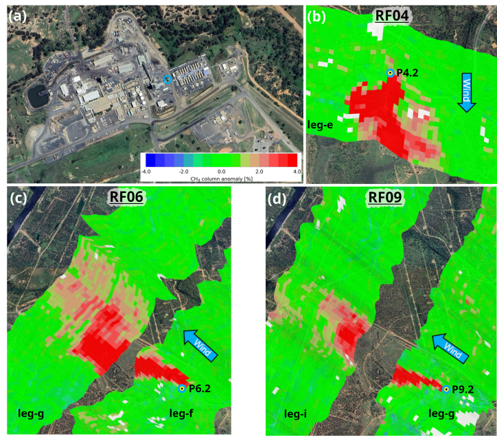
Fig. 4. MAMAP2DL CH 4 column observations over a ventilation shaft (cyan circle). (a) Google Earth imagery showing the shaft location. (b–d) Five of eleven flight legs acquired during research flights on 5, 9, and 16 September 2023, showing downwind CH 4 plume enhancements. Winds were from the north on 5 September and from the south-east on 9 and 16 September. Base map from Google Earth; imagery © 2026 CNES / Airbus.
