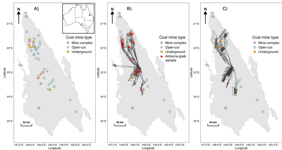
Fig. 1. A) Open-cut, underground and coal mining complexes operational in the Bowen Basin, Australia, during FY24. B) Flight paths (black lines) and the location of airborne grab samples (red dots) for all in-situ aircraft flights. C) Flight paths for all remote sensing aircraft flights. Bowen Basin boundary data © Queensland Government (2025b).
