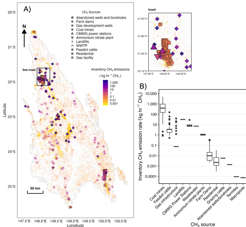
Fig. 2. (A) Location and \text{CH}_4 emission strength of sources within the UNSW inventory across the Bowen Basin, Queensland, Australia. Sources with non-fixed or spatially diffuse locations (e.g. grazing cattle, termites, macropods, and transportation-related emissions) are included in the UNSW inventory but are not spatially represented. The inset (black box) shows a magnified view of an area of dense source overlap. (B) Distribution of \text{CH}_4 emission rates ( \text{kg hr}^{-1} ) for discrete source categories within the UNSW inventory. Gas infrastructure includes coal seam gas and conventional gas facilities and associated infrastructure. Emission rates for grazing cattle are expressed on a per-head basis, whereas feedlot emissions are reported at the facility scale and therefore vary according to feedlot capacity. Further details on source classification and inventory construction are provided in SI-2.
