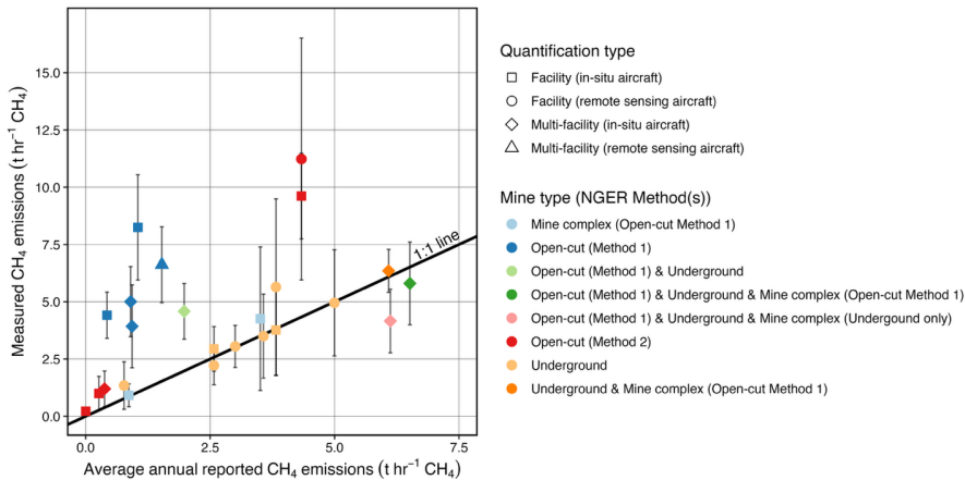
Fig. 5. Comparison between mean airborne emission rates and reported mean annual CH 4 emission rates, distinguished by mine type and NGER method. Each data point represents a mean emission rate ( \pm 2\sigma ) estimate derived from one or more quantifications of a single mine or mine grouping (see Table 1 for full details).
