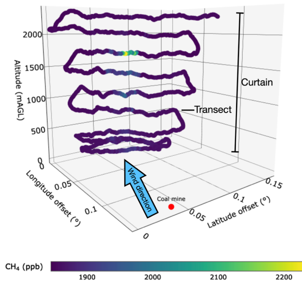
Fig. 3. Three-dimensional visualisation of measured downwind \text{CH}_4 enhancements from a flight performed by the in-situ aircraft on 28 September 2023. The red dot marks a quantified coal mine, and the colour bar indicates measured \text{CH}_4 mole fractions downwind of the coal mine.
