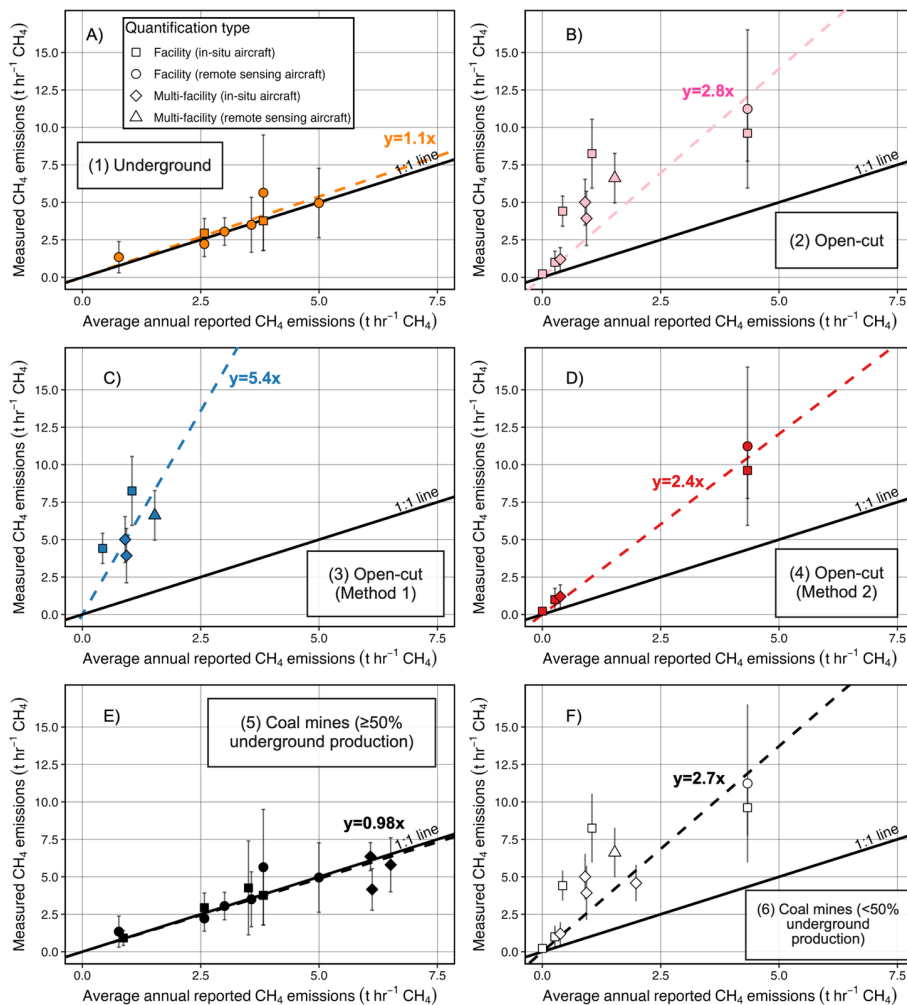
Fig. 7. Comparison between mean airborne emission rates ( \pm 2\sigma ) and reported mean annual \text{CH}_4 emission rates for: A) exclusively underground coal mines; B) exclusively open-cut coal mines; C) exclusively open-cut coal mines estimated using Method 1; D) exclusively open-cut coal mines estimated using Method 2; E) coal mines with \geq 50\% underground production; and F) coal mines with < 50\% underground production. The fixed-origin linear regression analysis model is indicated by the dashed line and the slope is indicated in each panel. Symbol shapes are as in Figs. 5 and 6.
